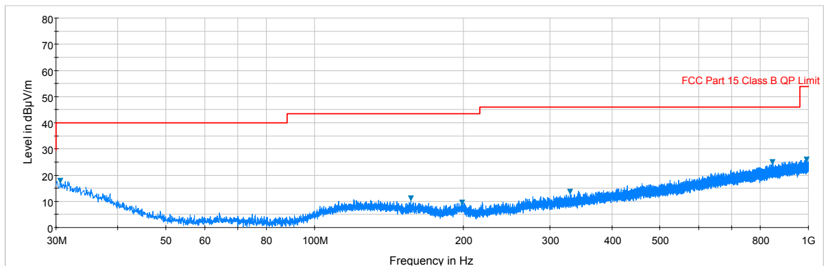
Plot 7-96. Radiated Spurious Plot below 1GHz (Pol. V)
