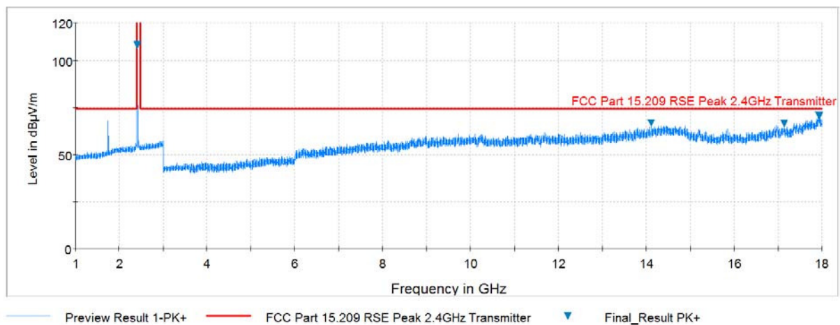
Plot 7-70. Radiated Spurious Plot above 1GHz (802.11b – Ch. 1, Ant. Pol. V)
