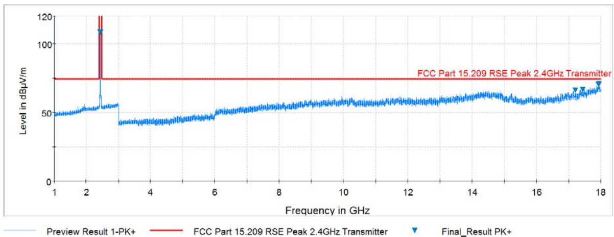
Plot 7-64. Radiated Spurious Plot above 1GHz (802.11b – Ch. 6, Ant. Pol. V)
