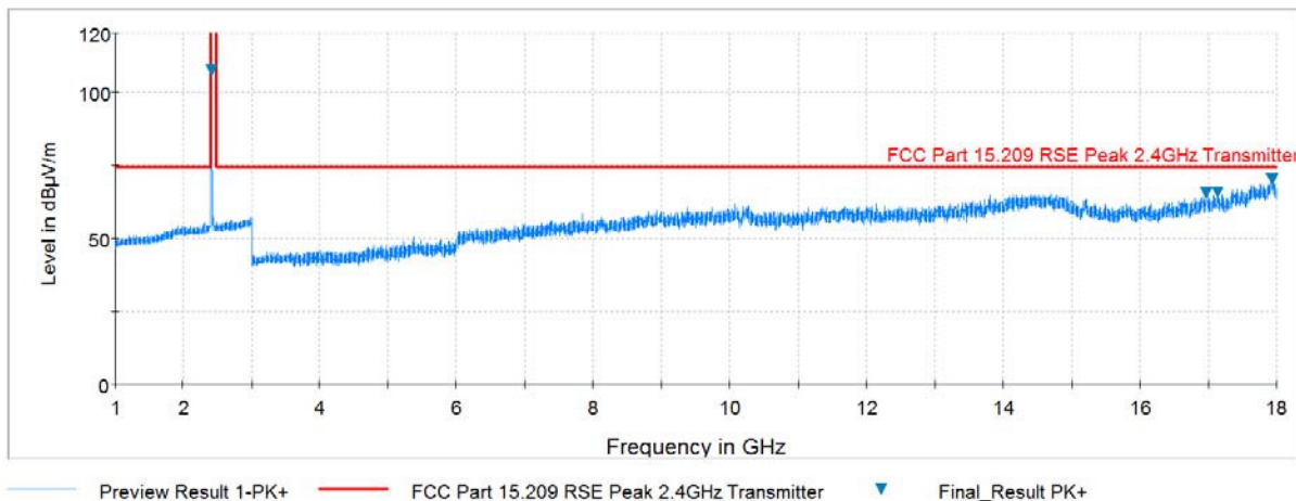
Plot 7-61. Radiated Spurious Plot above 1GHz (802.11b – Ch. 1, Ant. Pol. H)
