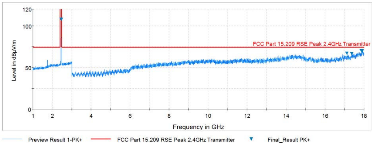
Plot 7-66. Radiated Spurious Plot above 1GHz (802.11b – Ch. 11, Ant. Pol. V)
