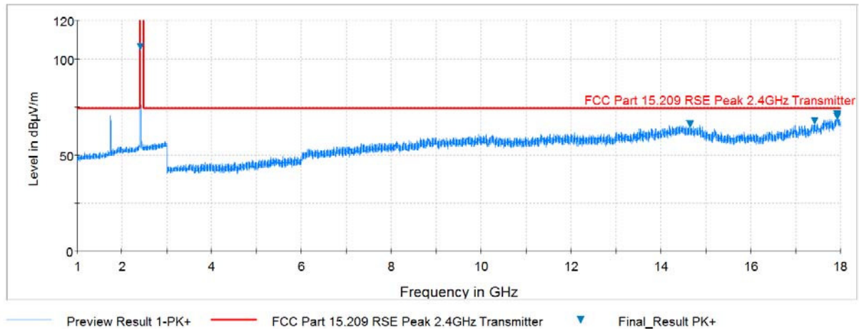
Plot 7-69. Radiated Spurious Plot above 1GHz (802.11b – Ch. 1, Ant. Pol. H)
