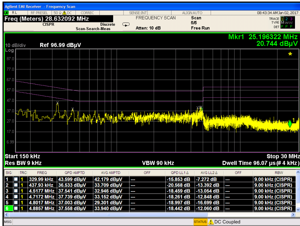
Plot 7-99. Line Conducted Plot with 802.11b (L)
