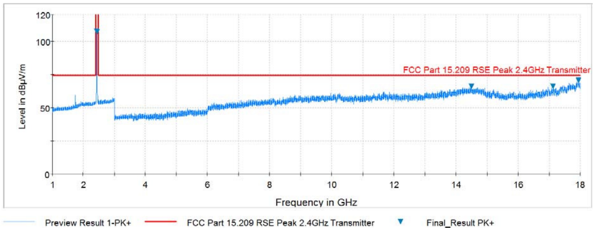
Plot 7-72. Radiated Spurious Plot above 1GHz (802.11b – Ch. 6, Ant. Pol. V)
