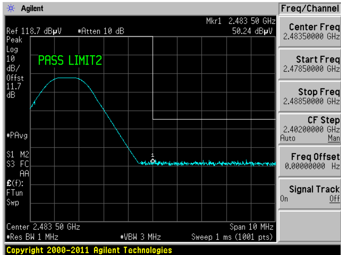
Plot 6-19. Radiated Upper Restricted Band Edge Plot (Peak)
