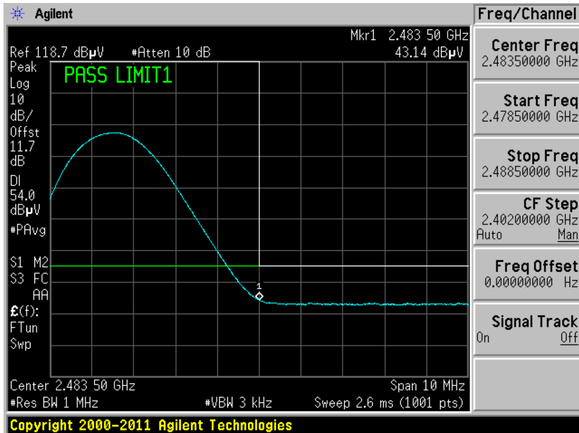
Plot 6-18. Radiated Upper Restricted Band Edge Plot (Average)
