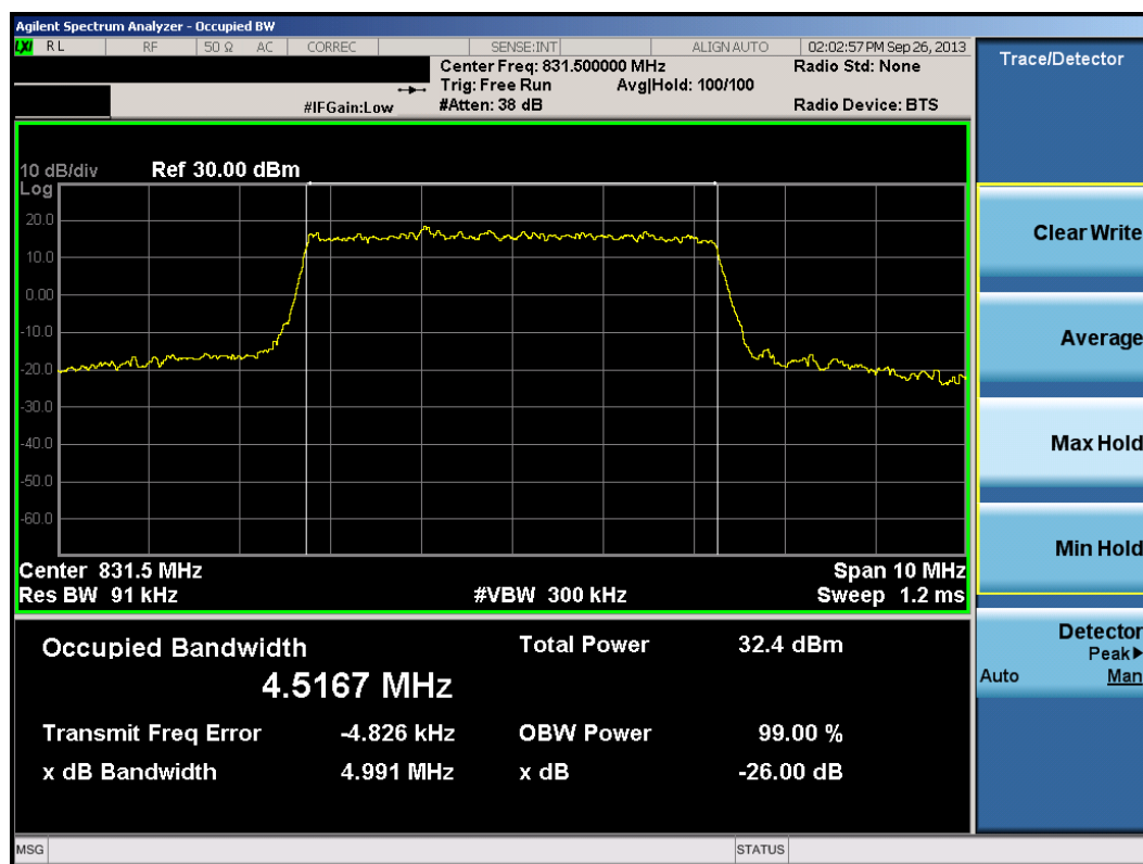
Plot 7-16. Occupied Bandwidth Plot (5.0MHz QPSK – RB Size 25)
