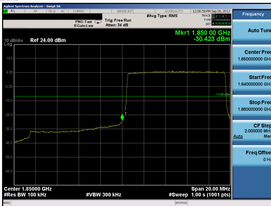
Plot 8-23. Lower Band Edge Plot (10.0MHz QPSK – RB Size 50)
