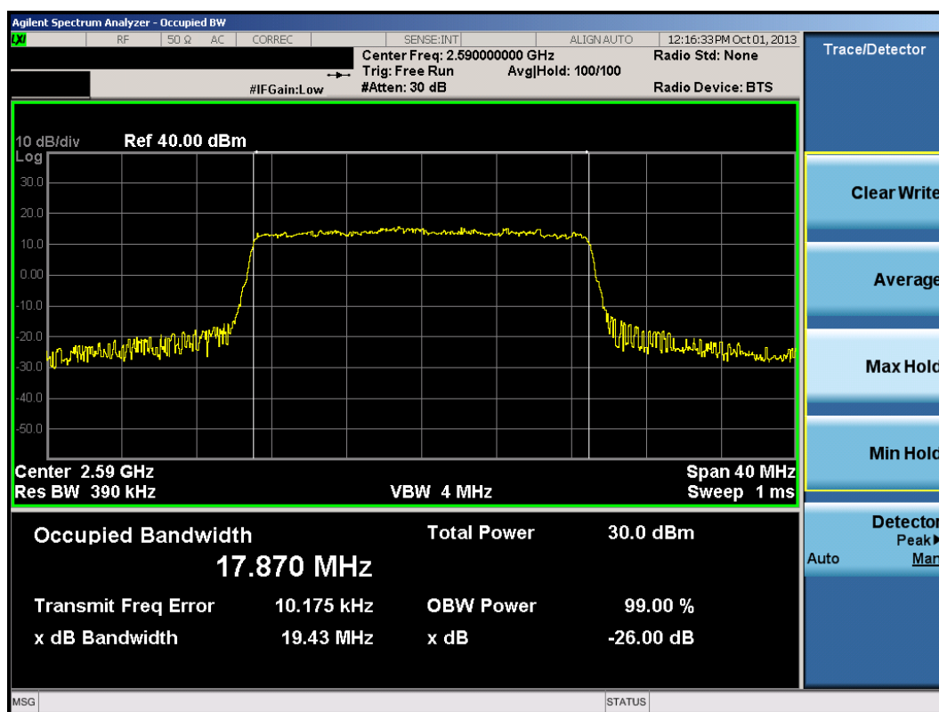
Plot 9-24. Occupied Bandwidth Plot (20.0MHz 16-QAM – RB Size 100)
