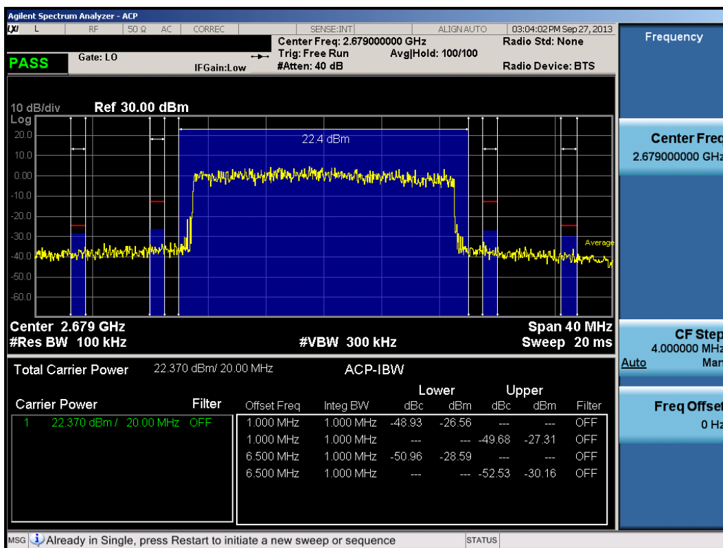
Plot 9-22. High Adjacent Channel Band Edge Plot (20.0MHz QPSK – RB Size 100)
