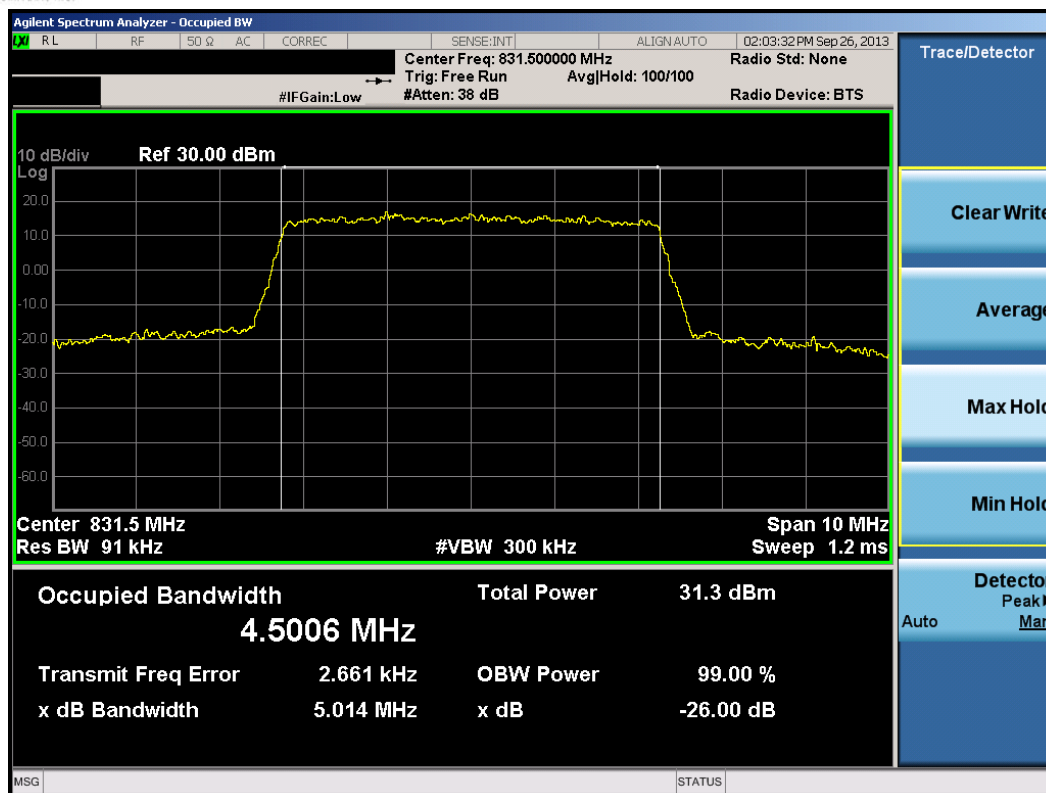
Plot 7-17. Occupied Bandwidth Plot (5.0MHz 16-QAM – RB Size 25)
