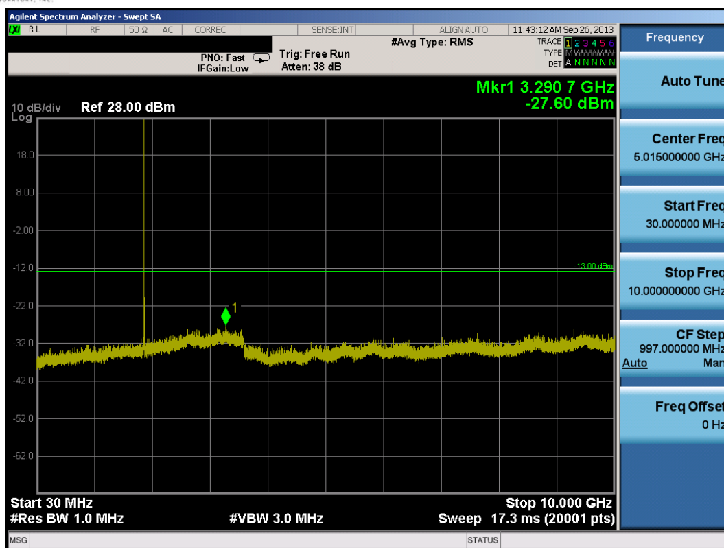
Plot 8-15. Conducted Spurious Plot (5.0MHz QPSK – RB Size 1, RB Offset 0 – Mid Channel)
