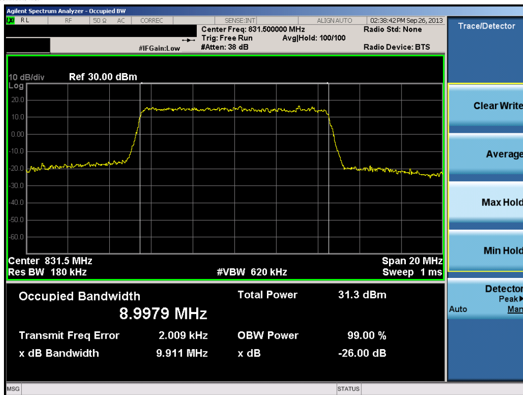
Plot 7-21. Occupied Bandwidth Plot (10.0MHz 16-QAM – RB Size 50)
