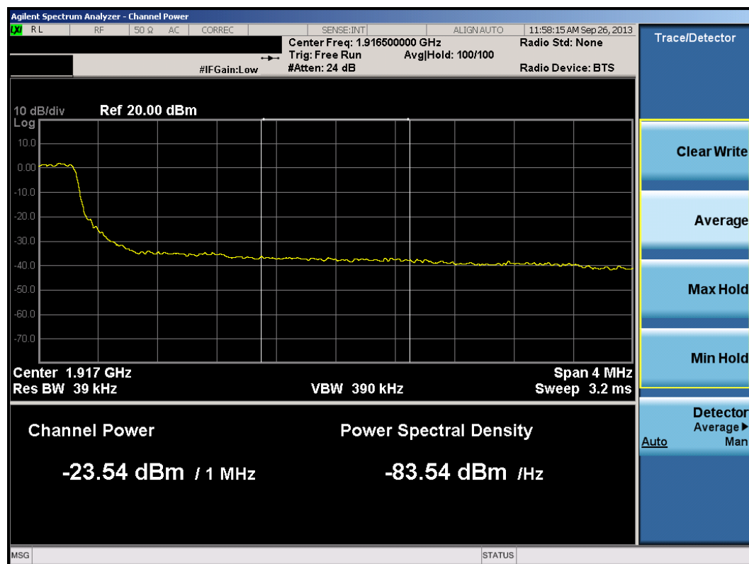
Plot 8-20. Upper Extended Band Edge Plot (5.0MHz QPSK – RB Size 25)
