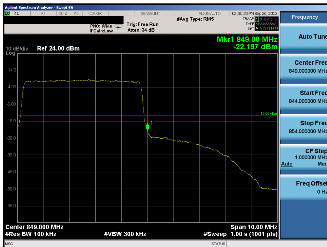
Plot 7-18. Upper Band Edge Plot (5.0MHz QPSK – RB Size 25)
