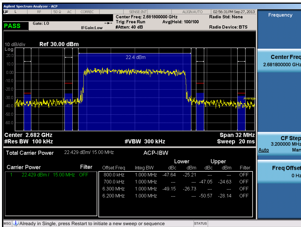
Plot 9-17. High Adjacent Channel Band Edge Plot (15.0MHz QPSK – RB Size 75)
