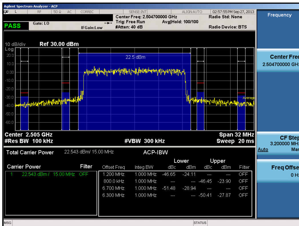
Plot 9-15. Low Adjacent Channel Band Edge Plot (15.0MHz QPSK – RB Size 75)
