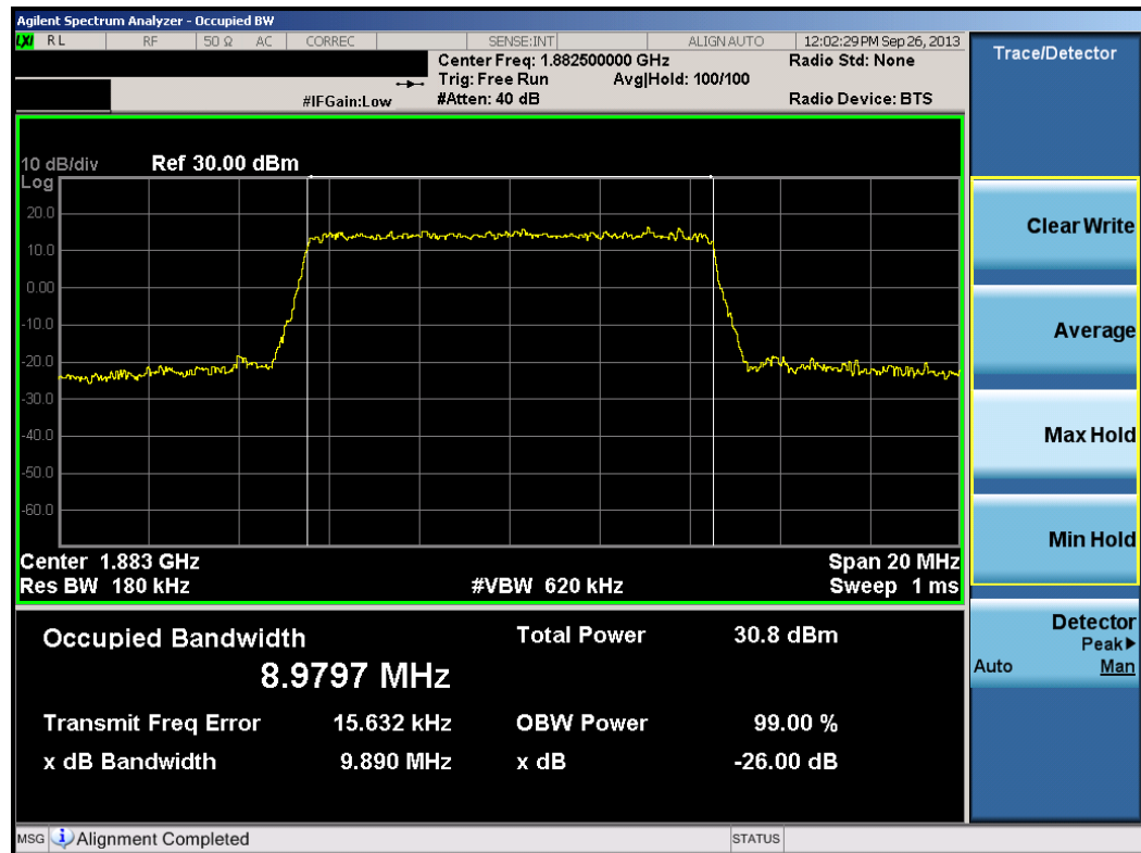
Plot 8-26. Occupied Bandwidth Plot (10.0MHz 16-QAM – RB Size 50)
