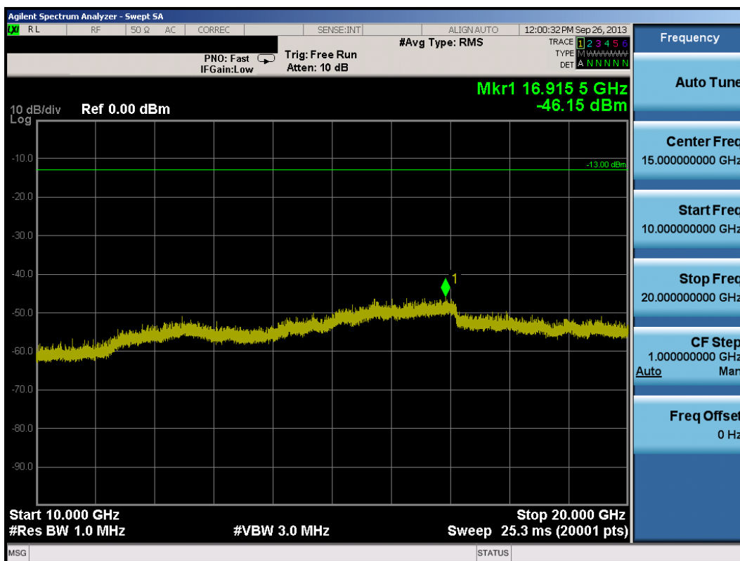
Plot 8-18. Conducted Spurious Plot (5.0MHz QPSK – RB Size 1, RB Offset 0 – High Channel)
