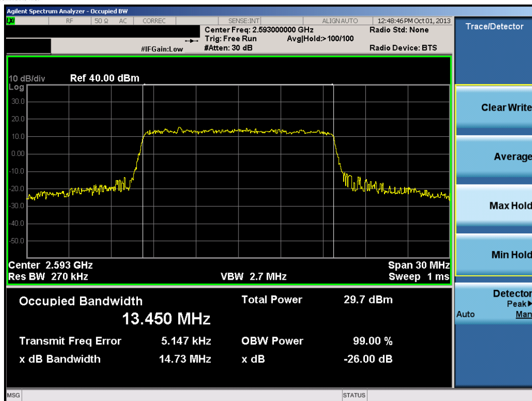
Plot 9-19. Occupied Bandwidth Plot (15.0MHz 16-QAM – RB Size 75)
