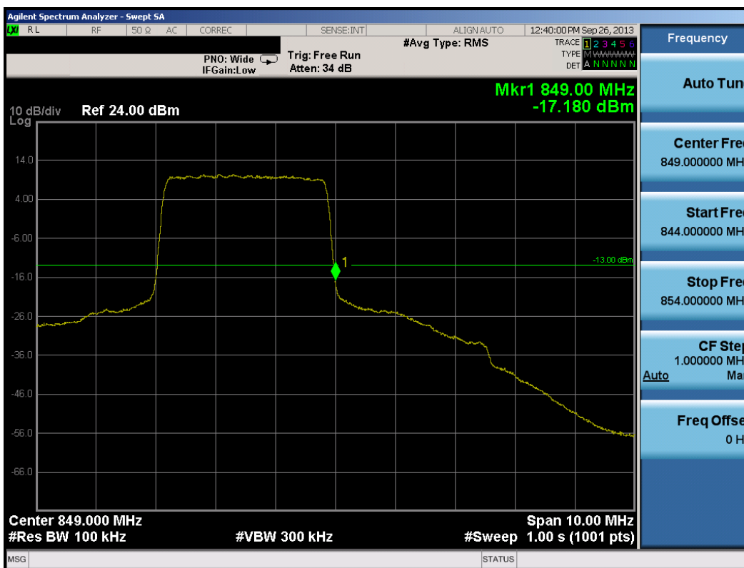
Plot 7-14. Upper Band Edge Plot (3.0MHz QPSK – RB Size 15)
