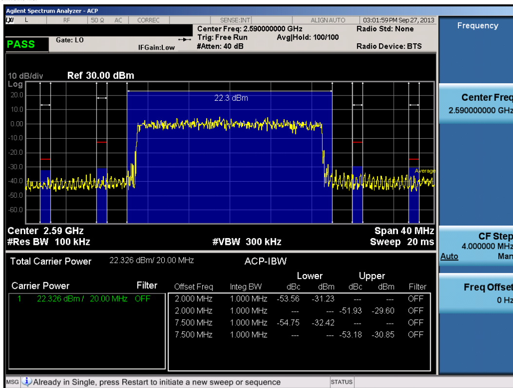
Plot 9-21. Mid Adjacent Channel Band Edge Plot (20.0MHz QPSK – RB Size 100)
