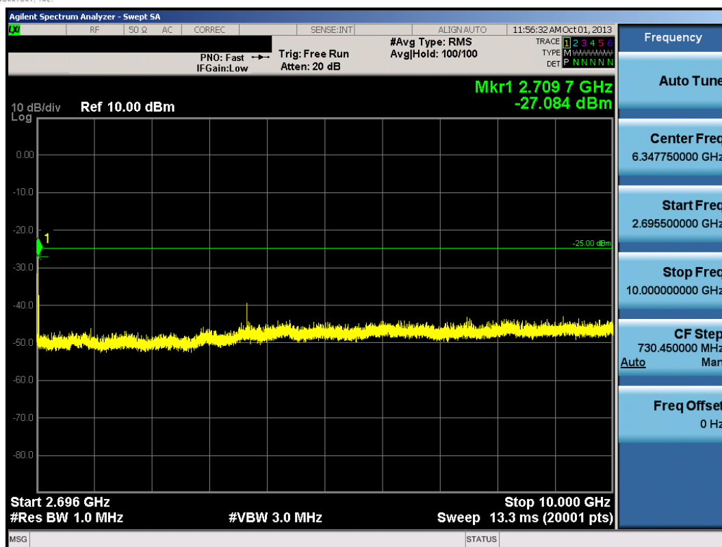
Plot 9-13. Conducted Spurious Plot (10.0MHz QPSK – RB Size 1, RB Offset 0 – High Channel)
