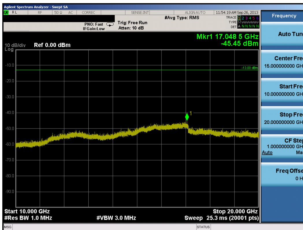
Plot 8-14. Conducted Spurious Plot (5.0MHz QPSK – RB Size 1, RB Offset 0 – Low Channel)
