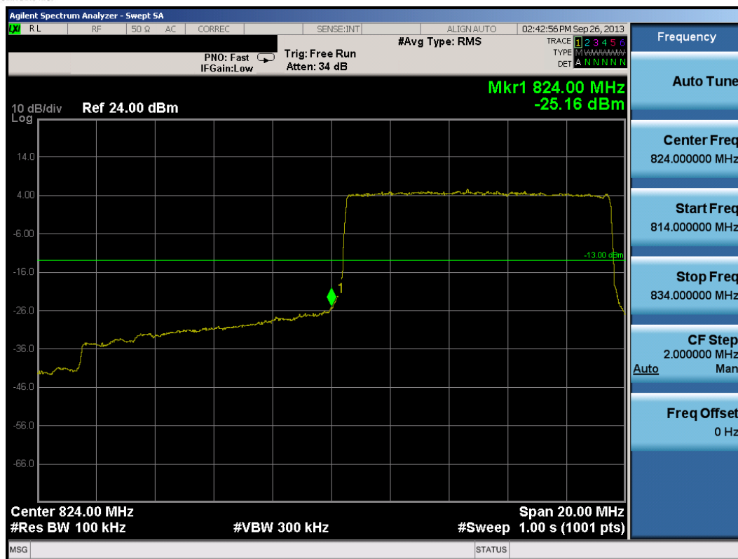
Plot 7-19. Lower Band Edge Plot (10.0MHz QPSK – RB Size 50)
