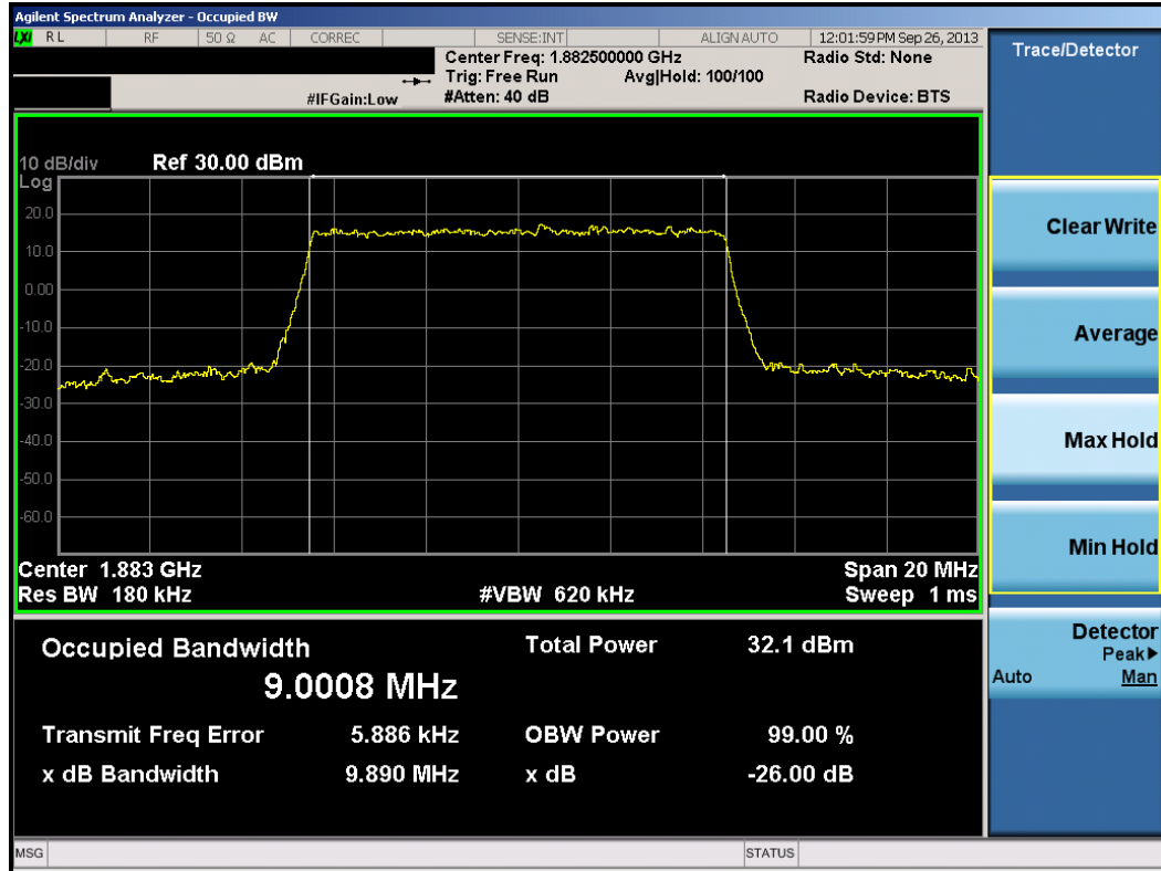
Plot 8-25. Occupied Bandwidth Plot (10.0MHz QPSK – RB Size 50)
