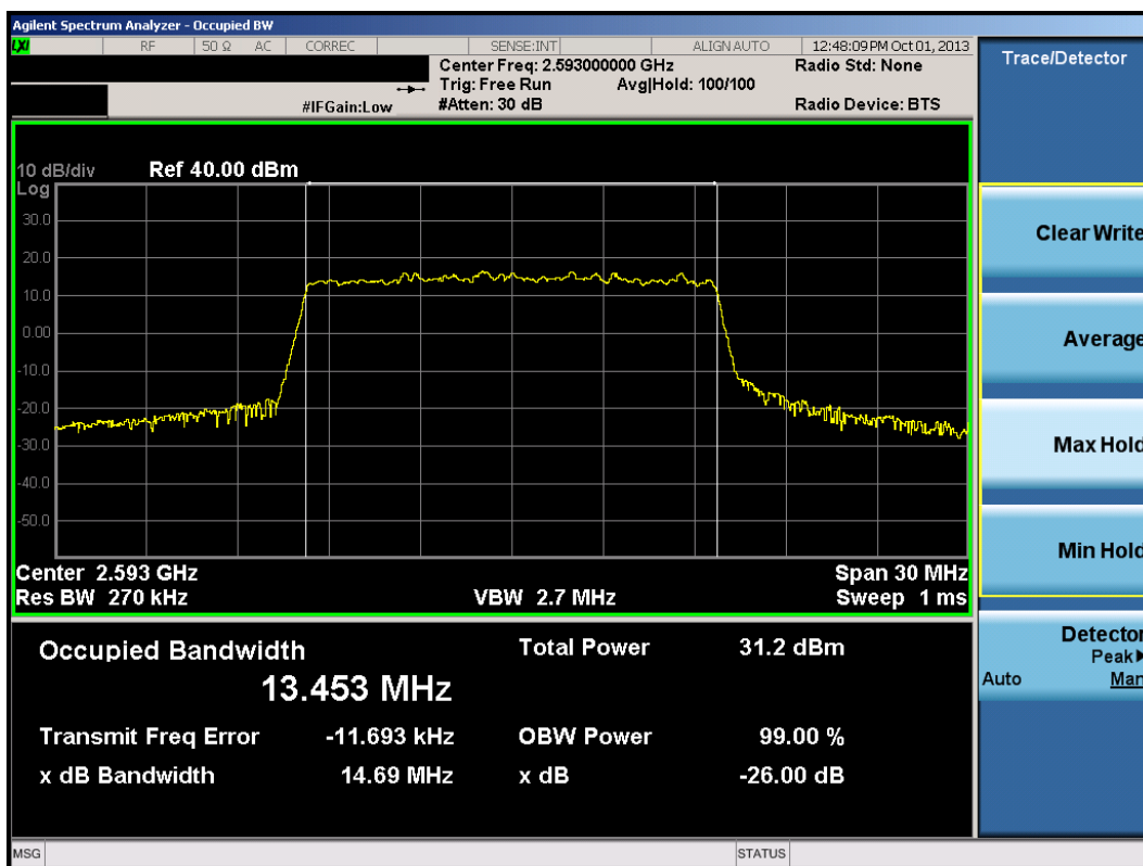
Plot 9-18. Occupied Bandwidth Plot (15.0MHz QPSK – RB Size 75)
