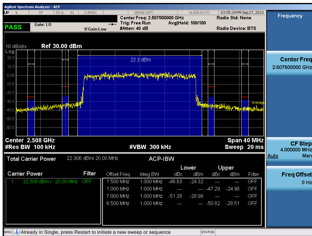
Plot 9-20. Low Adjacent Channel Band Edge Plot (20.0MHz QPSK – RB Size 100)
