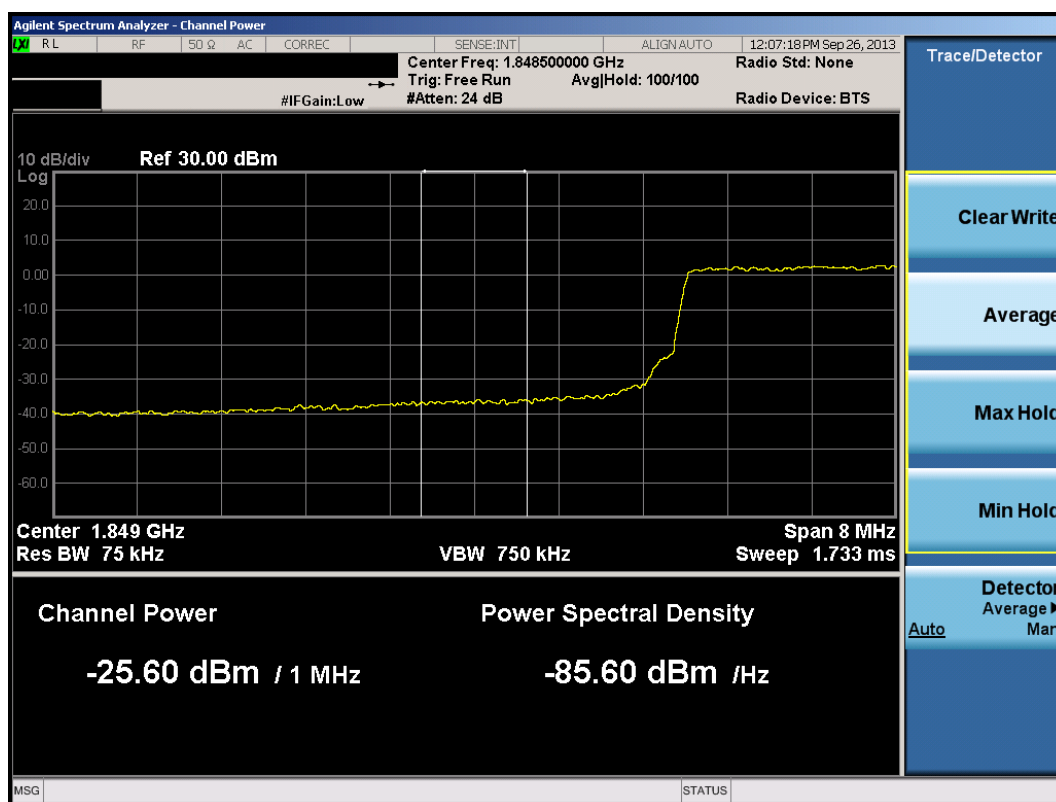
Plot 8-24. Lower Extended Band Edge Plot (10.0MHz QPSK – RB Size 50)
