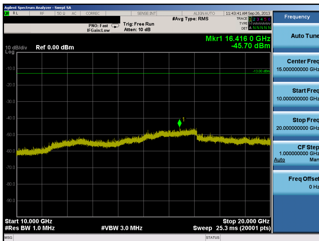
Plot 8-16. Conducted Spurious Plot (5.0MHz QPSK – RB Size 1, RB Offset 0 – Mid Channel)
