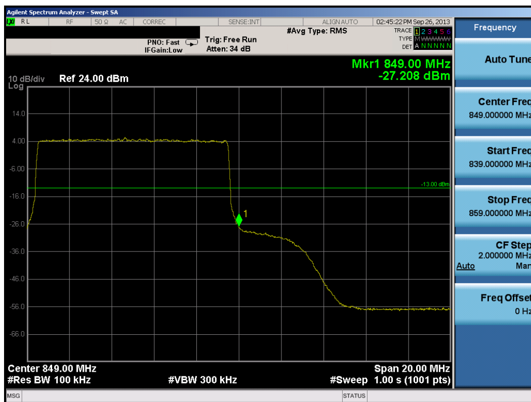
Plot 7-22. Upper Band Edge Plot (10.0MHz QPSK – RB Size 50)
