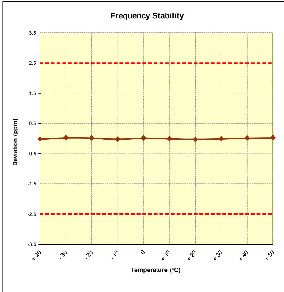
Figure 6-1. CDMA BC10 Frequency Stability Graph (Ch. 670)
