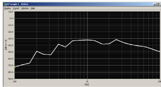
Figure 7-3 Worst-case ABM2 Plot for WD, GSM
