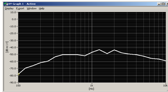
Figure 7-2 Worst-case ABM2 Plot for WD, CDMA
