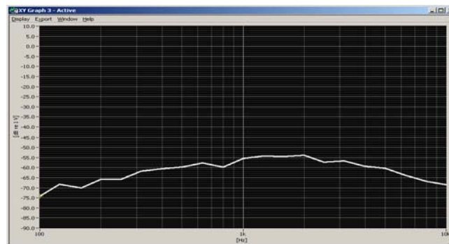
Figure 7-4 Worst-case ABM2 Plot for WD, UMTS
