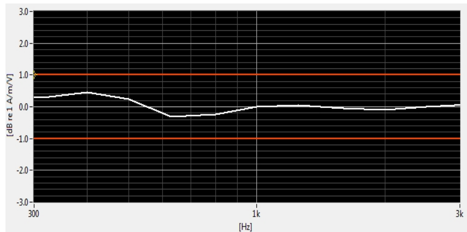
Figure 7-3 Helmholtz Coil Validation for Frequency Response
