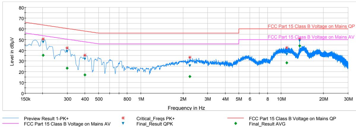
Plot 8-1. Line-Conducted Test Plot (L1)
