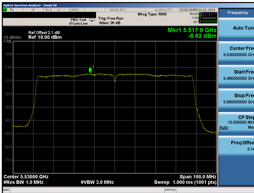
Plot 6-66. Peak Power Spectral Density Plot (80MHz BW 802.11ac (UNII Band 2C) – Ch. 106)
