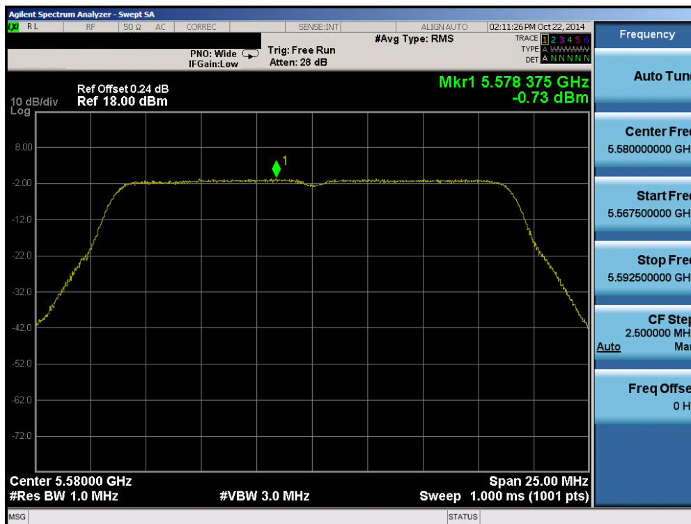
Plot 6-61. Peak Power Spectral Density Plot (20MHz BW 802.11n (UNII Band 2C) – Ch. 116)
