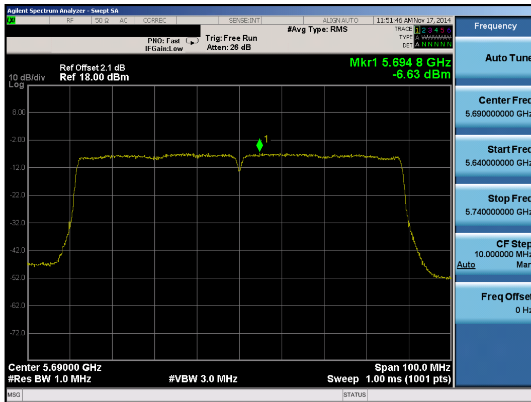
Plot 6-67. Peak Power Spectral Density Plot (80MHz BW 802.11ac (UNII Band 2C) – Ch. 138)
