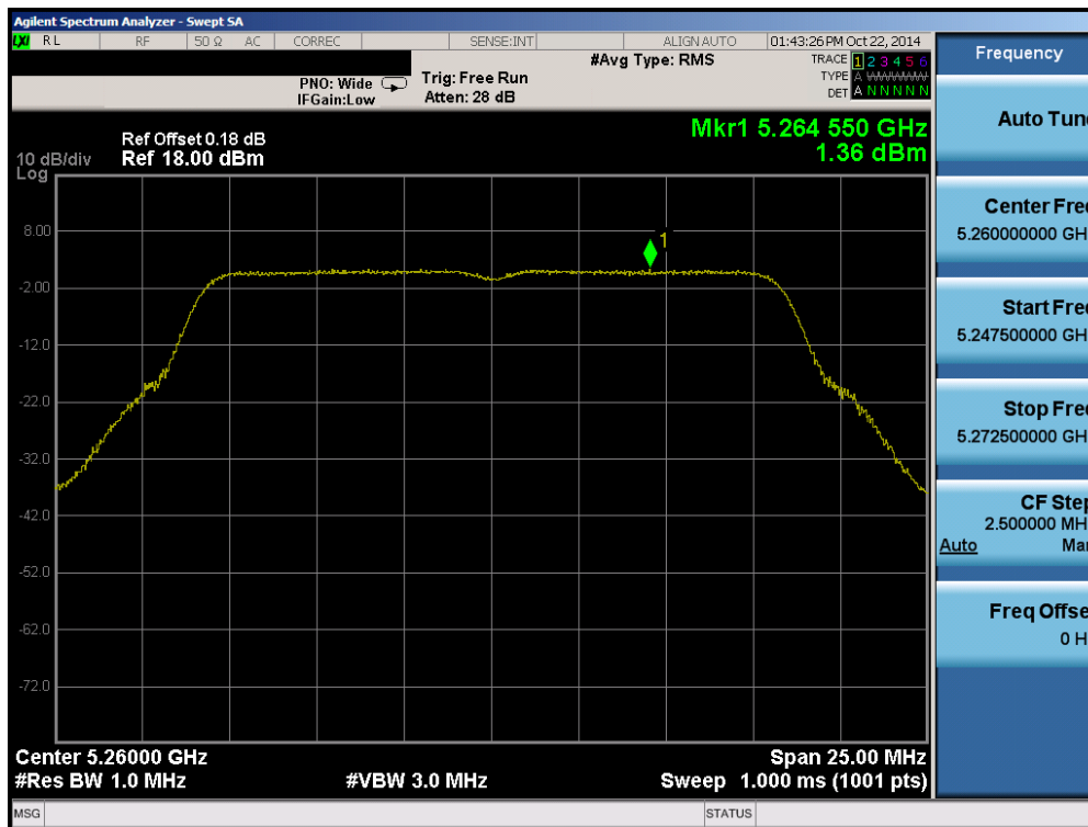
Plot 6-48. Peak Power Spectral Density Plot (802.11a (UNII Band 2A) – Ch. 52)
