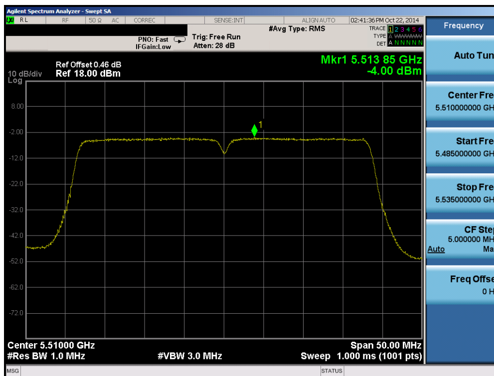
Plot 6-63. Peak Power Spectral Density Plot (40MHz BW 802.11n (UNII Band 2C) – Ch. 102)
