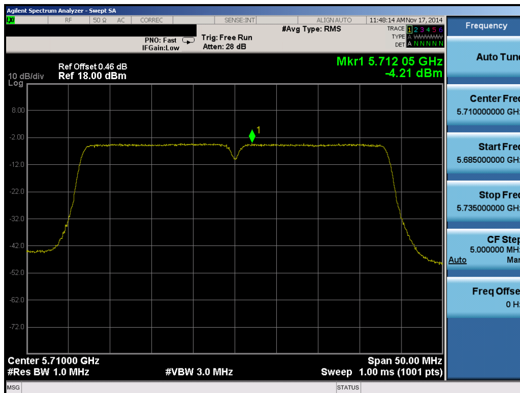
Plot 6-65. Peak Power Spectral Density Plot (40MHz BW 802.11n (UNII Band 2C) – Ch. 142)
