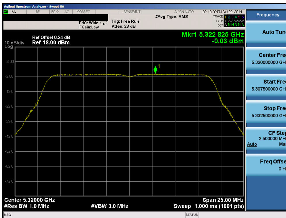
Plot 6-53. Peak Power Spectral Density Plot (20MHz BW 802.11n (UNII Band 2A) – Ch. 64)
