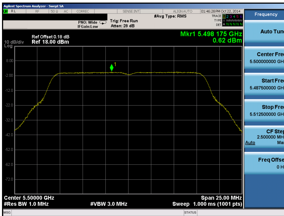
Plot 6-57. Peak Power Spectral Density Plot (802.11a (UNII Band 2C) – Ch. 100)
