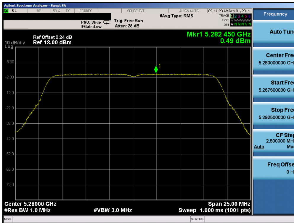
Plot 6-52. Peak Power Spectral Density Plot (20MHz BW 802.11n (UNII Band 2A) – Ch. 56)
