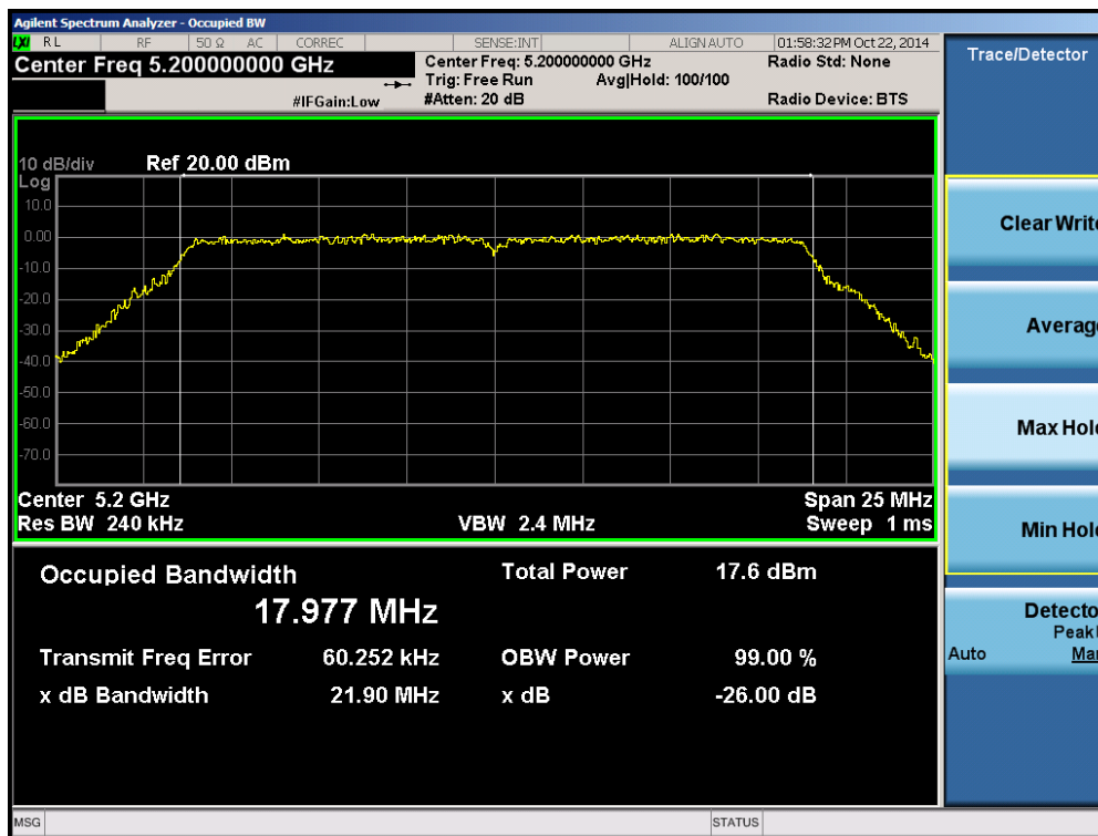
Plot 6-5. 26dB Bandwidth Plot (20MHz BW 802.11n (UNII Band 1) – Ch. 40)
