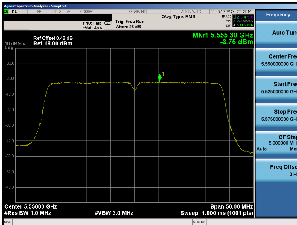
Plot 6-64. Peak Power Spectral Density Plot (40MHz BW 802.11n (UNII Band 2C) – Ch. 110)
