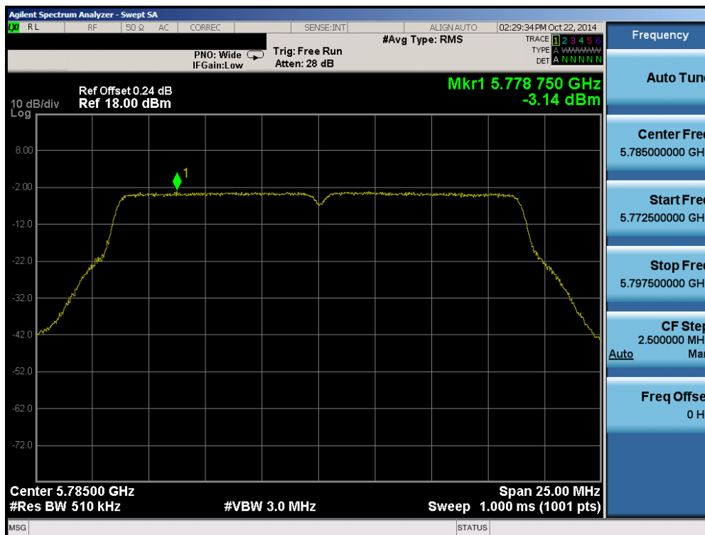
Plot 6-72. Peak Power Spectral Density Plot (20MHz BW 802.11n (UNII Band 3) – Ch. 157)
