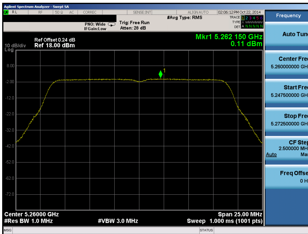
Plot 6-51. Peak Power Spectral Density Plot (20MHz BW 802.11n (UNII Band 2A) – Ch. 52)
