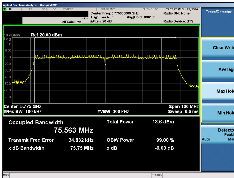
Plot 6-38. 6dB Bandwidth Plot (80MHz BW 802.11ac (UNII Band 3) – Ch. 155)
