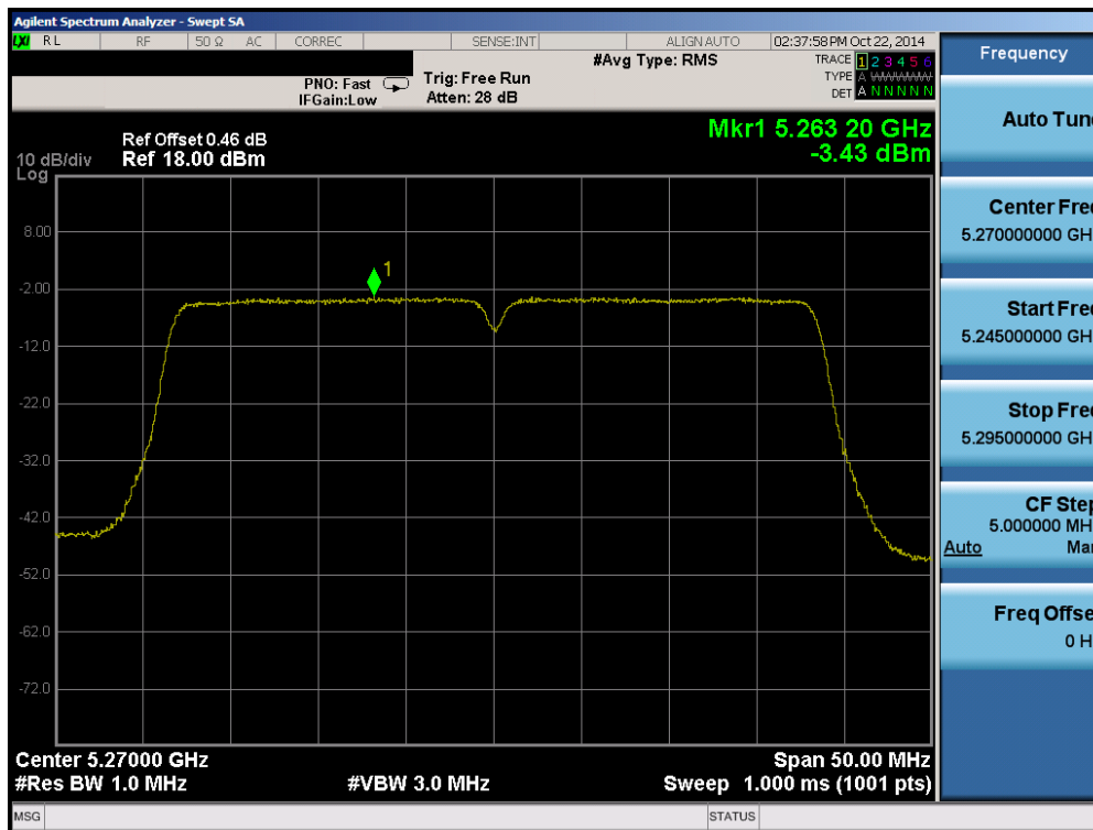
Plot 6-54. Peak Power Spectral Density Plot (40MHz BW 802.11n (UNII Band 2A) – Ch. 54)
