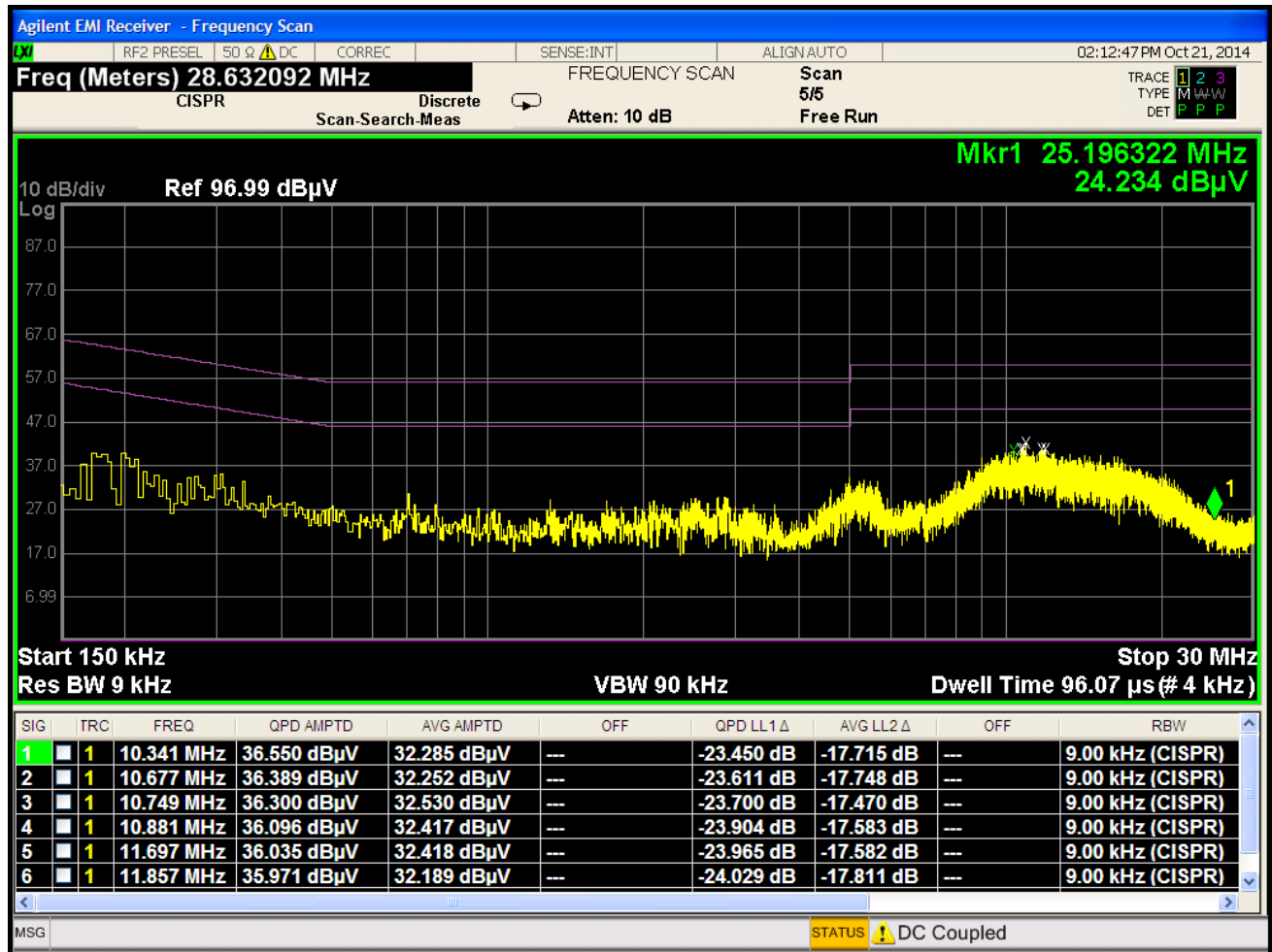
Plot 6-100. Line Conducted Plot with 802.11a UNII Band 1 (L1)
