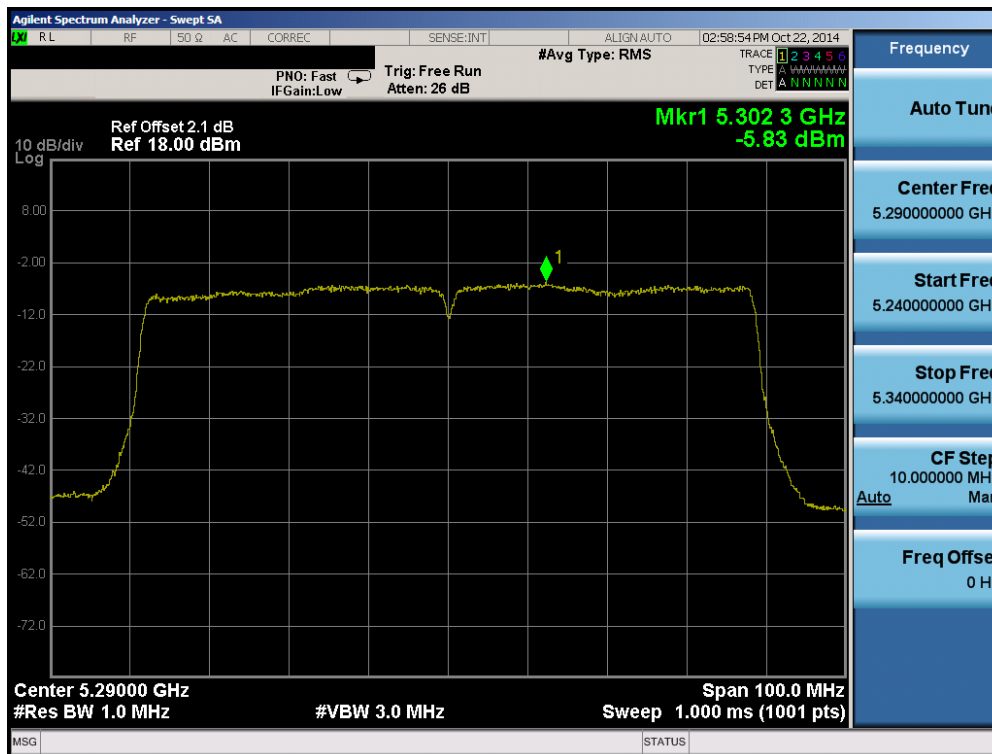
Plot 6-56. Peak Power Spectral Density Plot (80MHz BW 802.11ac (UNII Band 2A) – Ch. 58)
