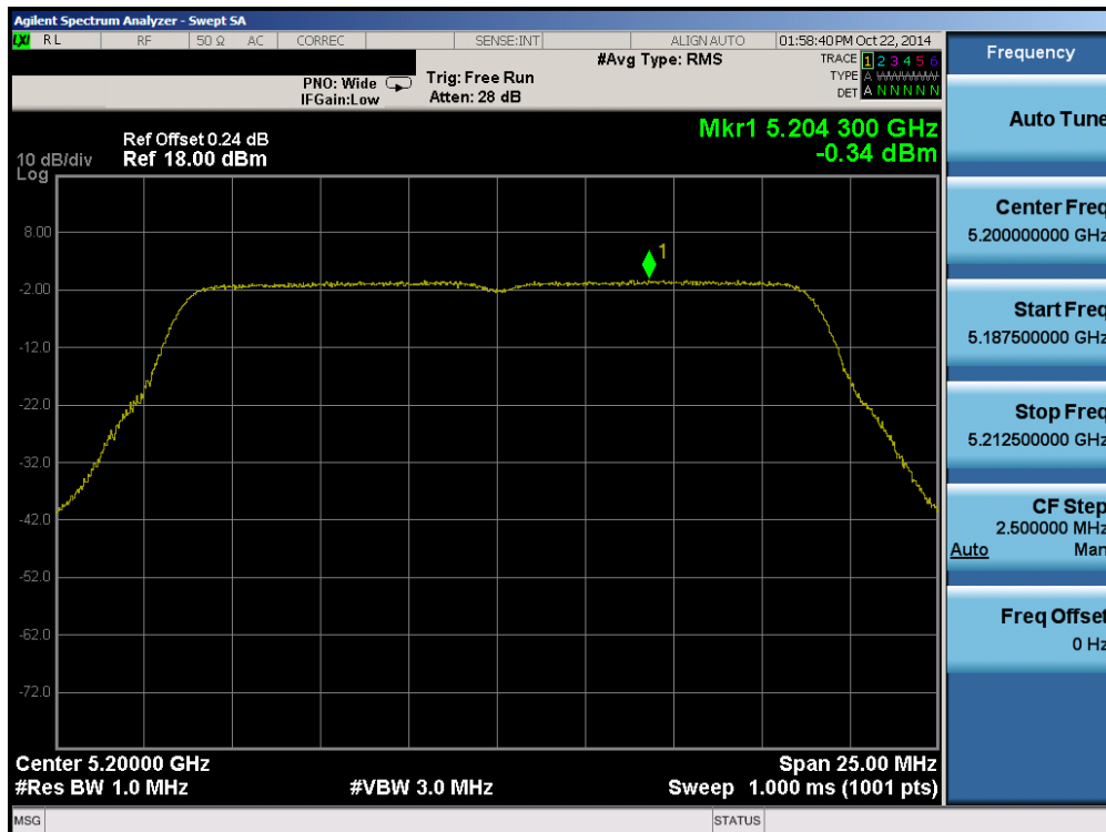
Plot 6-43. Peak Power Spectral Density Plot (20MHz BW 802.11n (UNII Band 1) – Ch. 40)
