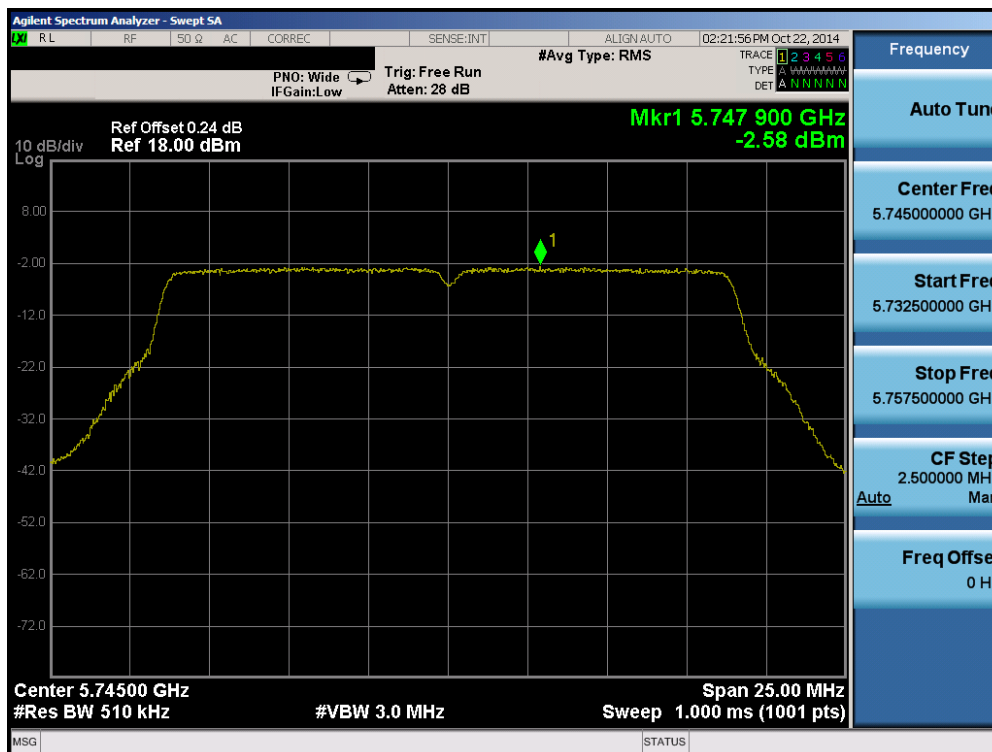
Plot 6-71. Peak Power Spectral Density Plot (20MHz BW 802.11n (UNII Band 3) – Ch. 149)
