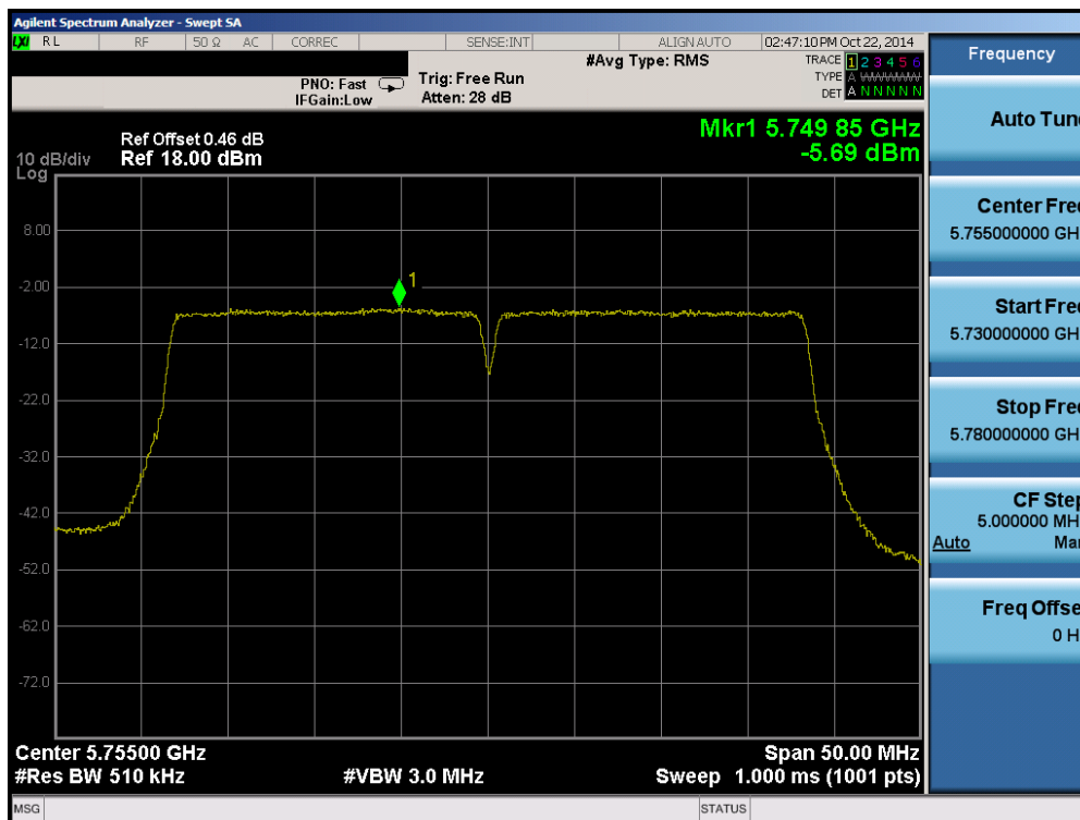
Plot 6-74. Peak Power Spectral Density Plot (40MHz BW 802.11n (UNII Band 3) – Ch. 151)
