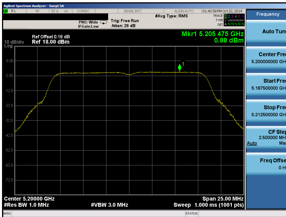
Plot 6-40. Peak Power Spectral Density Plot (802.11a (UNII Band 1) – Ch. 40)
