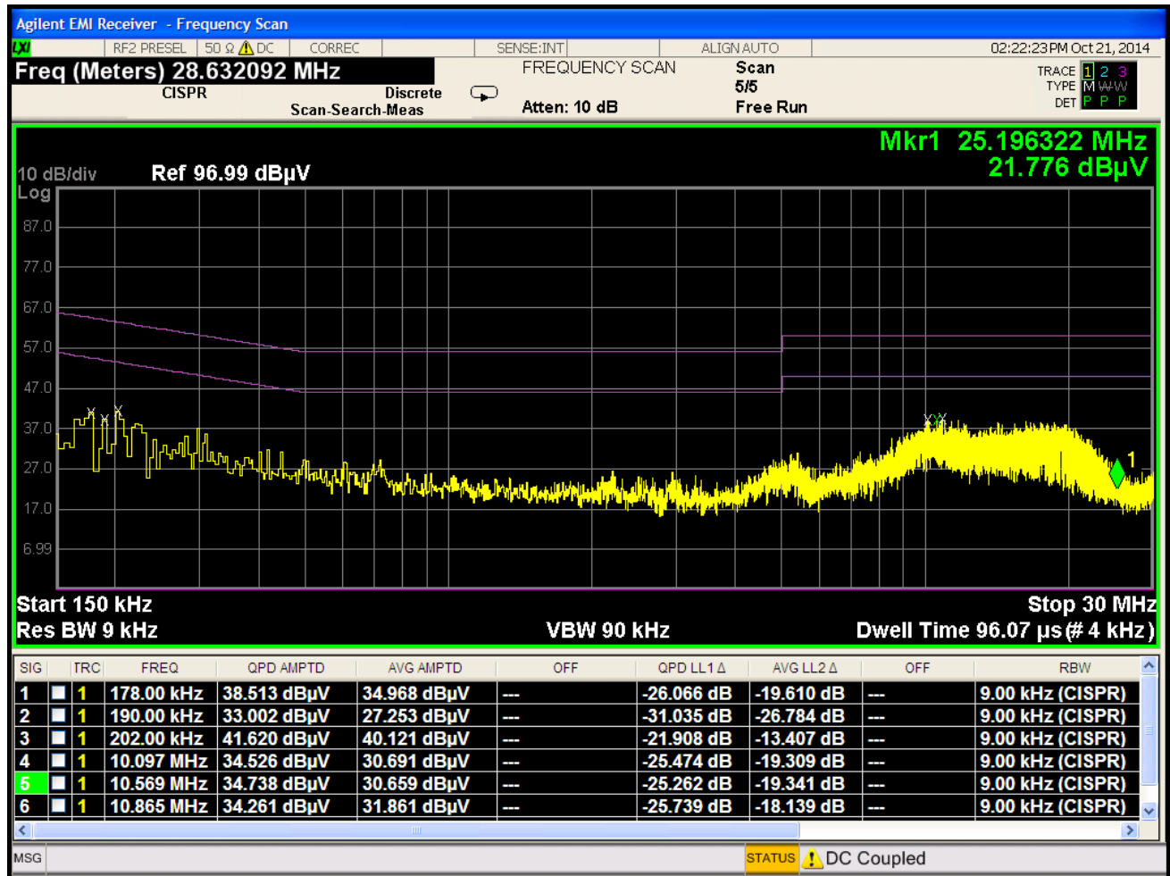
Plot 6-105. Line Conducted Plot with 802.11a UNII Band 2C (N)
