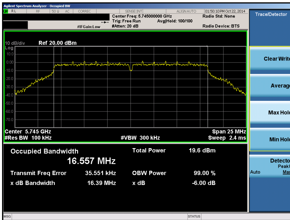
Plot 6-30. 6dB Bandwidth Plot (802.11a (UNII Band 3) – Ch. 149)
