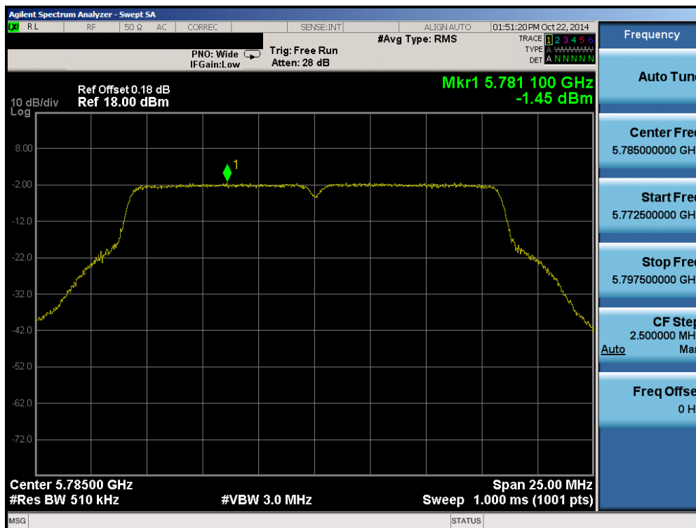
Plot 6-69. Peak Power Spectral Density Plot (802.11a (UNII Band 3) – Ch. 157)
