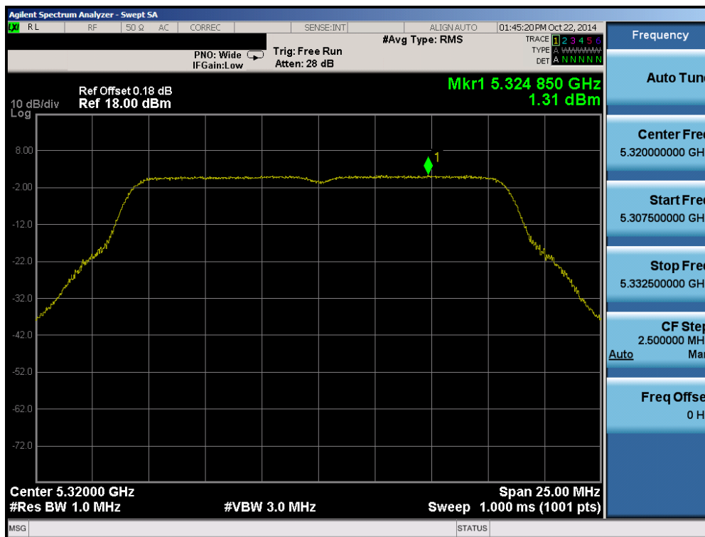
Plot 6-50. Peak Power Spectral Density Plot (802.11a (UNII Band 2A) – Ch. 64)
