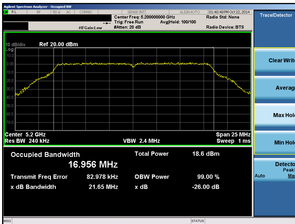
Plot 6-2. 26dB Bandwidth Plot (802.11a (UNII Band 1) – Ch. 40)
