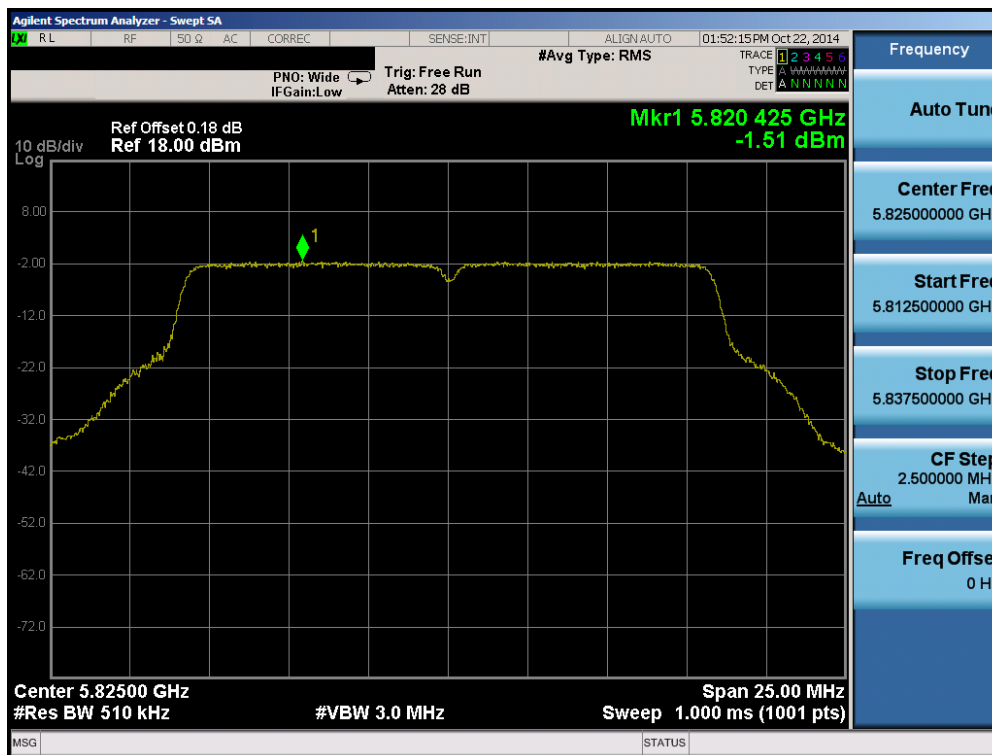
Plot 6-70. Peak Power Spectral Density Plot (802.11a (UNII Band 3) – Ch. 165)
