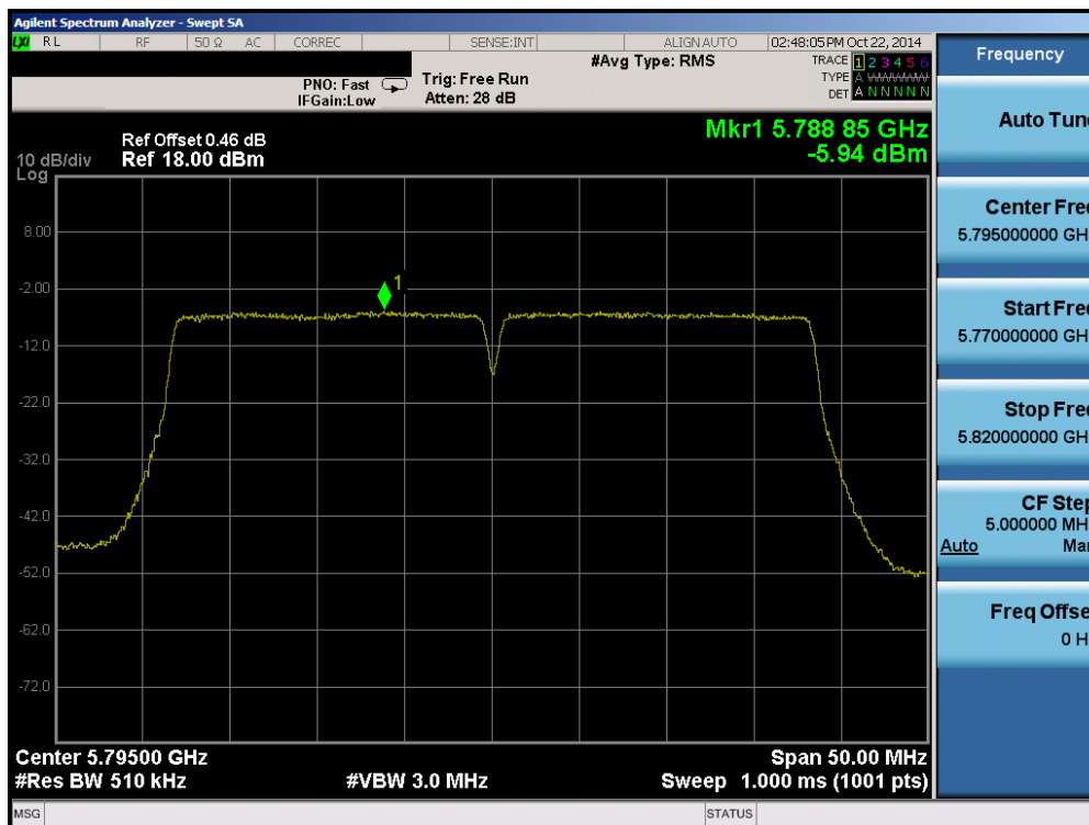
Plot 6-75. Peak Power Spectral Density Plot (40MHz BW 802.11n (UNII Band 3) – Ch. 159)
