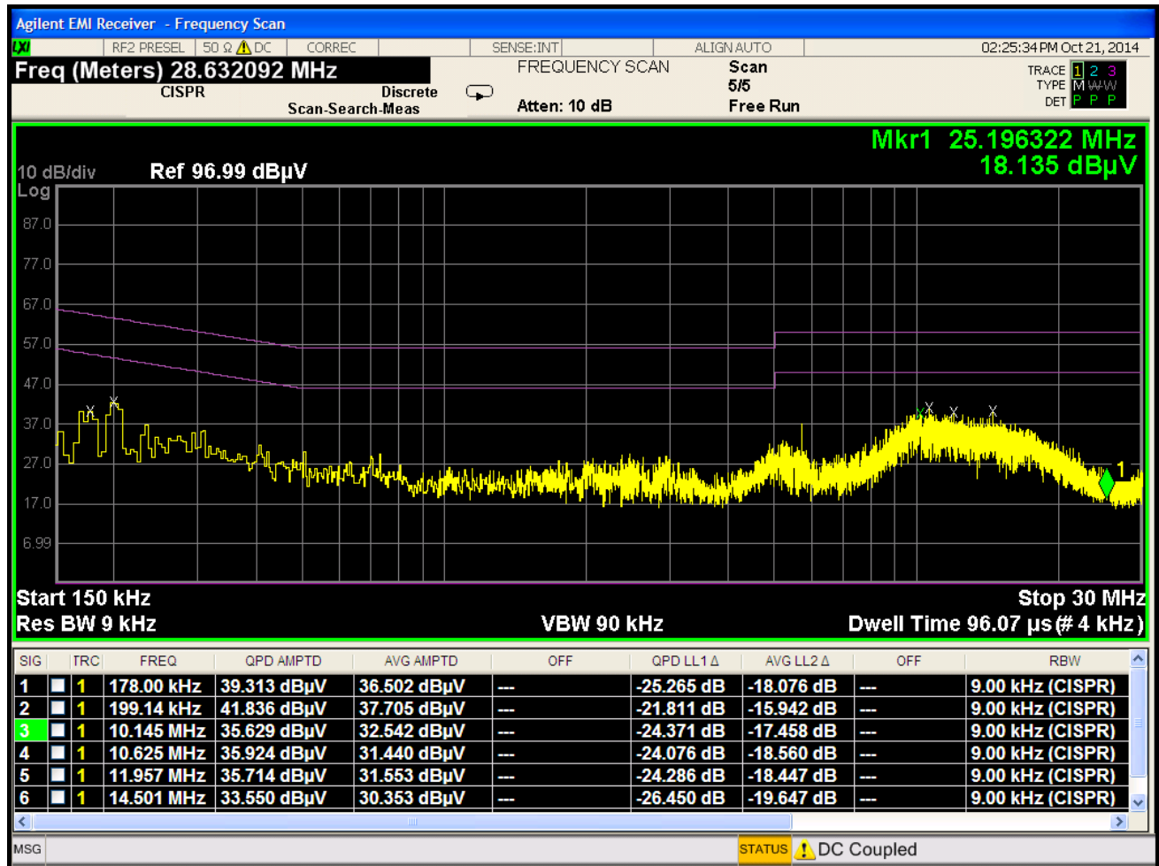
Plot 6-104. Line Conducted Plot with 802.11a UNII Band 2C (L1)
