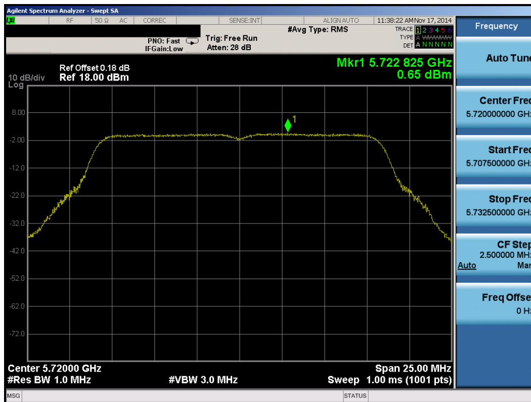
Plot 6-59. Peak Power Spectral Density Plot (802.11a (UNII Band 2C) – Ch. 144)
