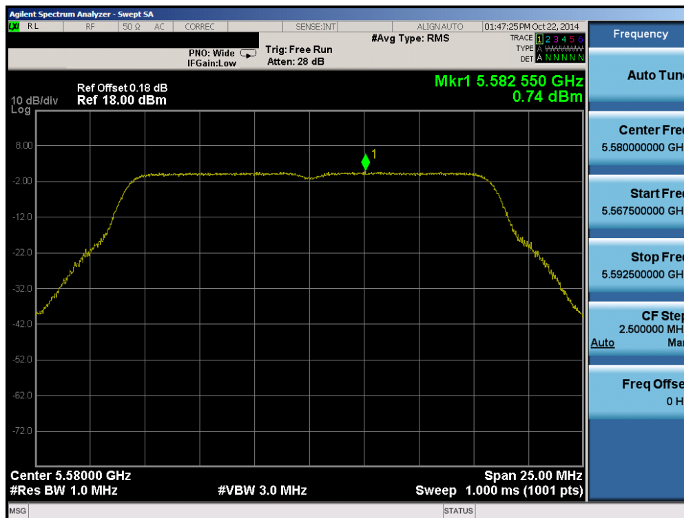
Plot 6-58. Peak Power Spectral Density Plot (802.11a (UNII Band 2C) – Ch. 116)
