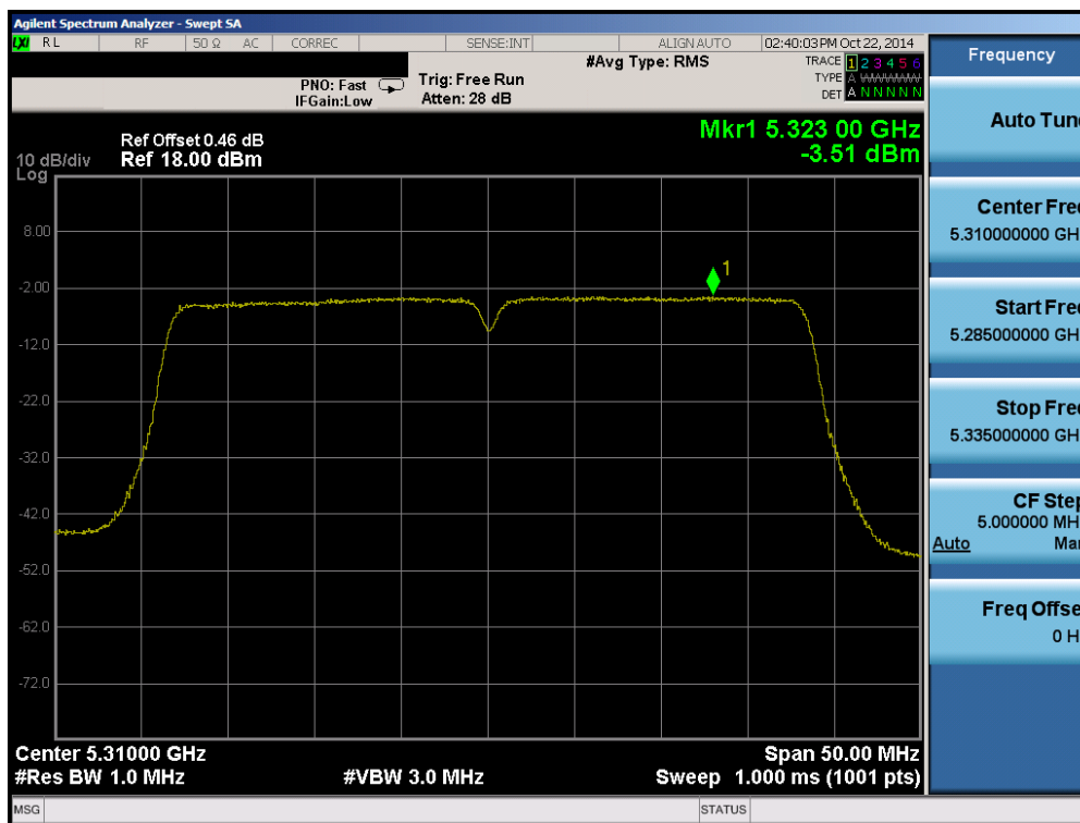
Plot 6-55. Peak Power Spectral Density Plot (40MHz BW 802.11n (UNII Band 2A) – Ch. 62)
