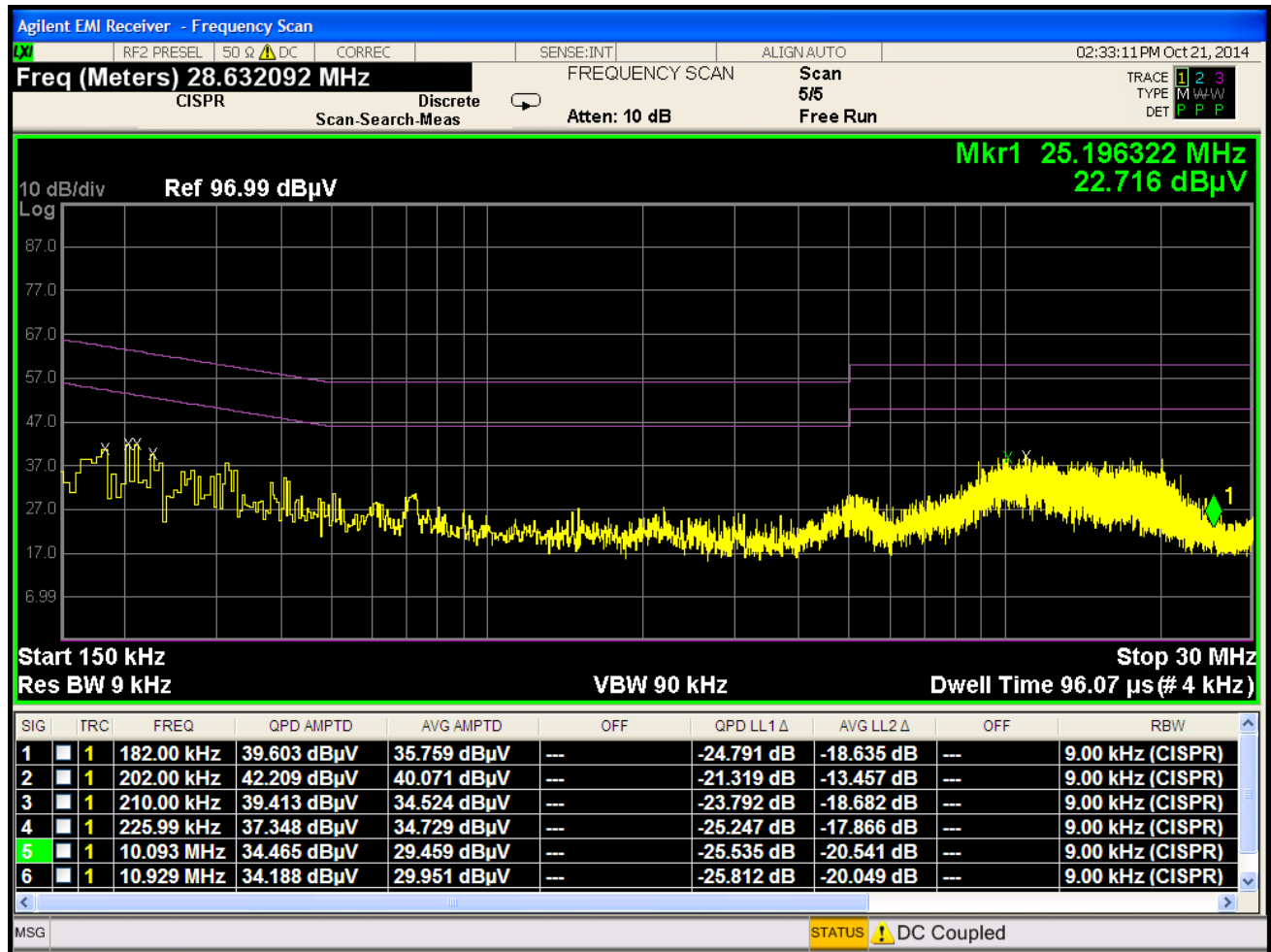
Plot 6-107. Line Conducted Plot with 802.11a UNII Band 3 (N)
