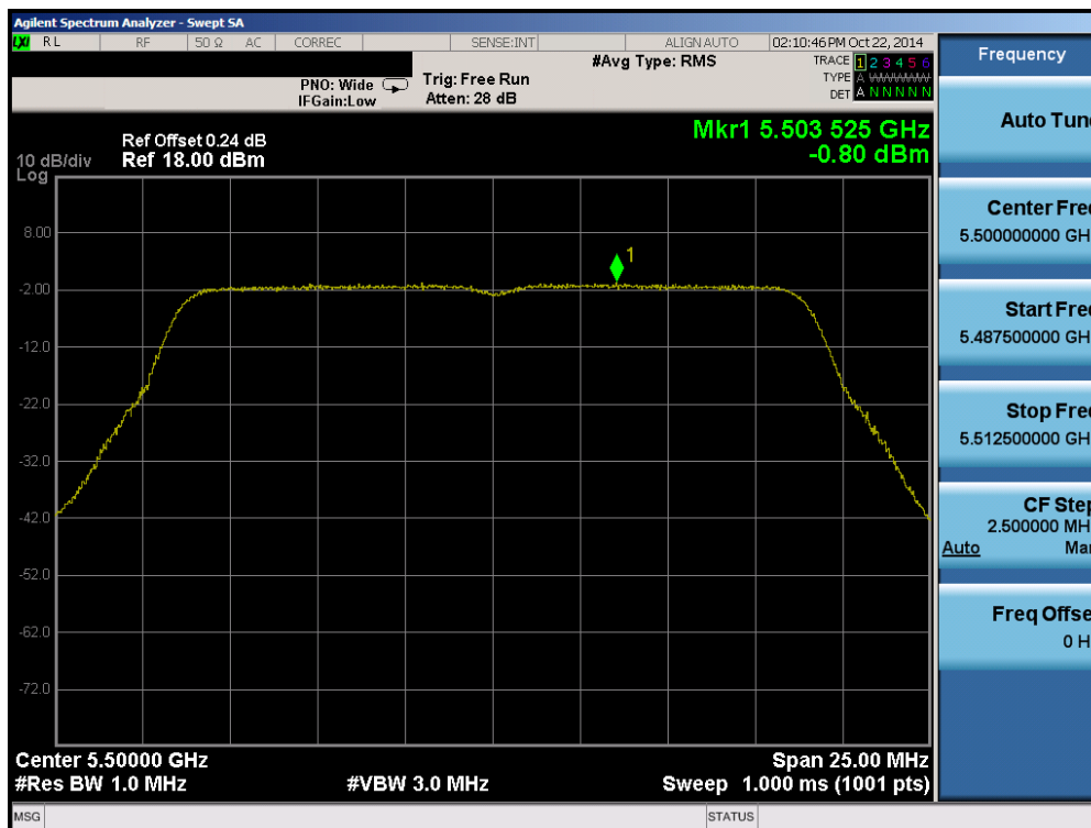
Plot 6-60. Peak Power Spectral Density Plot (20MHz BW 802.11n (UNII Band 2C) – Ch. 100)
