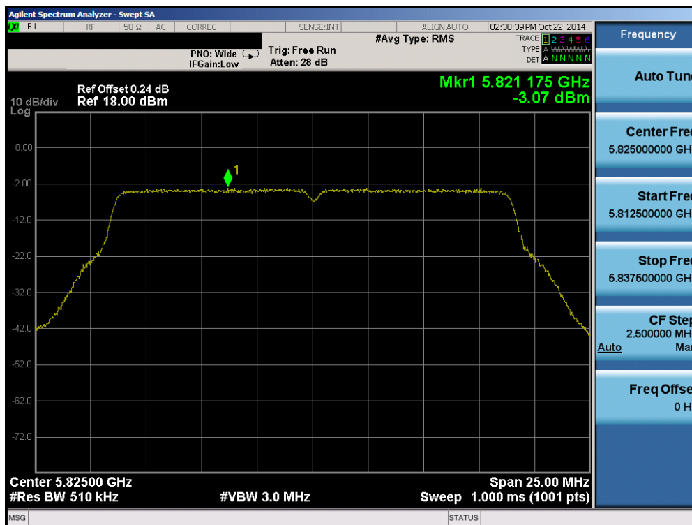
Plot 6-73. Peak Power Spectral Density Plot (20MHz BW 802.11n (UNII Band 3) – Ch. 165)
