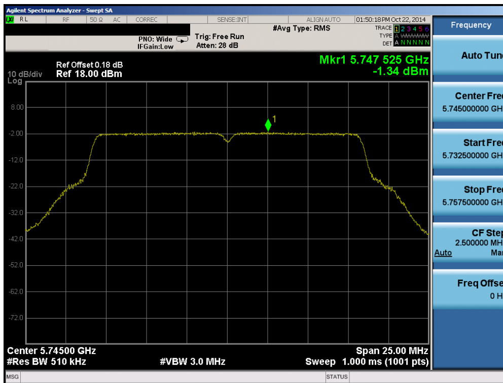
Plot 6-68. Peak Power Spectral Density Plot (802.11a (UNII Band 3) – Ch. 149)
