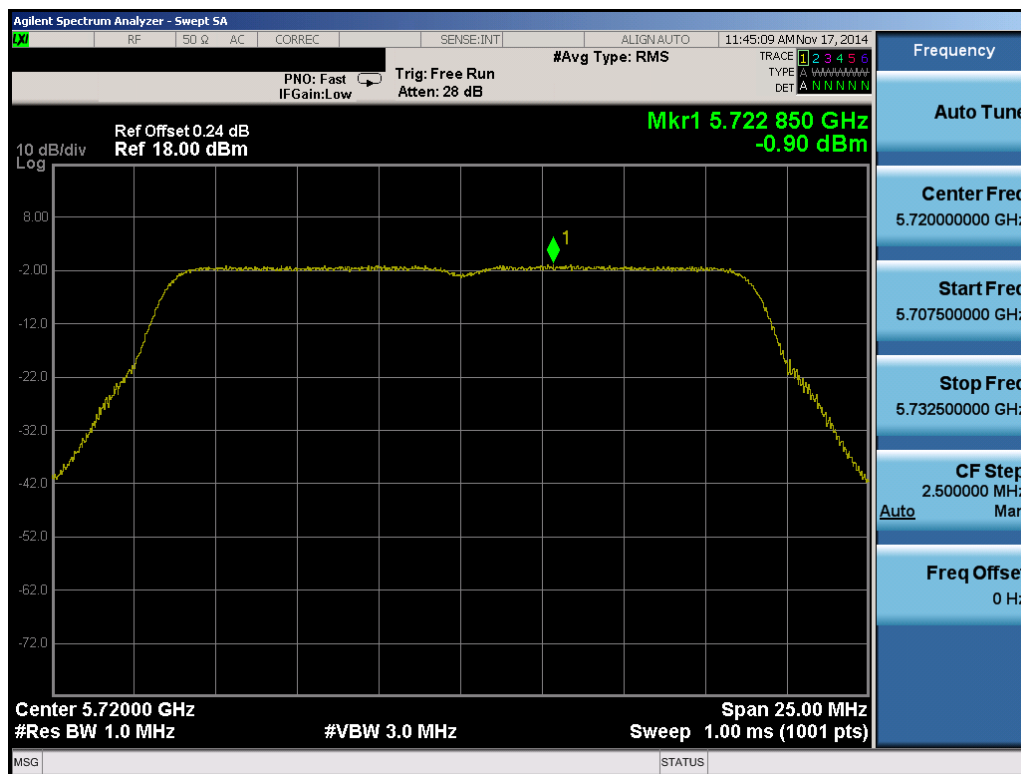
Plot 6-62. Peak Power Spectral Density Plot (20MHz BW 802.11n (UNII Band 2C) – Ch. 144)
