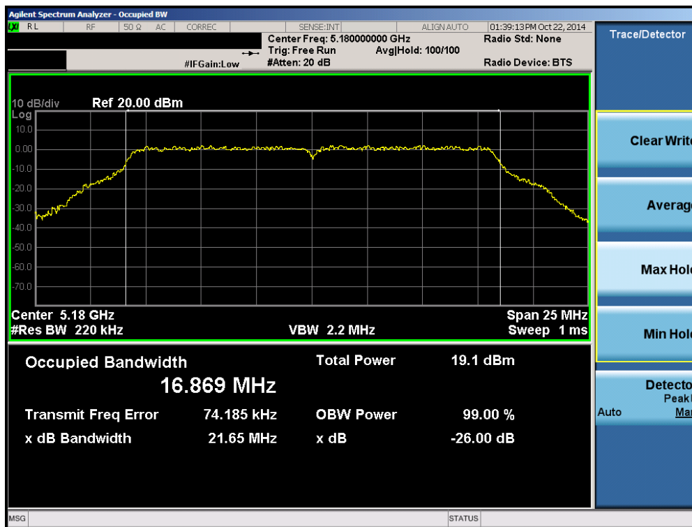
Plot 6-1. 26dB Bandwidth Plot (802.11a (UNII Band 1) – Ch. 36)
