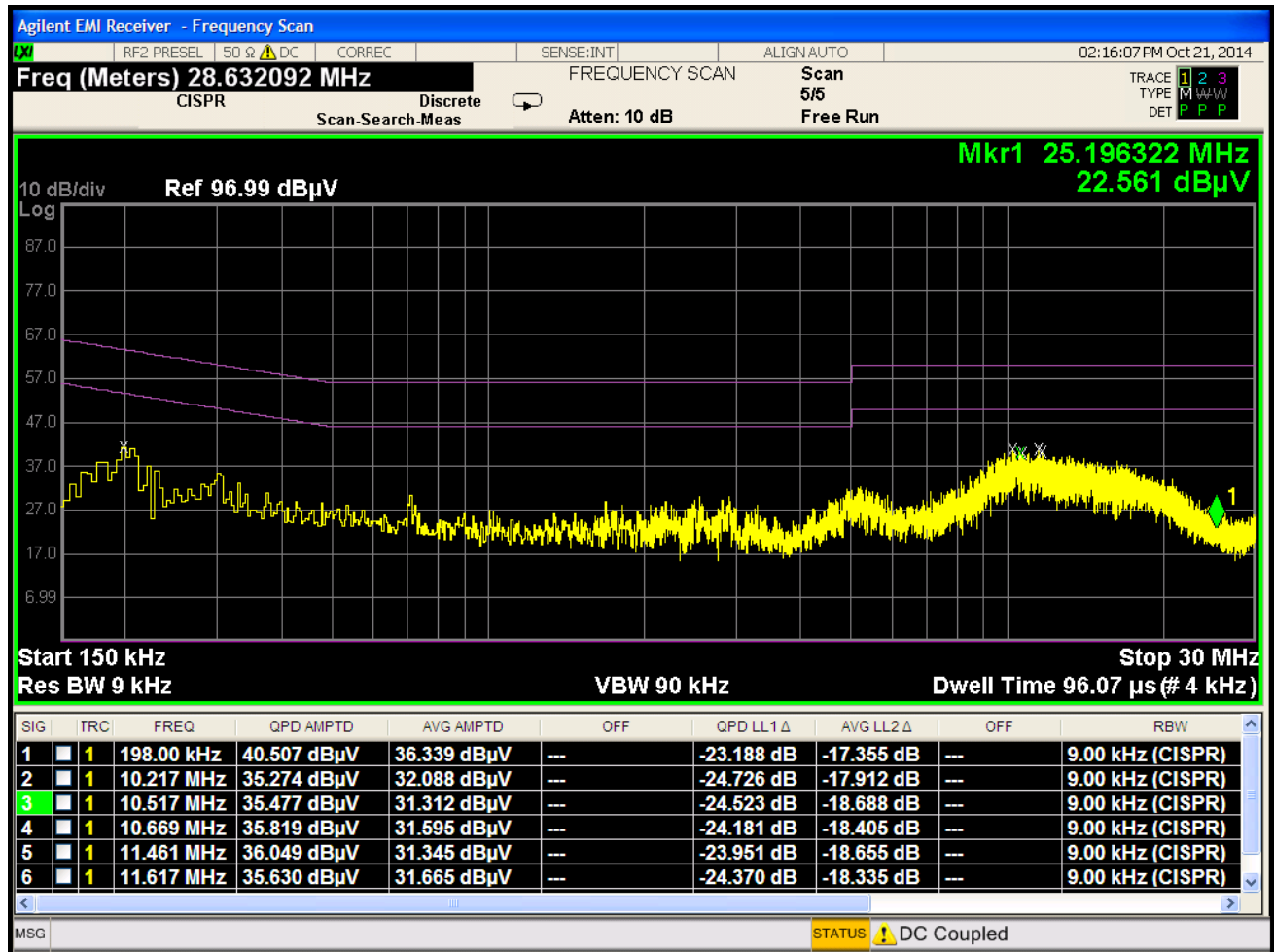
Plot 6-102. Line Conducted Plot with 802.11a UNII Band 2A (L1)
