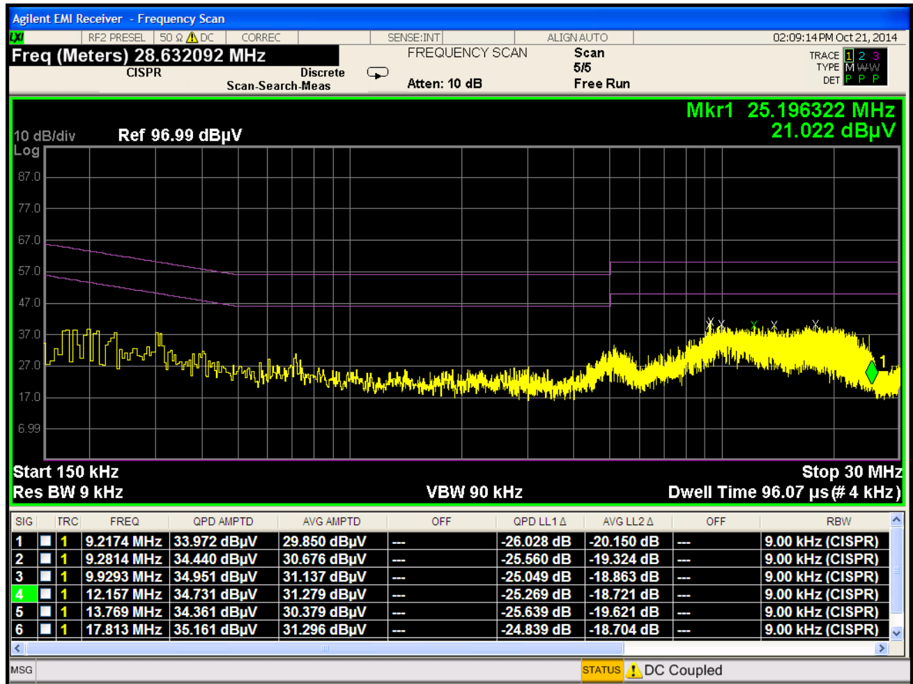
Plot 6-101. Line Conducted Plot with 802.11a UNII Band 1 (N)
