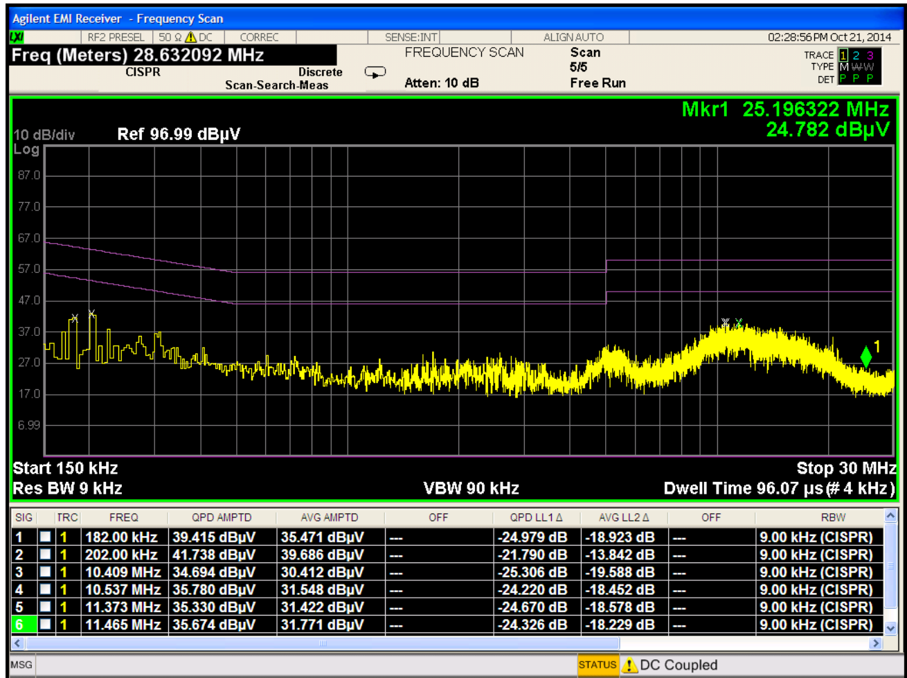
Plot 6-106. Line Conducted Plot with 802.11a UNII Band 3 (L1)
