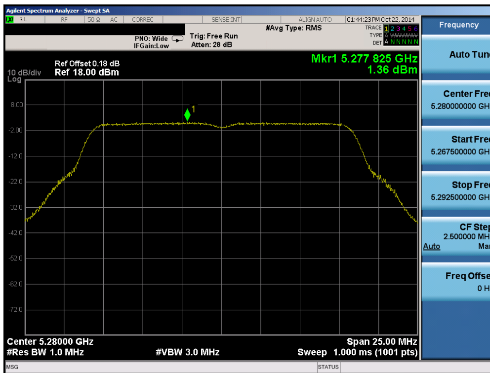
Plot 6-49. Peak Power Spectral Density Plot (802.11a (UNII Band 2A) – Ch. 56)
