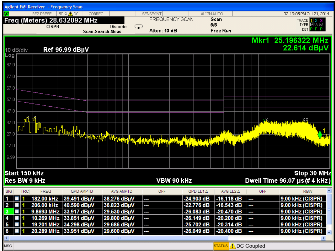
Plot 6-103. Line Conducted Plot with 802.11a UNII Band 2A (N)
