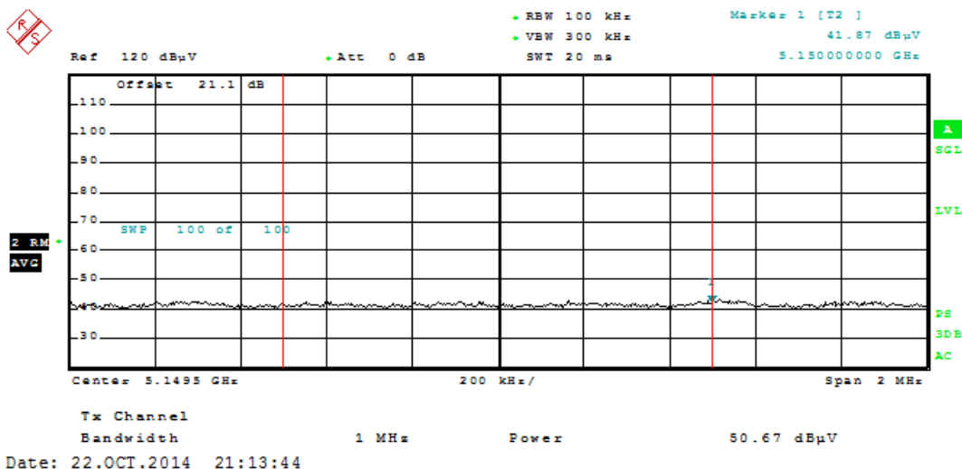
Plot 6-92. Radiated Restricted Lower Band Edge Plot (Average – UNII Band 1)
