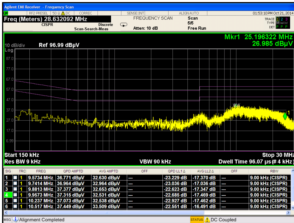
Plot 6-35. Line Conducted Plot with 802.11b (L1)
