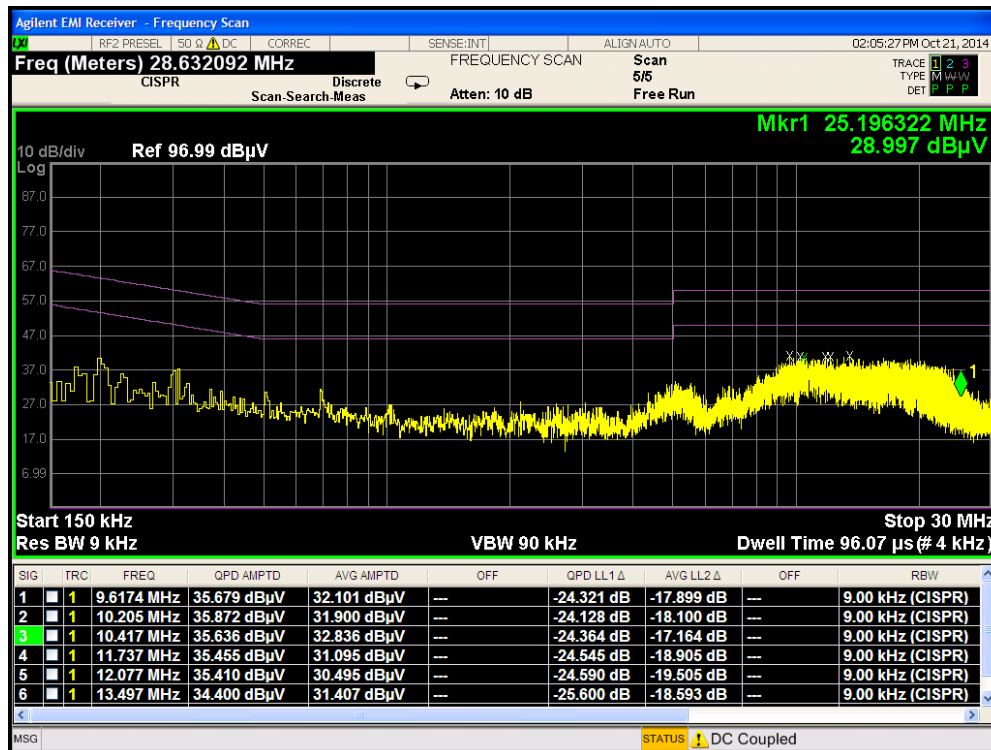
Plot 6-36. Line Conducted Plot with 802.11b (N)
