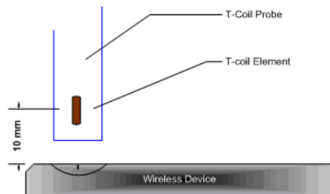
Figure 4-11 Measurement Distance
