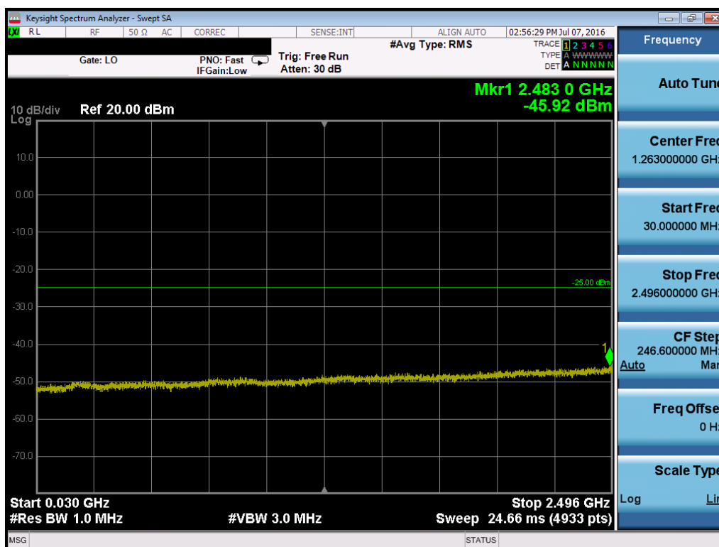
Plot 7-90. Conducted Spurious Plot (Band 41 – 10.0MHz QPSK – RB Size 1, RB Offset 0 – Mid Channel)
