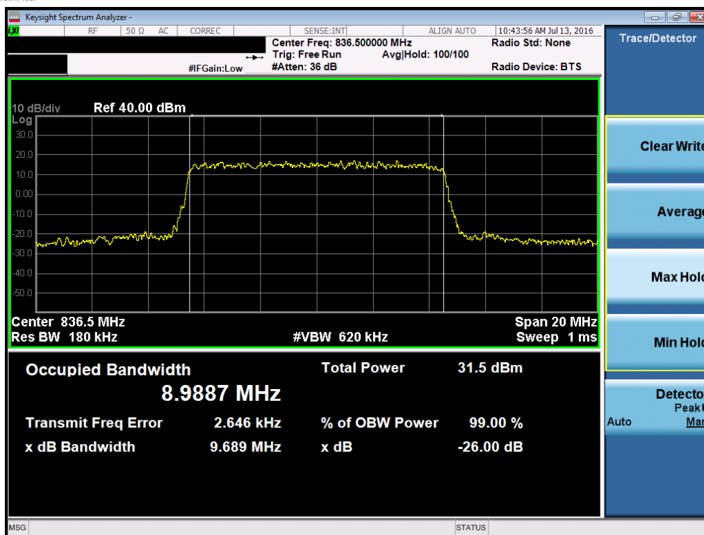
Plot 7-15. Occupied Bandwidth Plot (Band 5/26 – 10.0MHz QPSK – RB Size 50)
