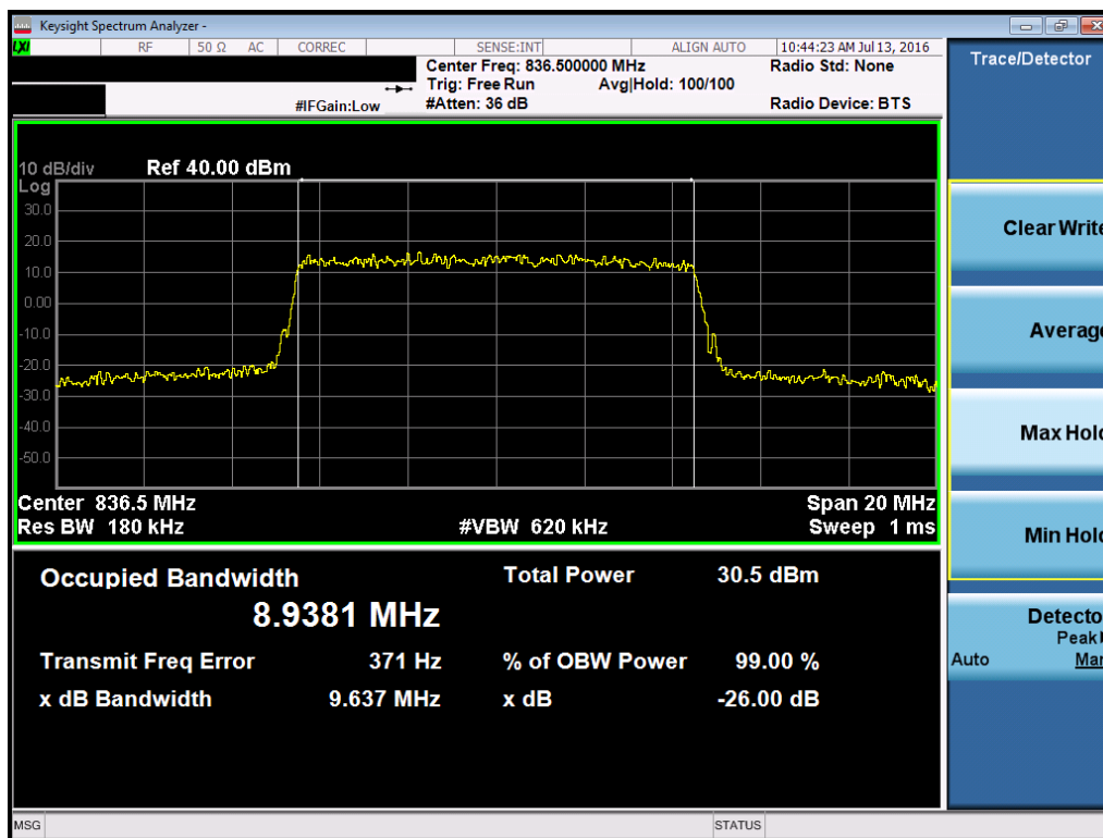
Plot 7-16. Occupied Bandwidth Plot (Band 5/26 – 10.0MHz 16-QAM – RB Size 50)
