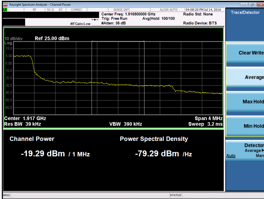
Plot 7-153. Upper Extended Band Edge Plot (Band 2/25 – 3.0MHz QPSK – RB Size 15)
