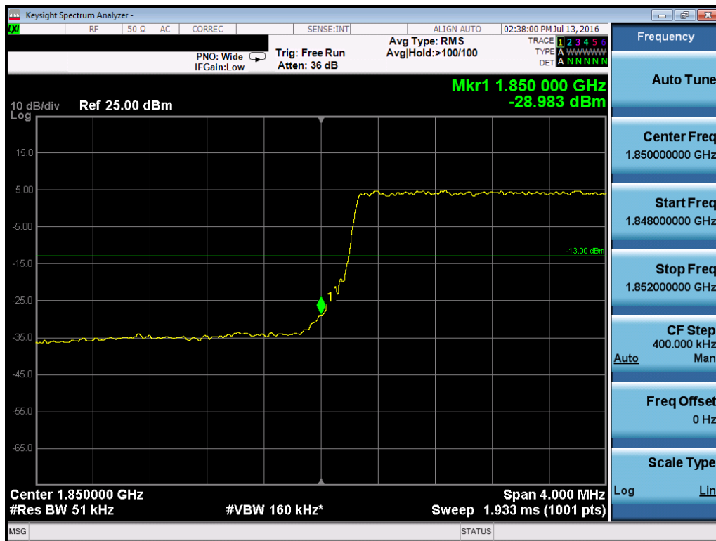
Plot 7-154. Lower Band Edge Plot (Band 2/25 – 5.0MHz QPSK – RB Size 25)
