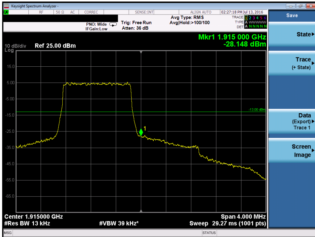
Plot 7-148. Upper Band Edge Plot (Band 2/25 – 1.4MHz QPSK – RB Size 6)
