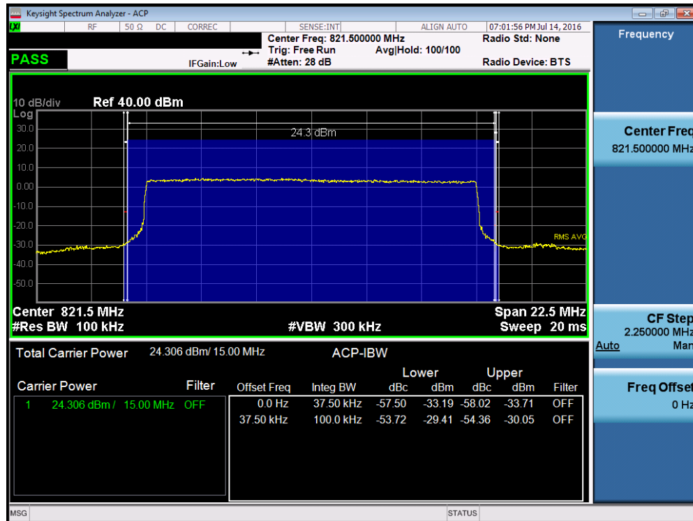
Plot 7-24. Channel Edge Plot (15MHz QPSK – RB Size 75)
