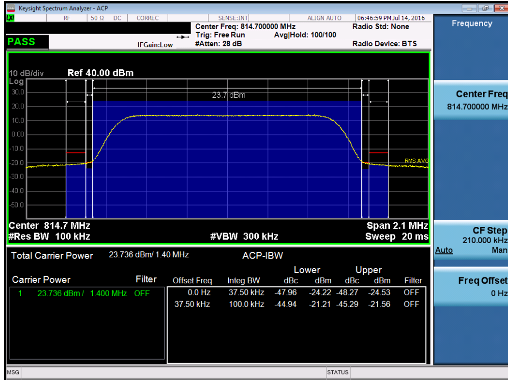
Plot 7-17. Channel Edge Plot (1.4MHz QPSK – RB Size 6– Low Channel)
