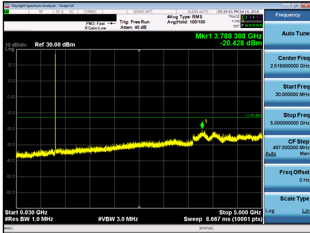
Plot 7-15. Conducted Spurious Plot (3MHz QPSK – RB Size 1, RB Offset 0 – High Channel)
