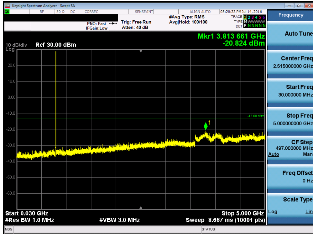
Plot 7-13. Conducted Spurious Plot (3MHz QPSK – RB Size 1, RB Offset 0 – Low Channel)
