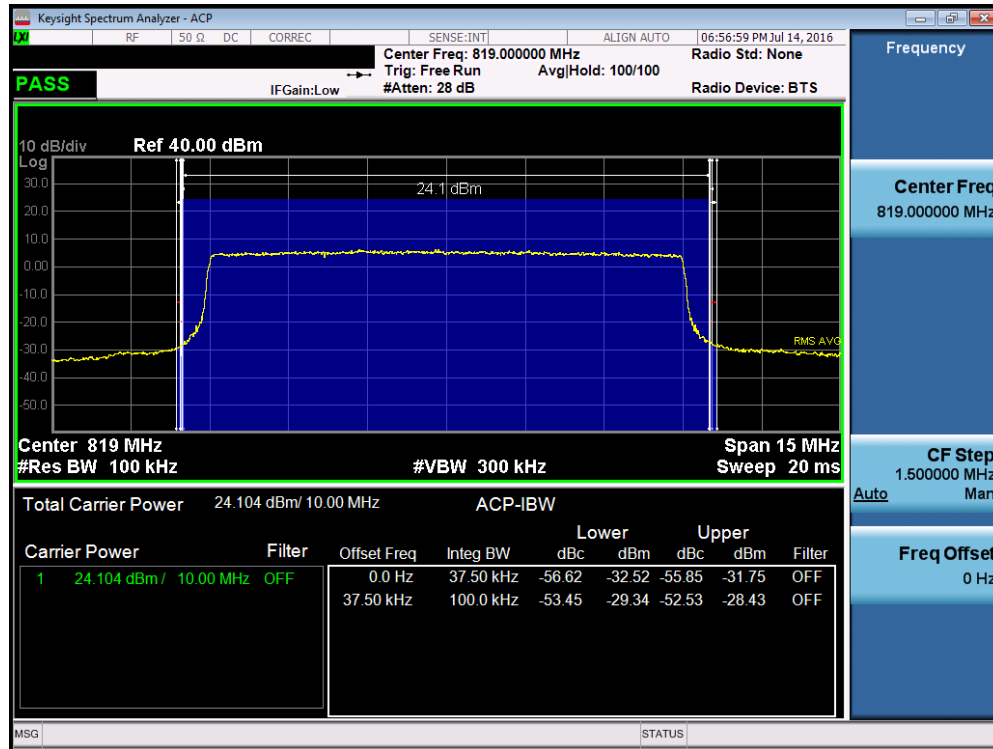
Plot 7-23. Channel Edge Plot (10MHz QPSK – RB Size 50)
