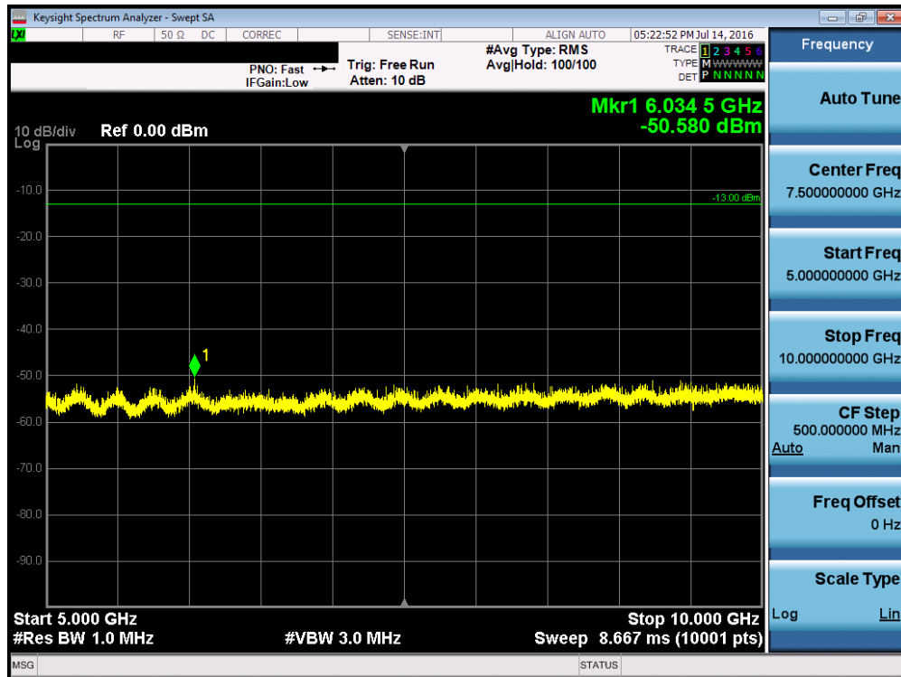
Plot 7-16. Conducted Spurious Plot (3MHz QPSK – RB Size 1, RB Offset 0 – High Channel)
