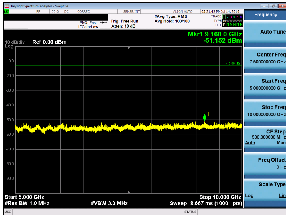
Plot 7-14. Conducted Spurious Plot (3MHz QPSK – RB Size 1, RB Offset 0 – Low Channel)
