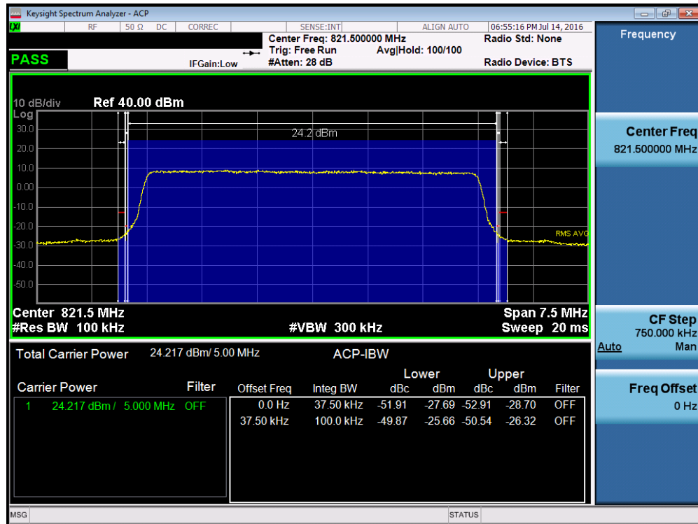
Plot 7-22. Channel Edge Plot (5MHz QPSK – RB Size 25 – High Channel)
