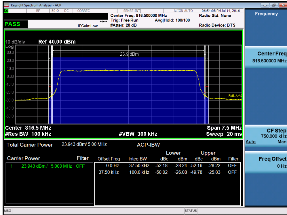
Plot 7-21. Channel Edge Plot (5MHz QPSK – RB Size 25– Low Channel)
