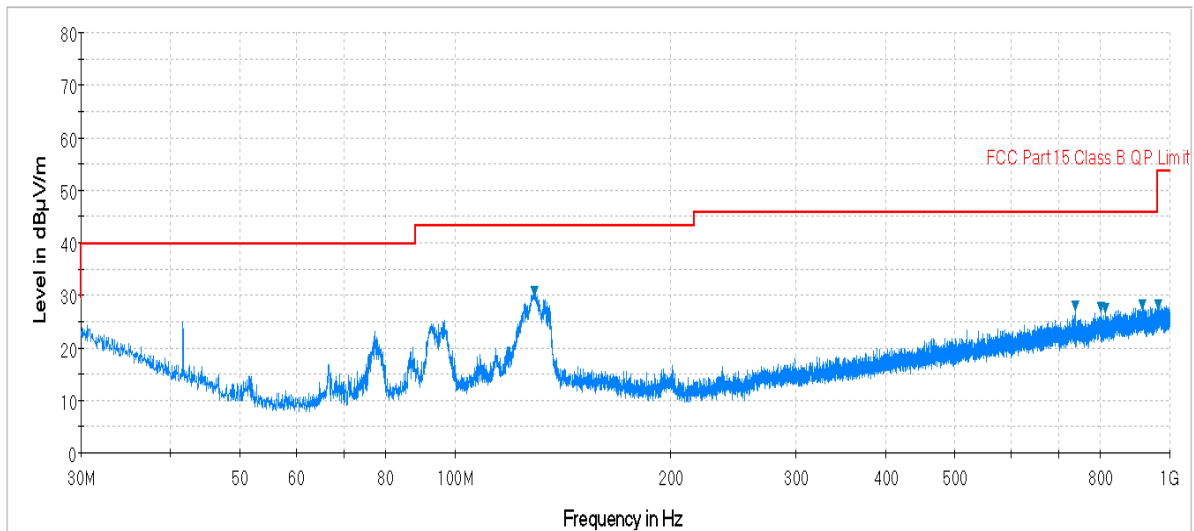
Plot 7-12. Radiated Spurious Plot below 1GHz (Pol. V)
