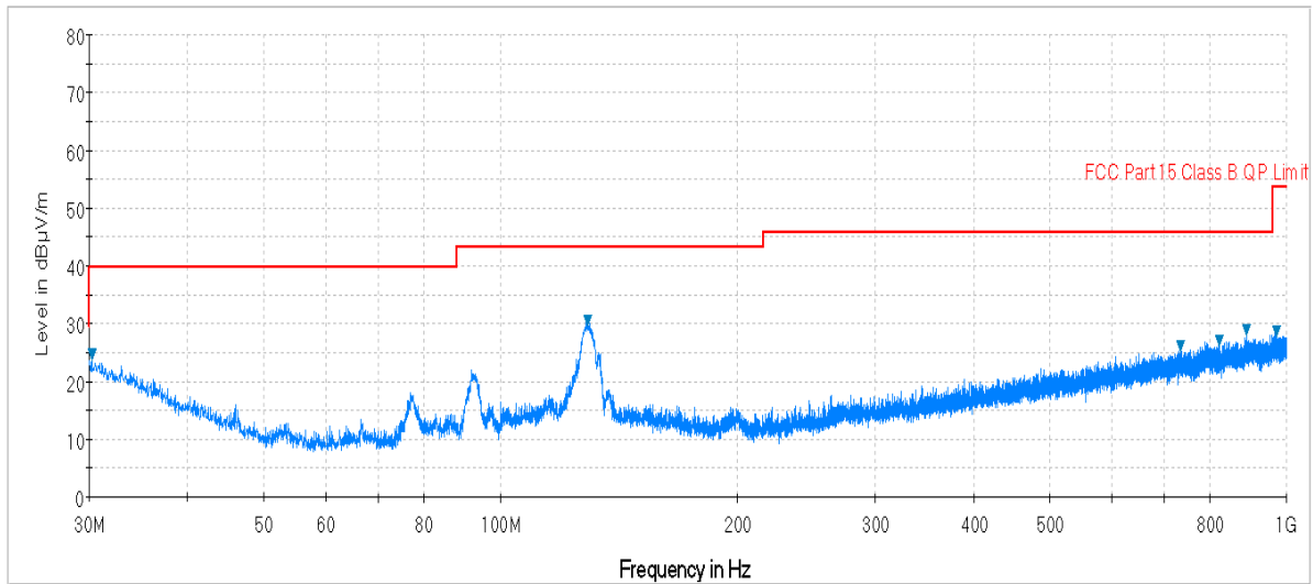
Plot 7-11. Radiated Spurious Plot below 1GHz (Pol. H)
