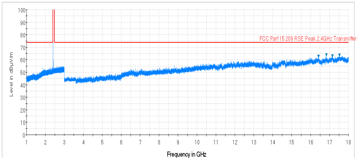
Plot 7-2. Radiated Spurious Plot above 1GHz (BT – Ch. 0, Ant. Pol. V)
