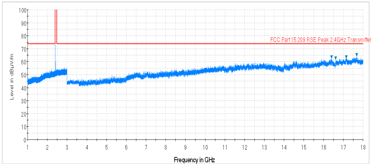
Plot 7-1. Radiated Spurious Plot above 1GHz (BT – Ch. 0, Ant. Pol. H)
