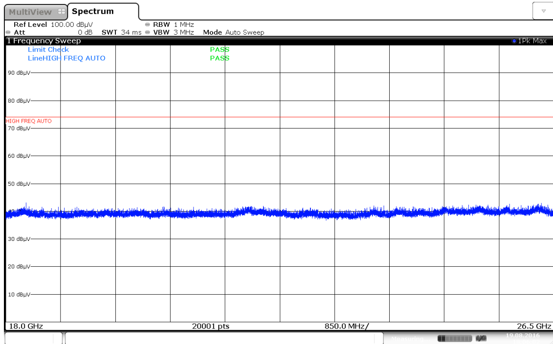
Plot 7-8. Radiated Spurious Plot above 18GHz (Pol. V)
