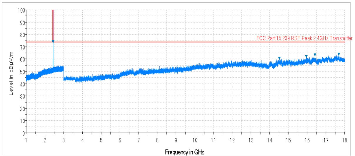
Plot 7-4. Radiated Spurious Plot above 1GHz (BT – Ch. 39, Ant. Pol. V)
