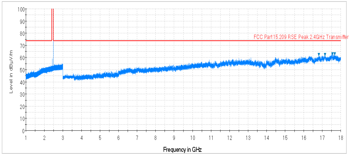
Plot 7-5. Radiated Spurious Plot above 1GHz (BT – Ch. 78, Ant. Pol. H)
