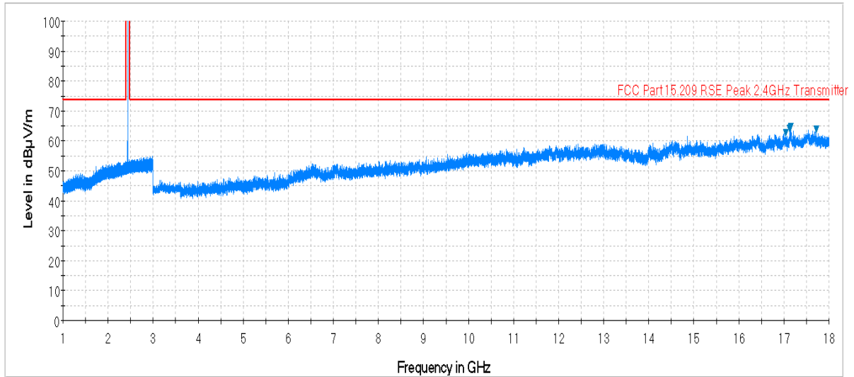
Plot 7-3. Radiated Spurious Plot above 1GHz (BT – Ch. 39, Ant. Pol. H)
