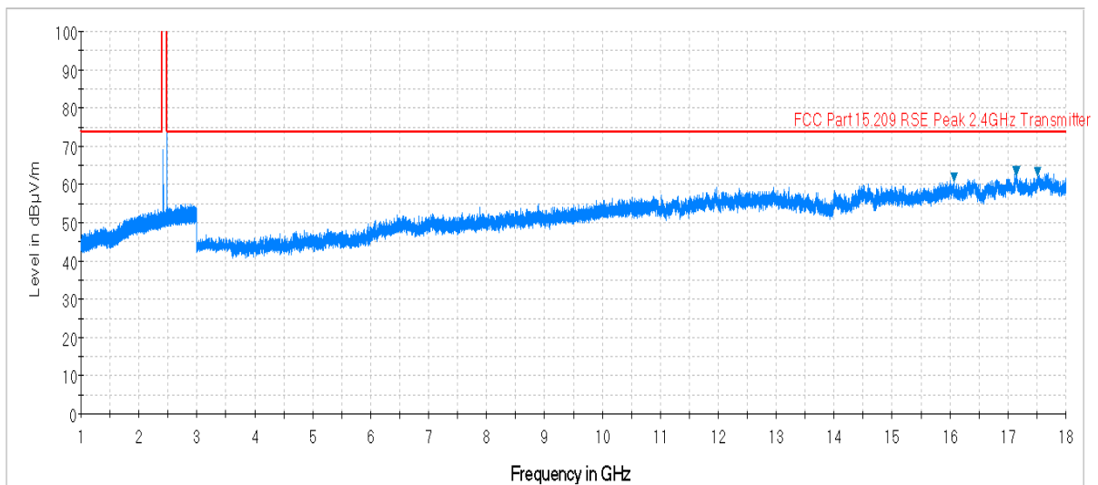
Plot 7-6. Radiated Spurious Plot above 1GHz (BT – Ch. 78, Ant. Pol. V)
