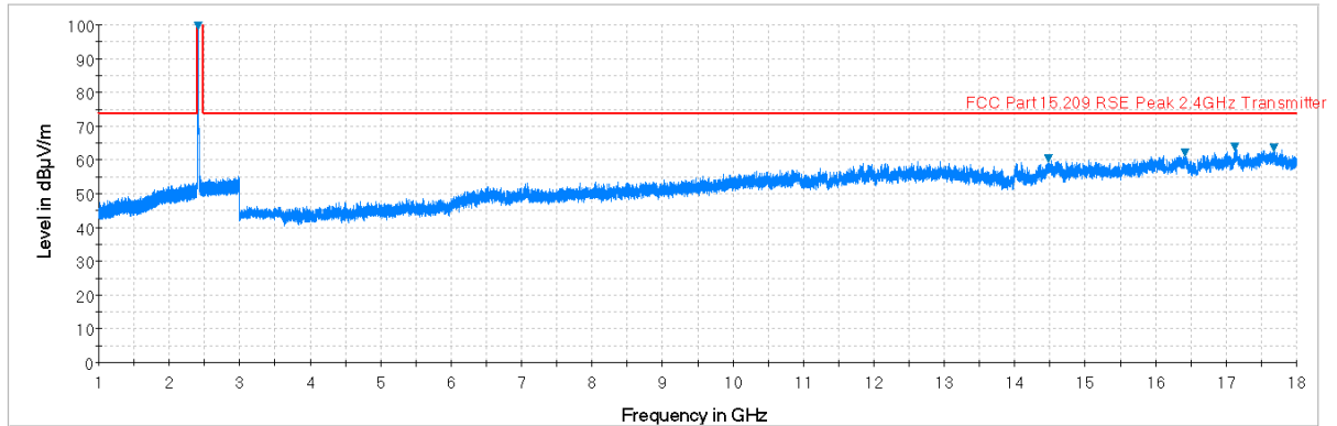
Plot 7-9. Radiated Spurious Plot above 1GHz (802.11b – Ch. 1, Ant. Pol. H)
