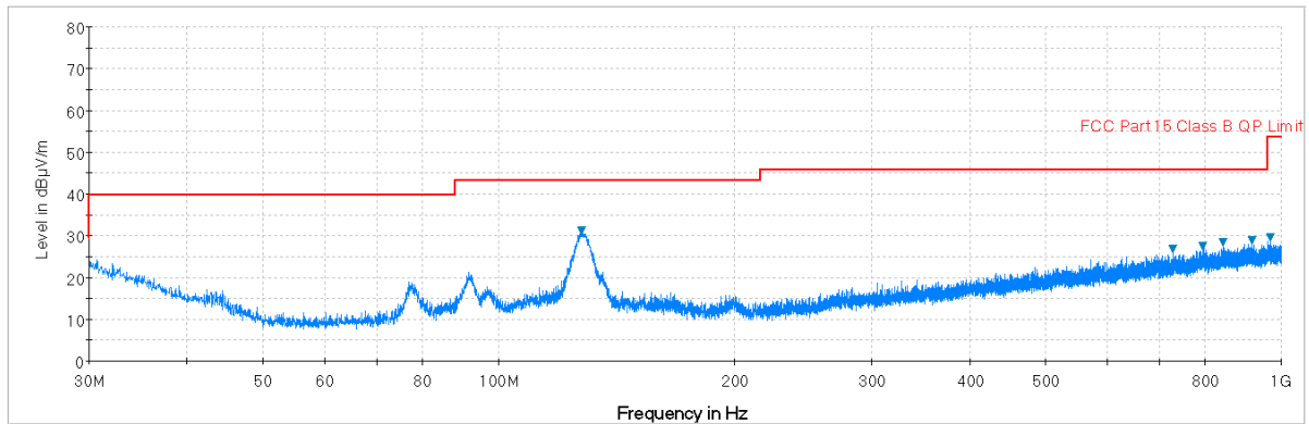
Plot 7-29. Radiated Spurious Plot below 1GHz (Pol. H)
