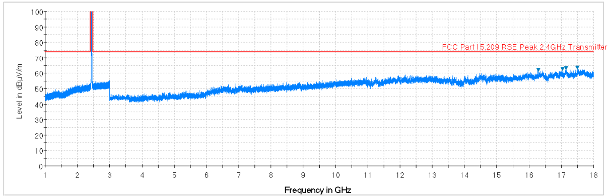
Plot 7-12. Radiated Spurious Plot above 1GHz (802.11b – Ch. 6, Ant. Pol. V)
