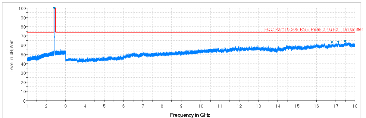
Plot 7-10. Radiated Spurious Plot above 1GHz (802.11b – Ch. 1, Ant. Pol. V)
