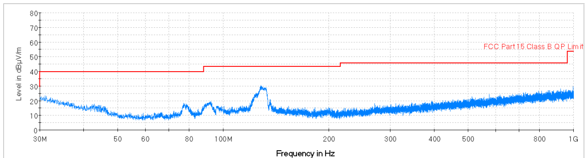
Plot 7-30. Radiated Spurious Plot below 1GHz (Pol. V)
