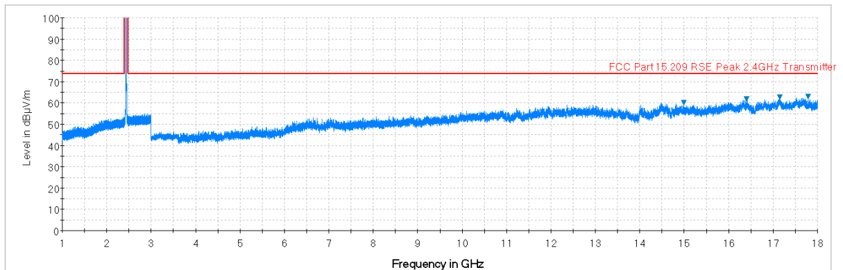
Plot 7-11. Radiated Spurious Plot above 1GHz (802.11b – Ch. 6, Ant. Pol. H)
