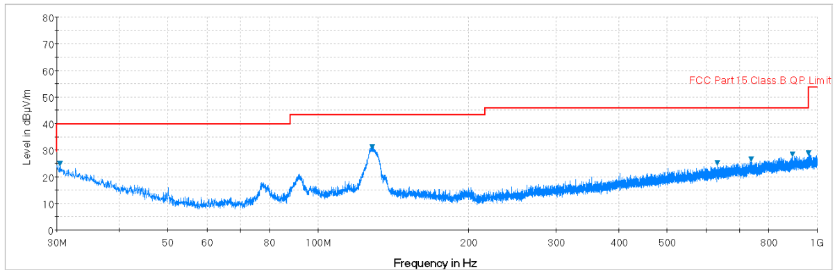
Plot 7-31. Radiated Spurious Plot below 1GHz (Pol. H)
