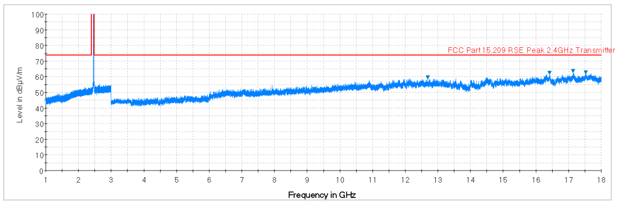
Plot 7-13. Radiated Spurious Plot above 1GHz (802.11b – Ch. 11, Ant. Pol. H)
