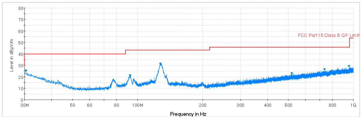
Plot 7-32. Radiated Spurious Plot below 1GHz (Pol. V)
