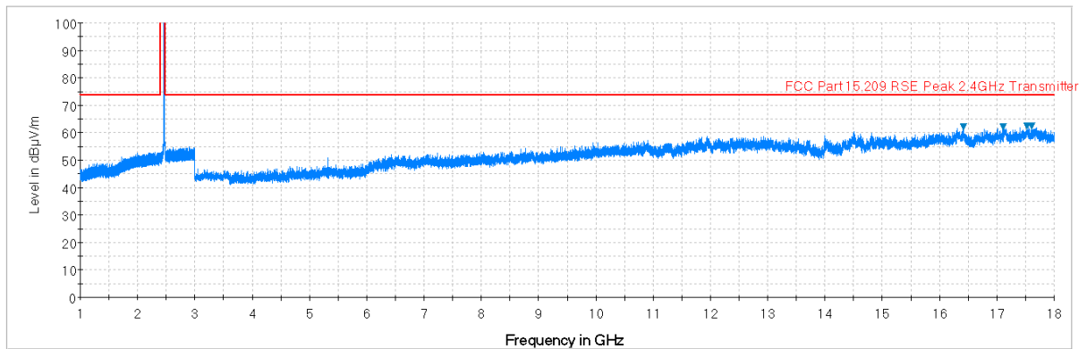
Plot 7-14. Radiated Spurious Plot above 1GHz (802.11b – Ch. 11, Ant. Pol. V)
