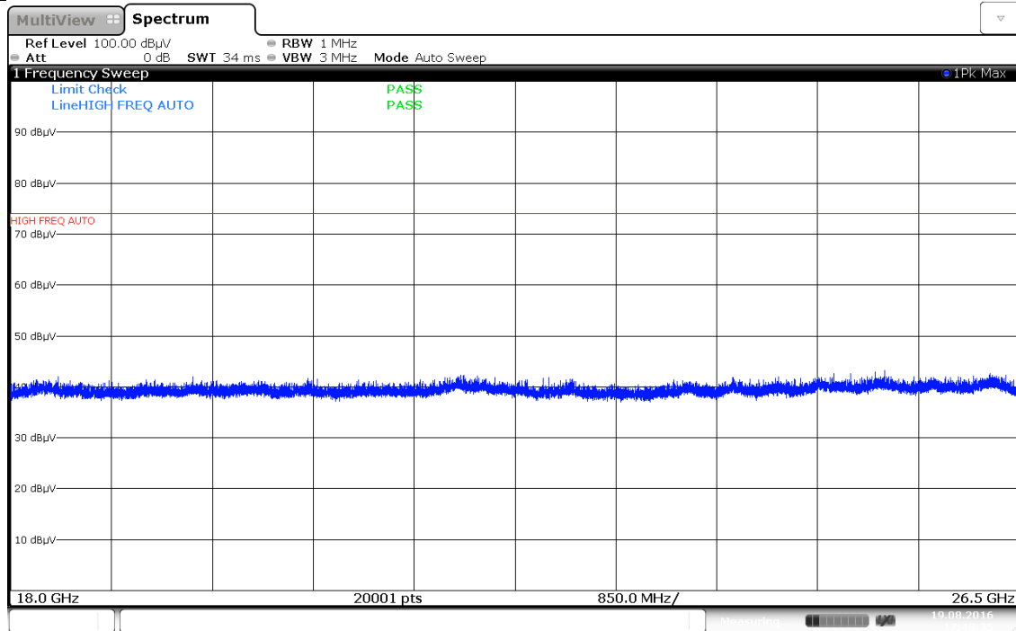
Plot 7-15. Radiated Spurious Plot above 18GHz (Pol. H)
