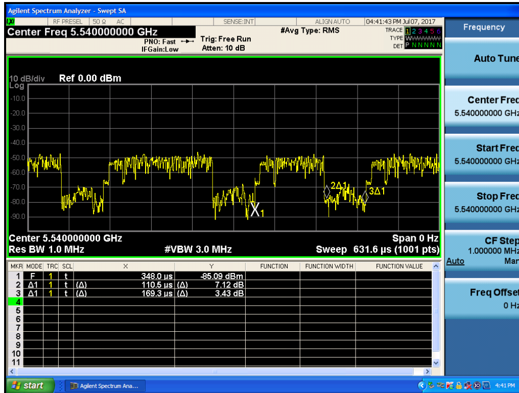
Figure 5-2. Band 2C Channel Loading
