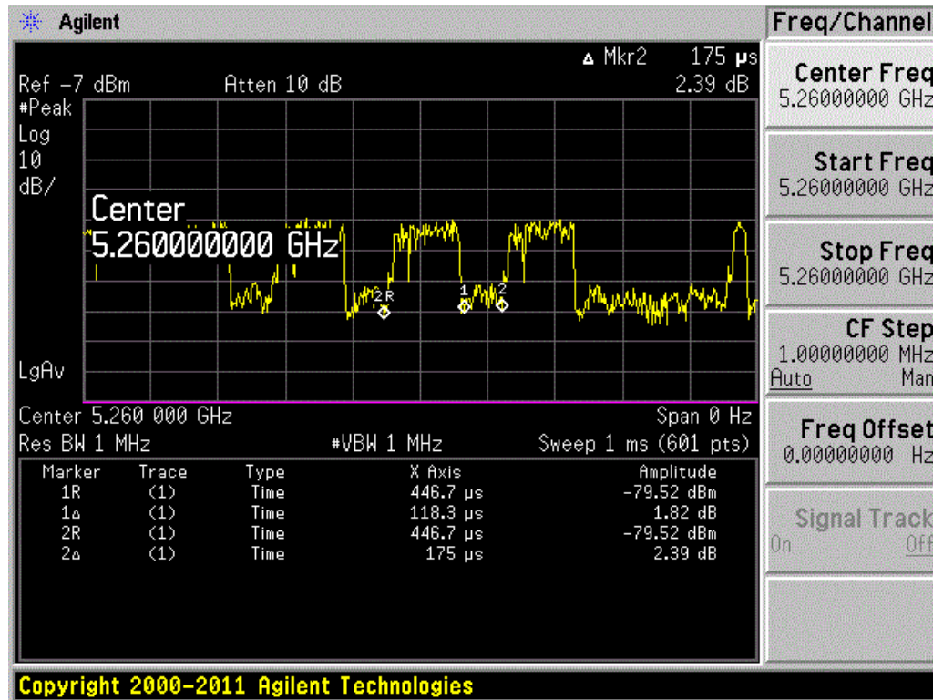
Figure 5-1. Band 2A Channel Loading
