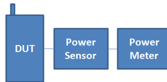
Figure 6-1 Power Measurement Setup for unlicensed modes
