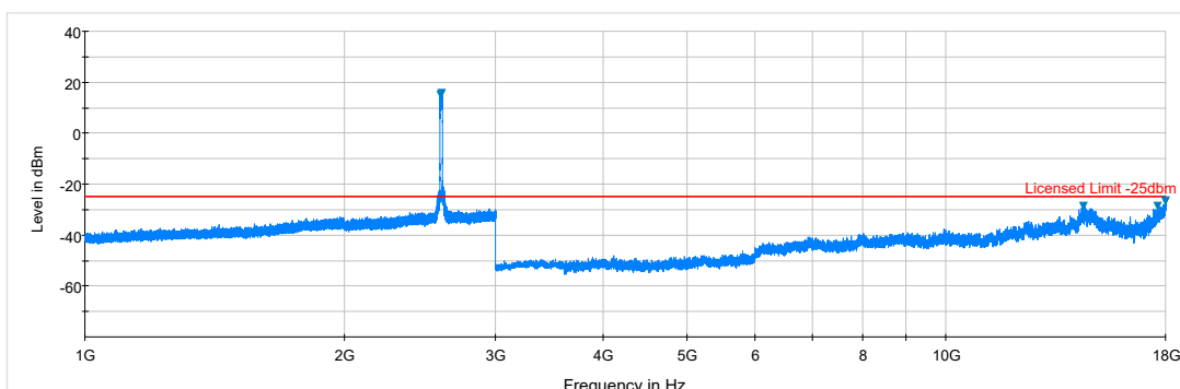
Plot 7-254. Radiated Spurious Plot (ULCA B41 PCC: RB 100 Offset 0, SCC: RB 100 Offset 0, Ant. Pol. H)
