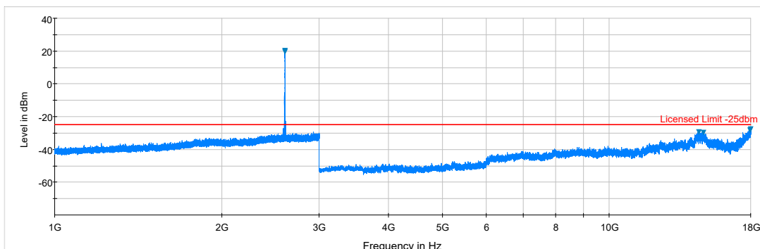
Plot 7-253. Radiated Spurious Plot (ULCA B41 PCC: RB 1 Offset 99, SCC: RB 1 Offset 0, Ant. Pol. V)
