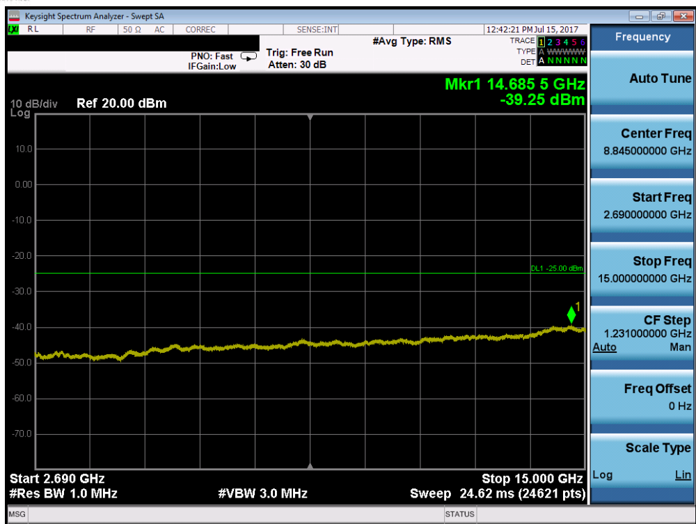
Plot 7-228. Conducted Spurious Plot (Band 41 – 20.0MHz QPSK – PCC 1/99 SCC 1/0 – Mid Channel)
