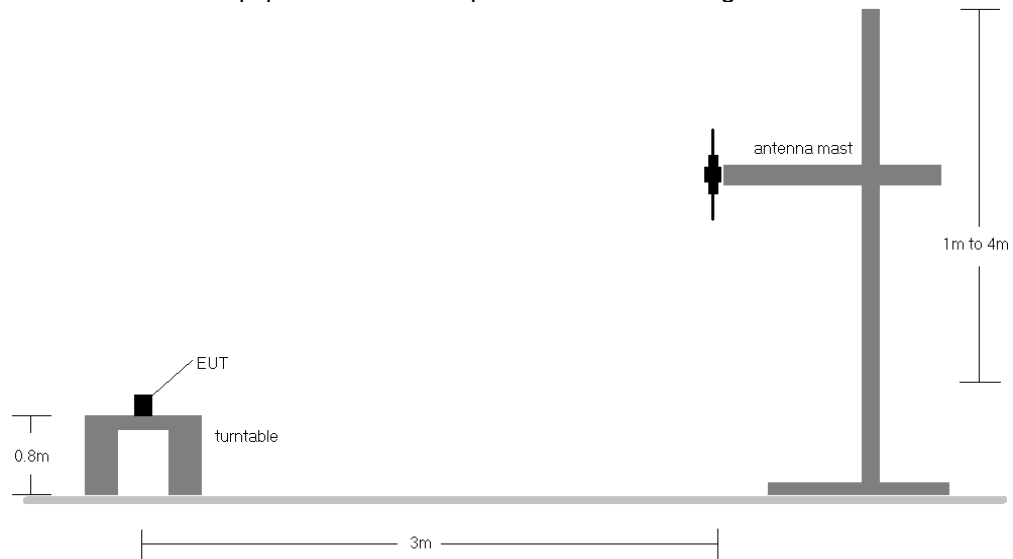
Figure 7-4. Radiated Test Setup <1GHz
