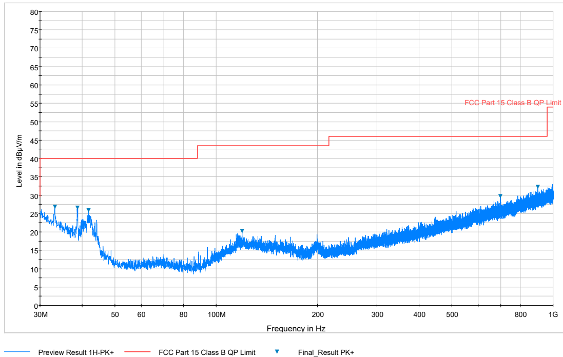
Plot 7-54. Radiated Spurious Plot below 1GHz (Pol. H)
