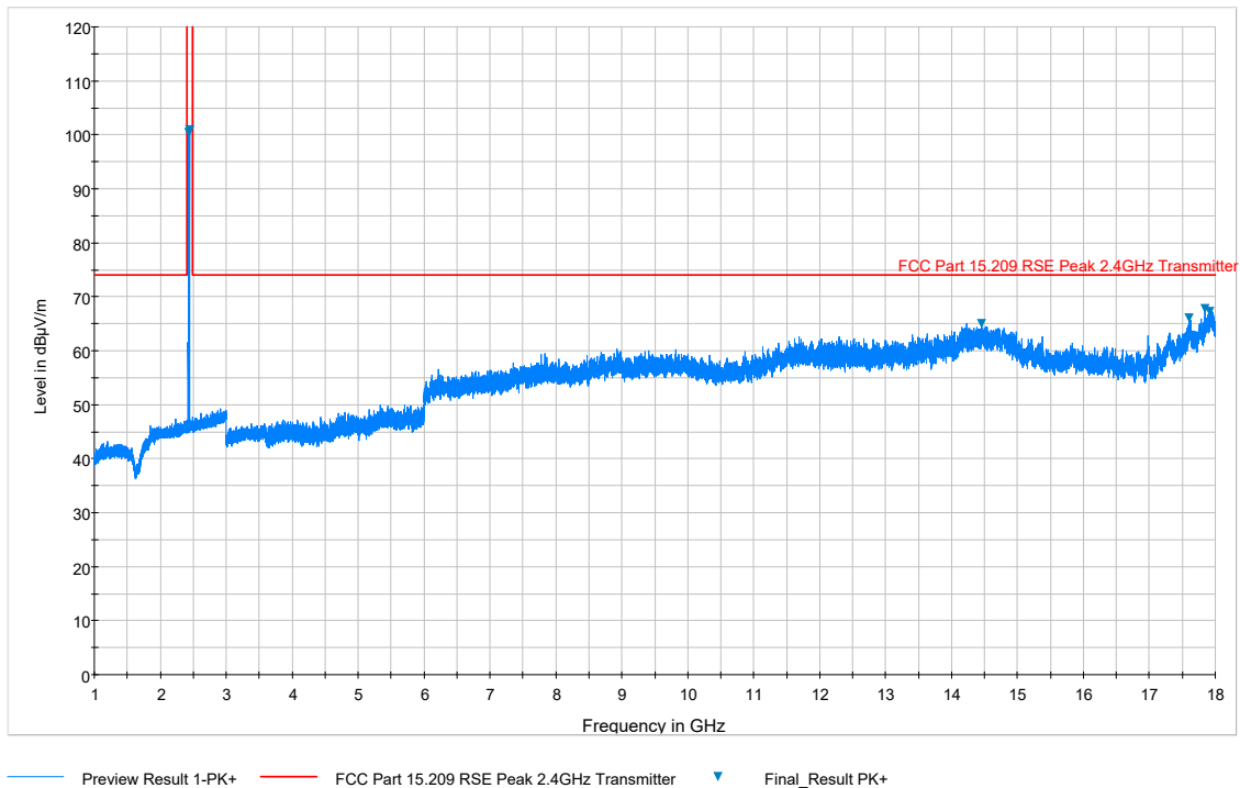
Plot 7-44. Radiated Spurious Plot above 1GHz (BT – Ch. 39, Ant. Pol. H)
