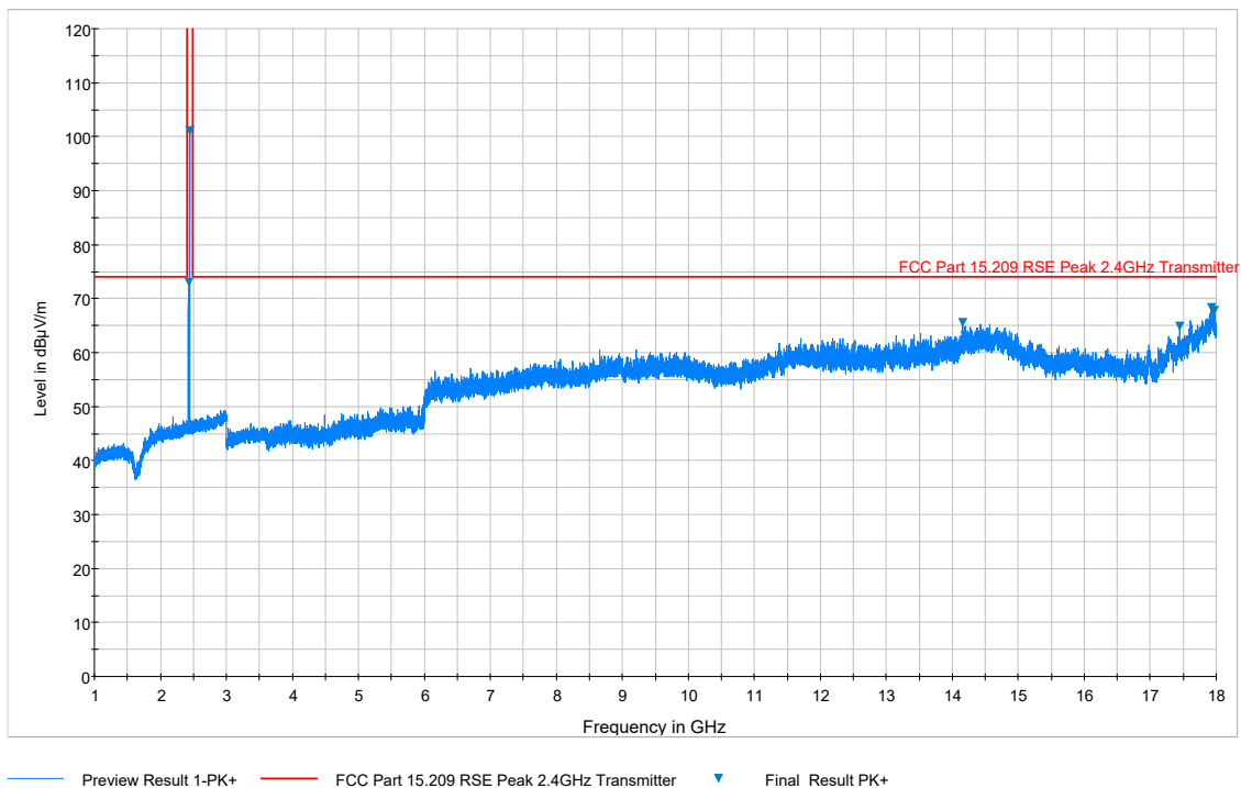
Plot 7-45. Radiated Spurious Plot above 1GHz (BT – Ch. 39, Ant. Pol. V)
