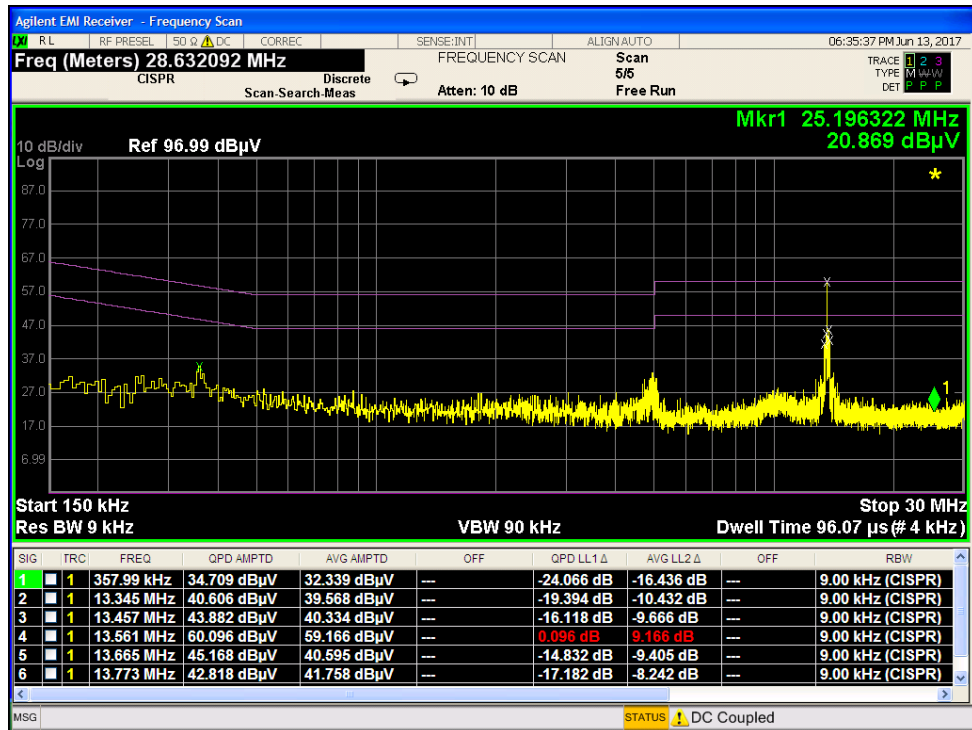
Plot 7-2. Line-Conducted Test Plot (with Antenna Connected) (N)
