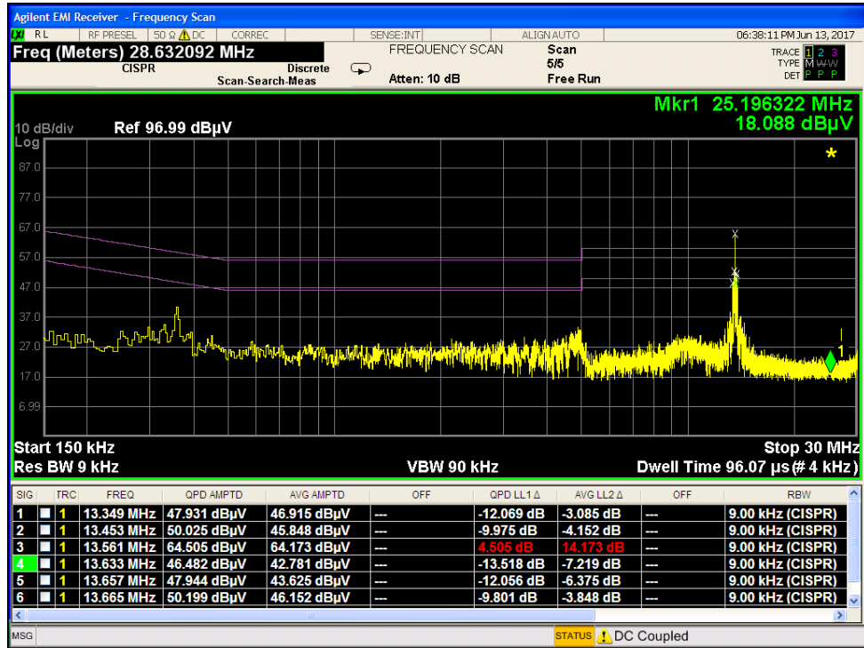
Plot 7-1. Line-Conducted Test Plot (with Antenna Connected) (L1)
