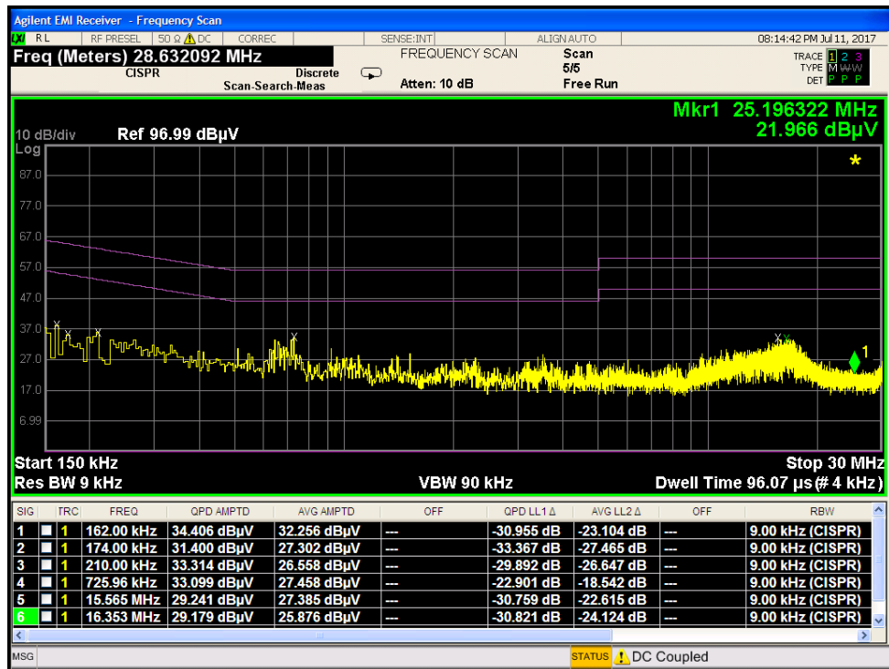
Plot 7-4. Line-Conducted Test Plot (With Antenna Terminated in 50 Ω) (N)
