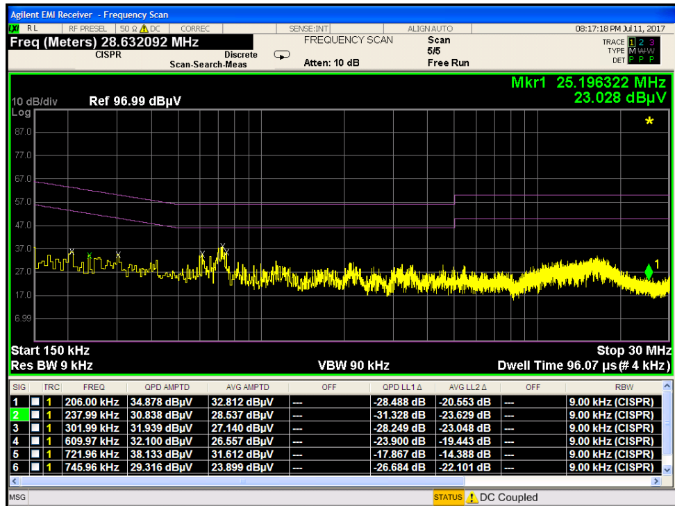
Plot 7-3. Line-Conducted Test Plot (With Antenna Terminated in 50 Ω) (L1)
