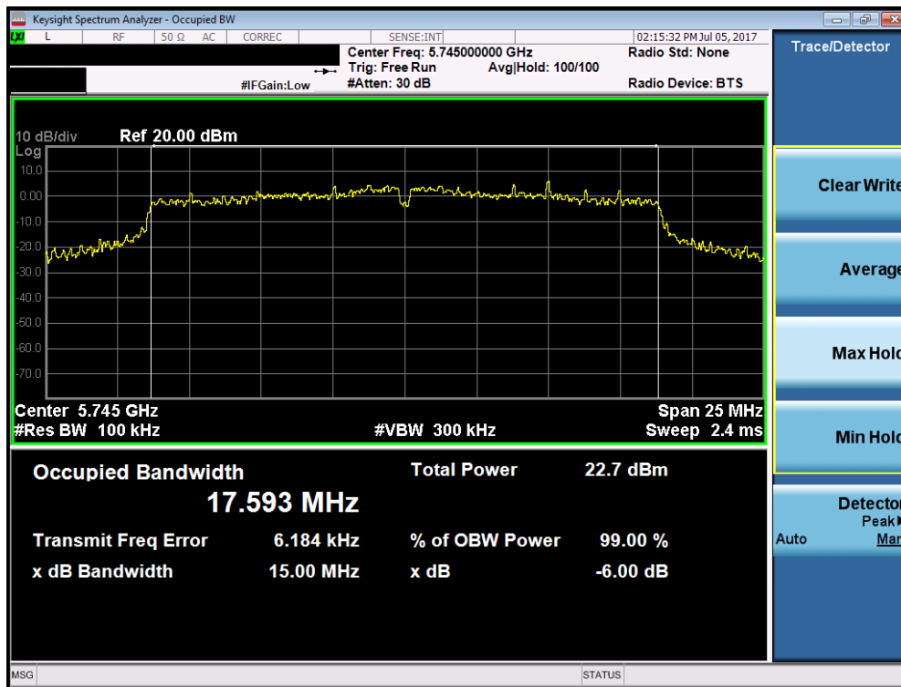
Plot 7-71. 6dB Bandwidth Plot (20MHz BW 802.11n (UNII Band 3) – Ch. 149)
