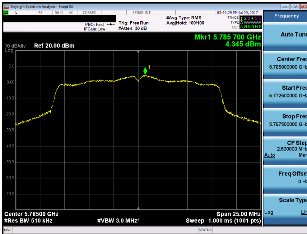
Plot 7-107. Power Spectral Density Plot (802.11a (UNII Band 3) – Ch. 157)
