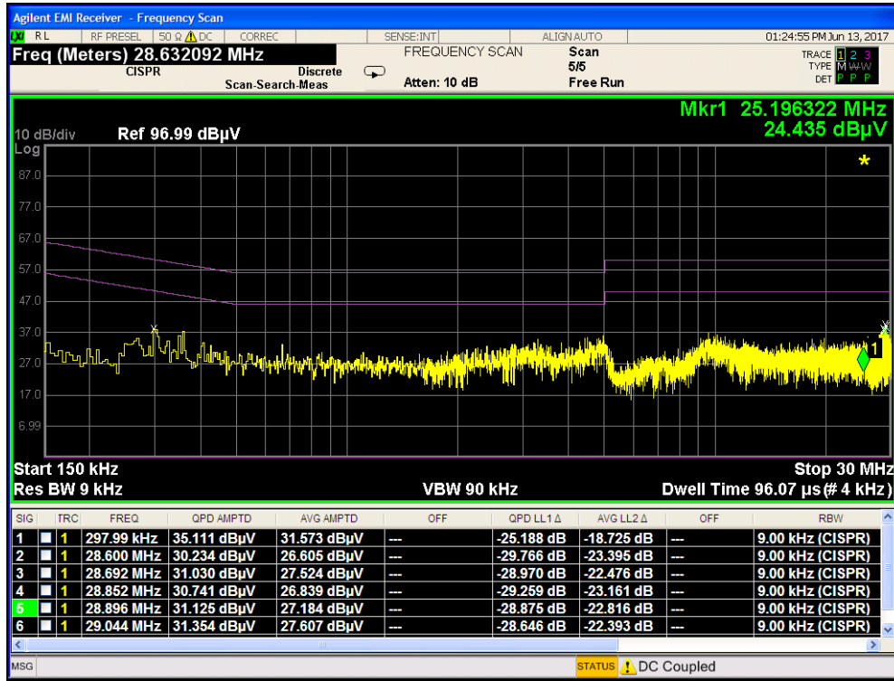
Plot 7-233. Line Conducted Plot with 802.11a UNII Band 1 (L1)
