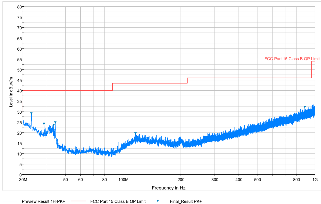
Plot 7-229. Radiated Spurious Plot below 1GHz (802.11a – U3 Ch. 157, Ant. Pol. H)
