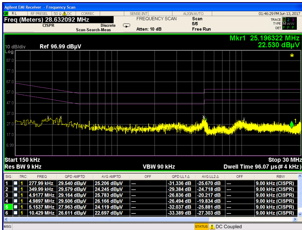
Plot 7-240. Line Conducted Plot with 802.11a UNII Band 3 (N)
