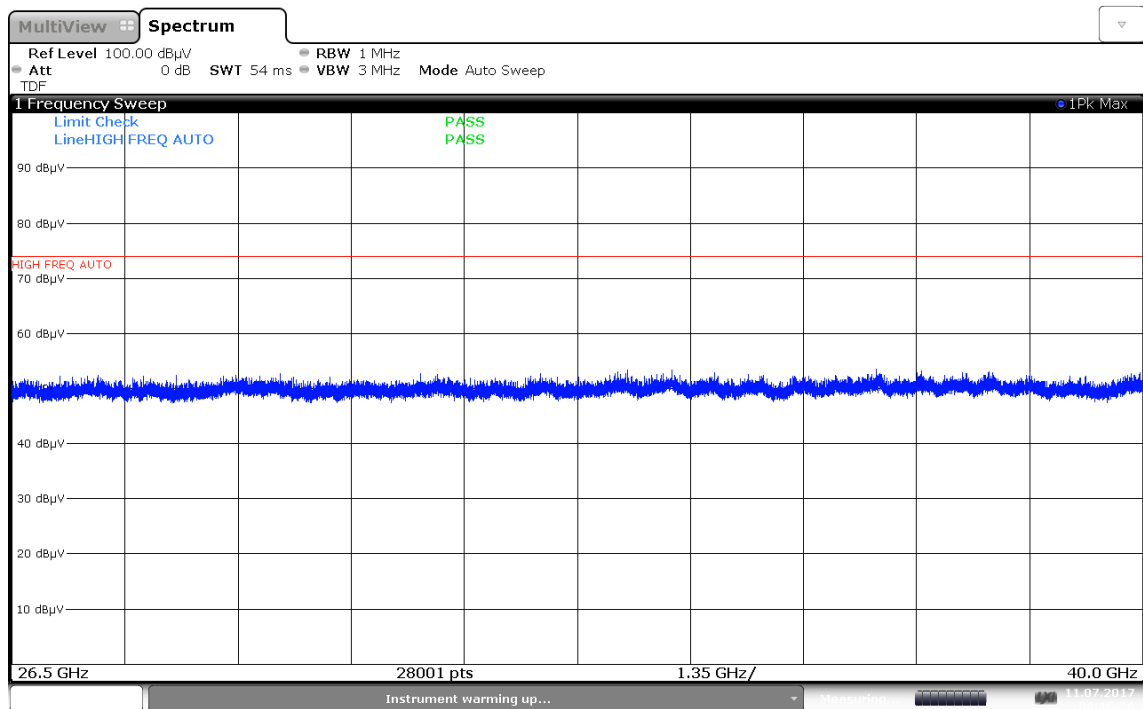
Plot 7-180. Radiated Spurious Plot 26.5-40GHz (2.4GHz – 5GHz, Ant. Pol. H)
