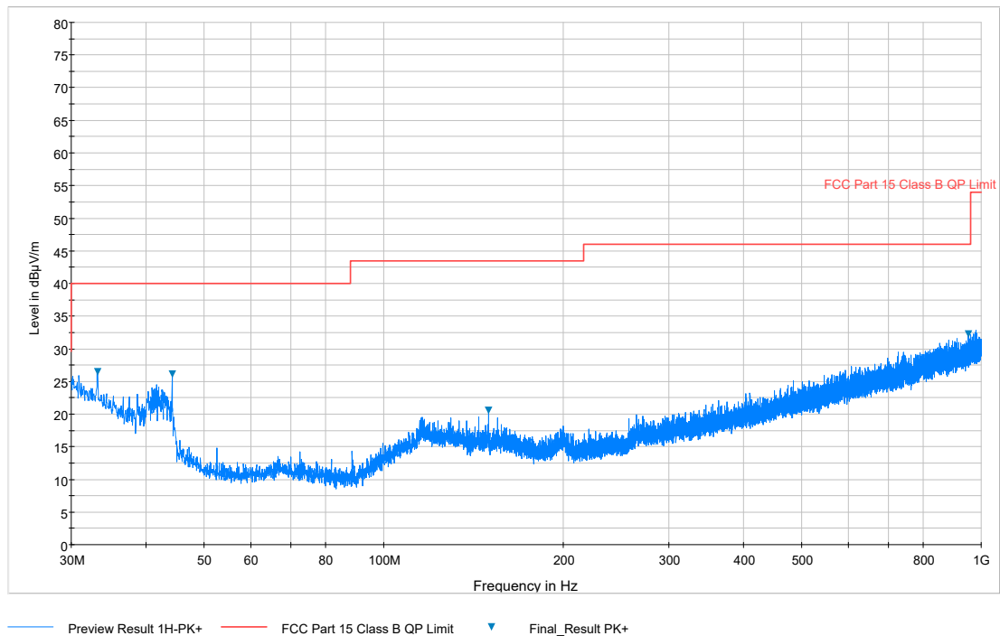
Plot 7-230. Radiated Spurious Plot below 1GHz (802.11a – U3 Ch. 157, Ant. Pol. V)
