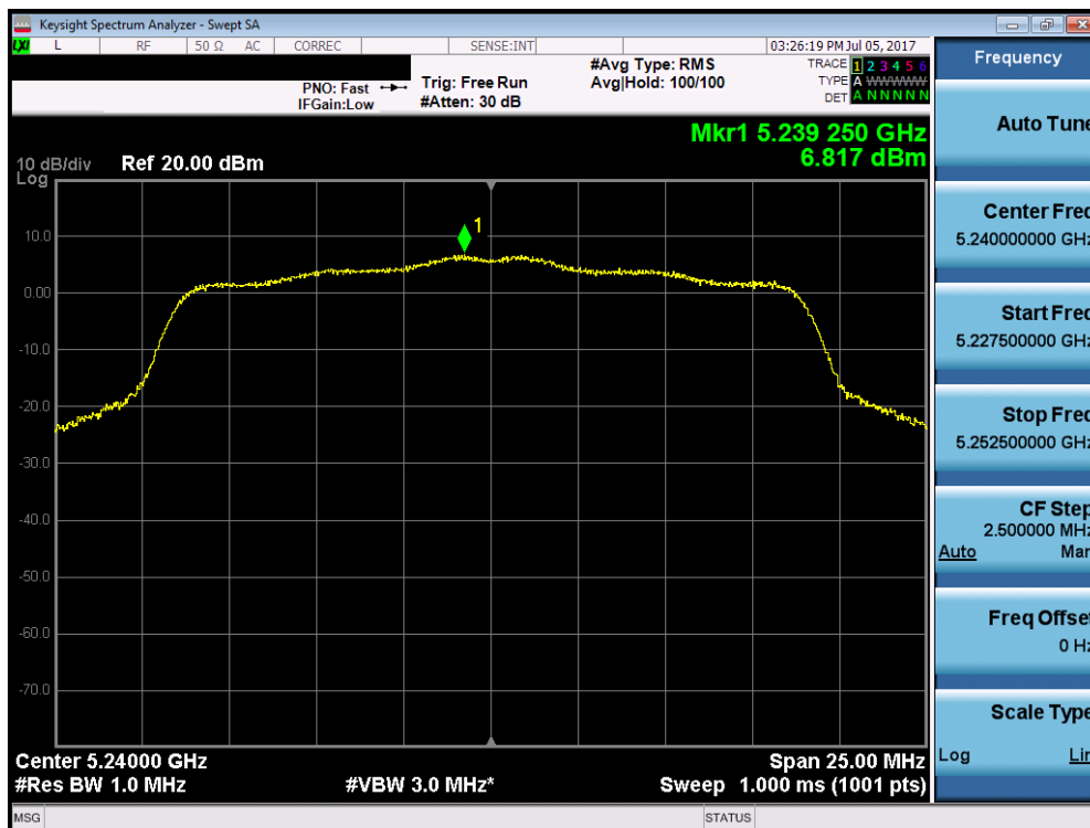
Plot 7-120. Power Spectral Density Plot (20MHz BW 802.11n (UNII Band 1) – Ch. 48)
