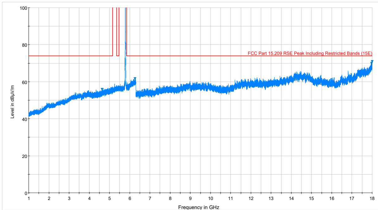
Plot 7-160. Radiated Spurious Plot above 1GHz (802.11a – U3 Ch. 157, Ant. Pol. V)
