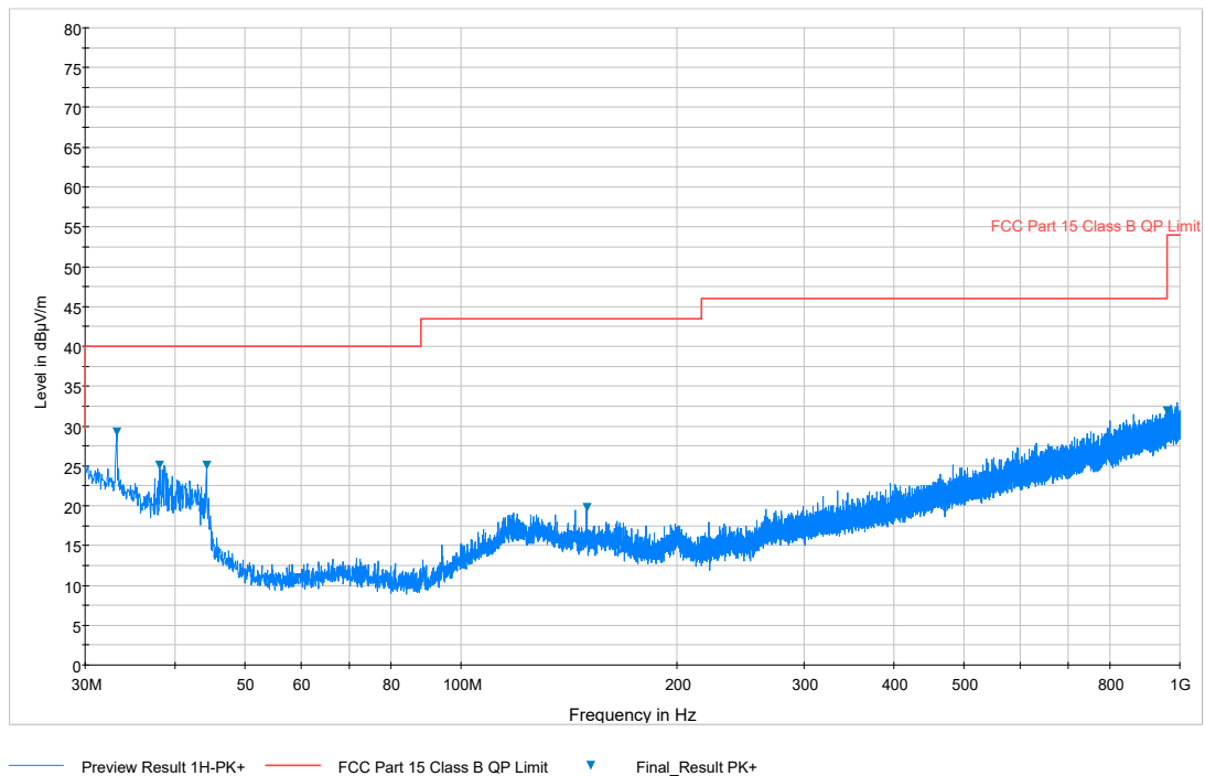
Plot 7-90. Radiated Spurious Plot below 1GHz (Pol. V)
