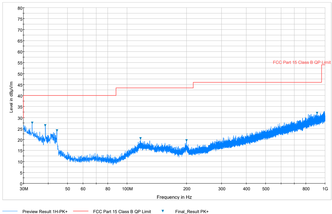
Plot 7-88. Radiated Spurious Plot below 1GHz (Pol. V)
