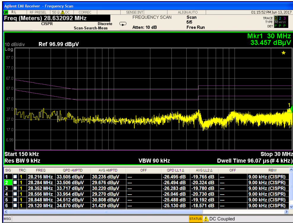
Plot 7-91. Line Conducted Plot with 802.11b (L1)
