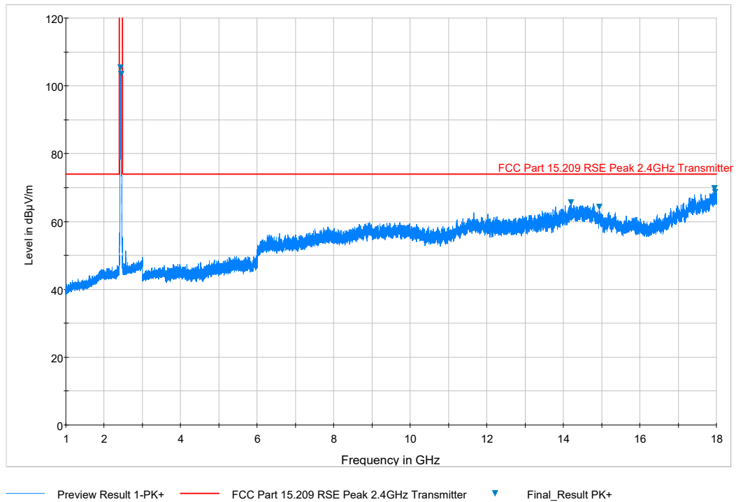
Plot 7-71. Radiated Spurious Plot above 1GHz (802.11b – Ch. 6, Ant. Pol. H)
