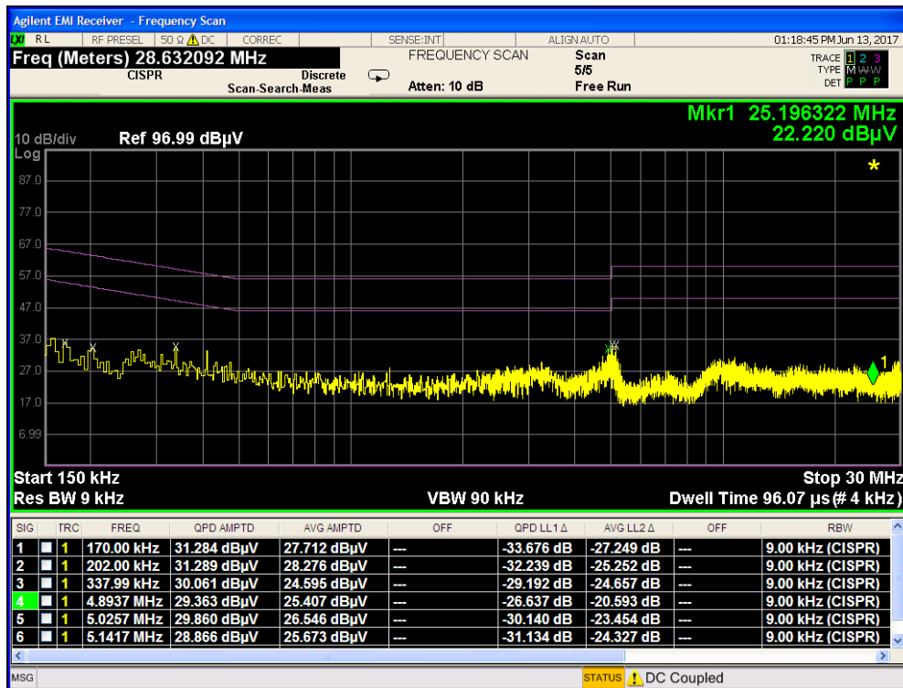
Plot 7-92. Line Conducted Plot with 802.11b (N)
