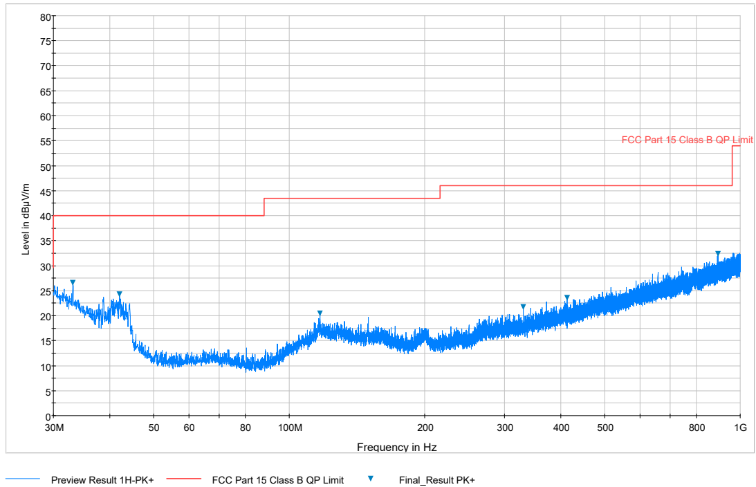
Plot 7-87. Radiated Spurious Plot below 1GHz (Pol. H)
