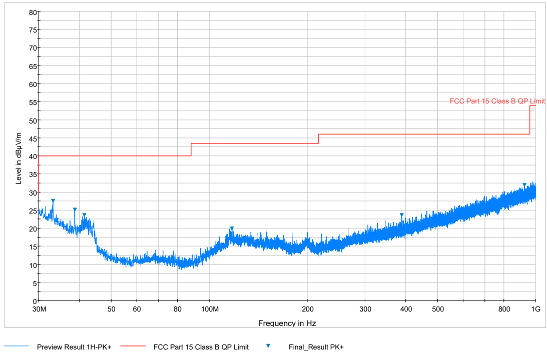
Plot 7-89. Radiated Spurious Plot below 1GHz (Pol. H)
