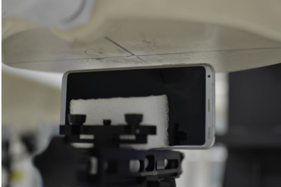
SAR Test Setup Photo 13: Left at 1.0 cm
