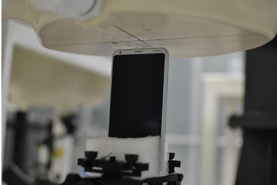
SAR Test Setup Photo 9: Top at 1.0 cm
