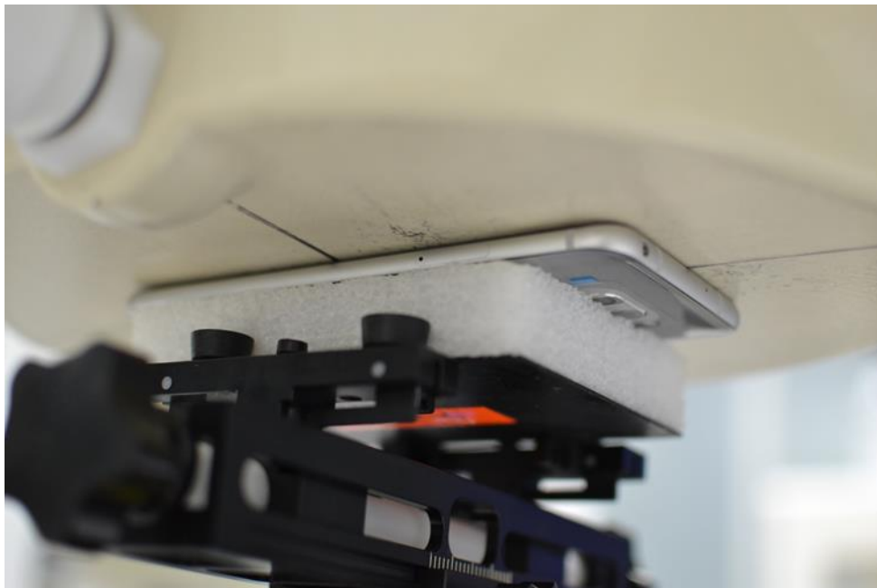
SAR Test Setup Photo 8: Front at 0.0 cm
