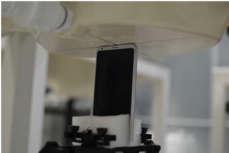
SAR Test Setup Photo 10: Top at 0.0 cm
