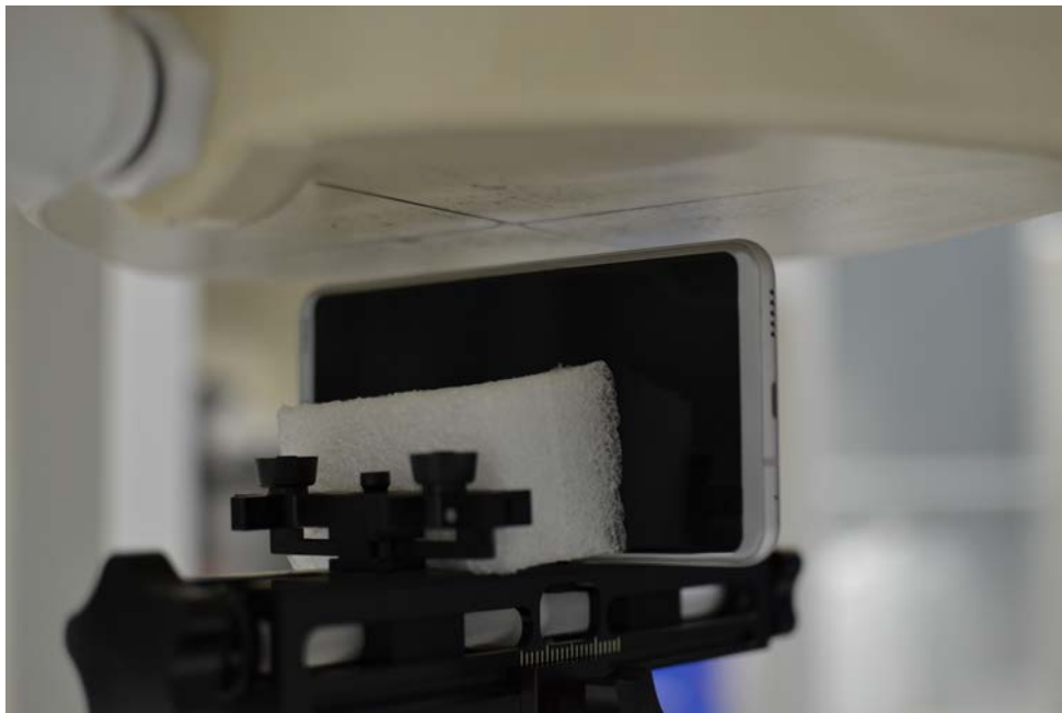
SAR Test Setup Photo 12: Right at 1.0 cm
