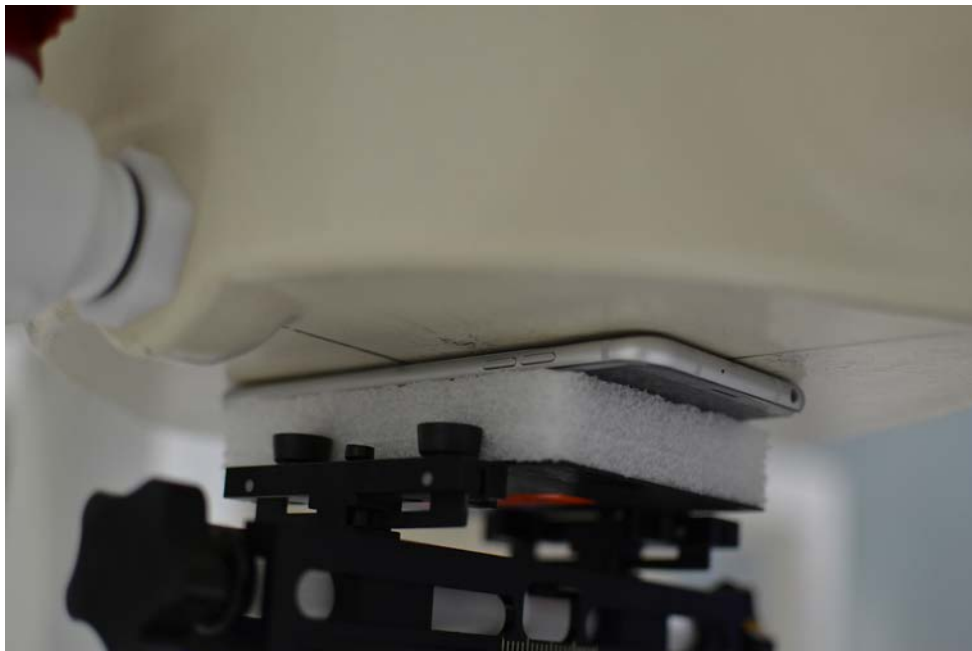
SAR Test Setup Photo 6: Back at 0.0 cm
