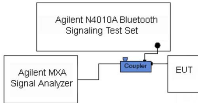
Figure 9-4 Power Measurement Setup
