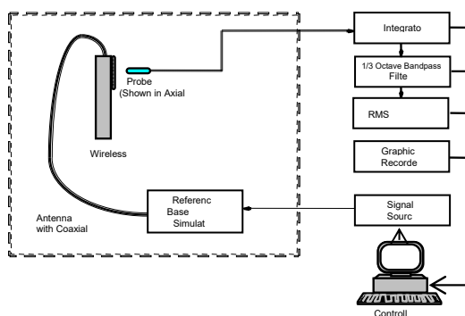
Figure 4-14 Audio Magnetic Field Test Setup
