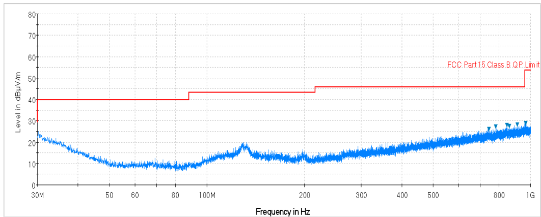
Plot 7-53. Radiated Spurious Plot below 1GHz (Pol. V)
