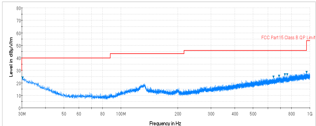
Plot 7-52. Radiated Spurious Plot below 1GHz (Pol. H)
