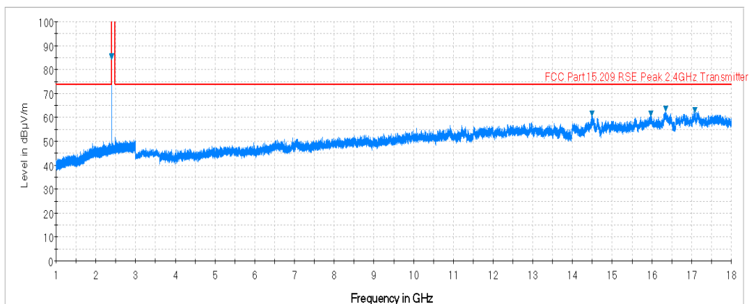
Plot 7-43. Radiated Spurious Plot above 1GHz (BT – Ch. 0, Ant. Pol. V)
