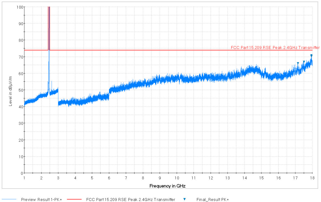
Plot 7-42. Radiated Spurious Plot above 1GHz (802.11b – Ch. 11, Ant. Pol. V)
