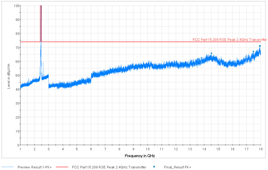
Plot 7-41. Radiated Spurious Plot above 1GHz (802.11b – Ch. 11, Ant. Pol. H)
