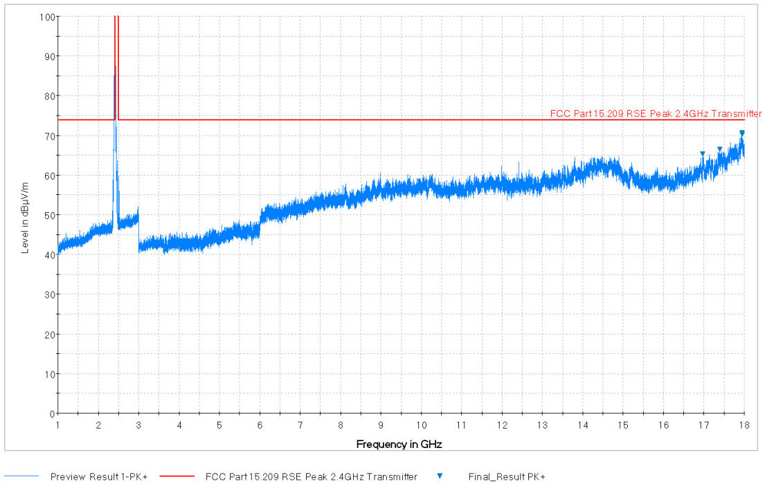
Plot 7-37. Radiated Spurious Plot above 1GHz (802.11b – Ch. 1, Ant. Pol. H)
