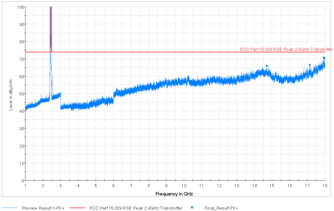
Plot 7-39. Radiated Spurious Plot above 1GHz (802.11b – Ch. 6, Ant. Pol. H)
