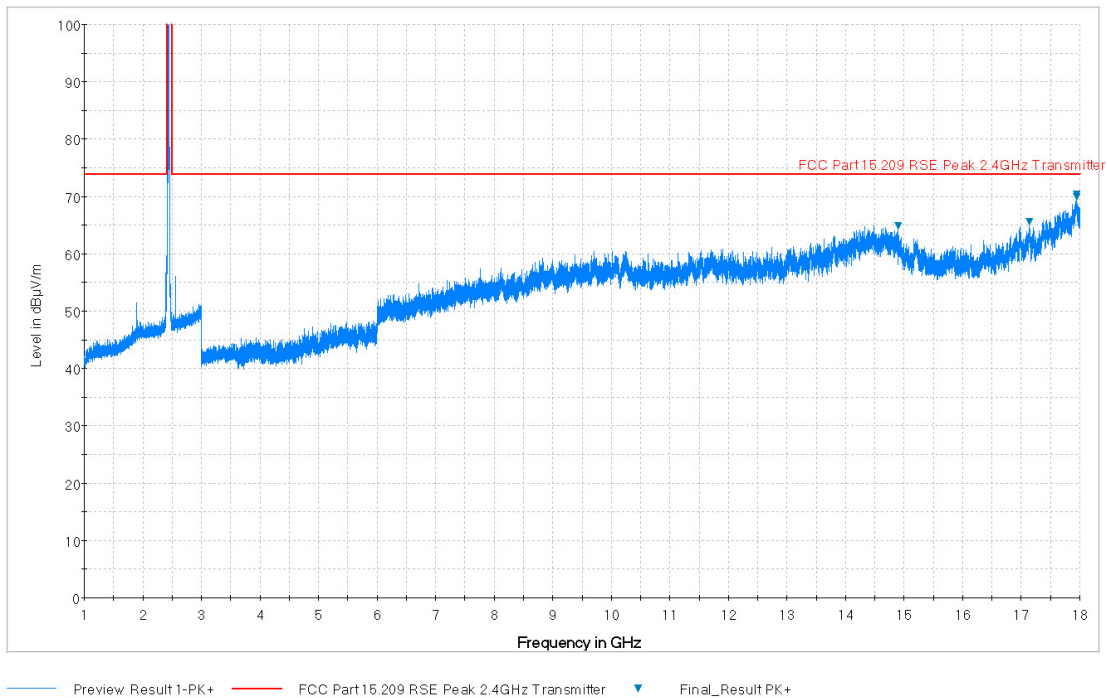
Plot 7-40. Radiated Spurious Plot above 1GHz (802.11b – Ch. 6, Ant. Pol. V)
