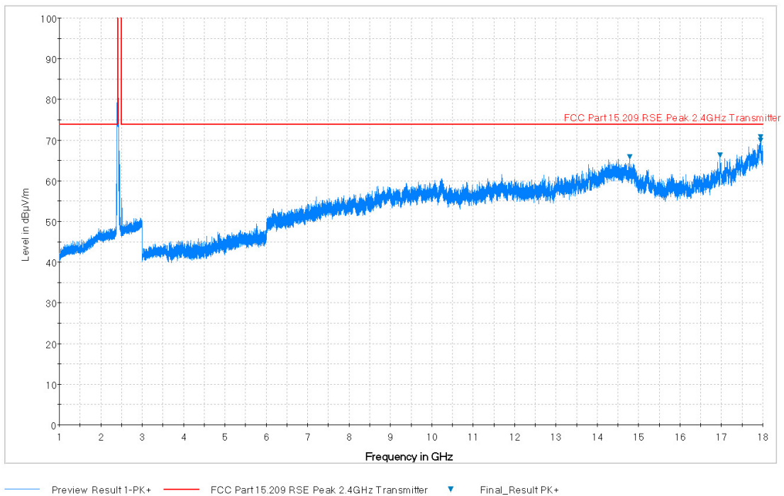
Plot 7-38. Radiated Spurious Plot above 1GHz (802.11b – Ch. 1, Ant. Pol. V)
