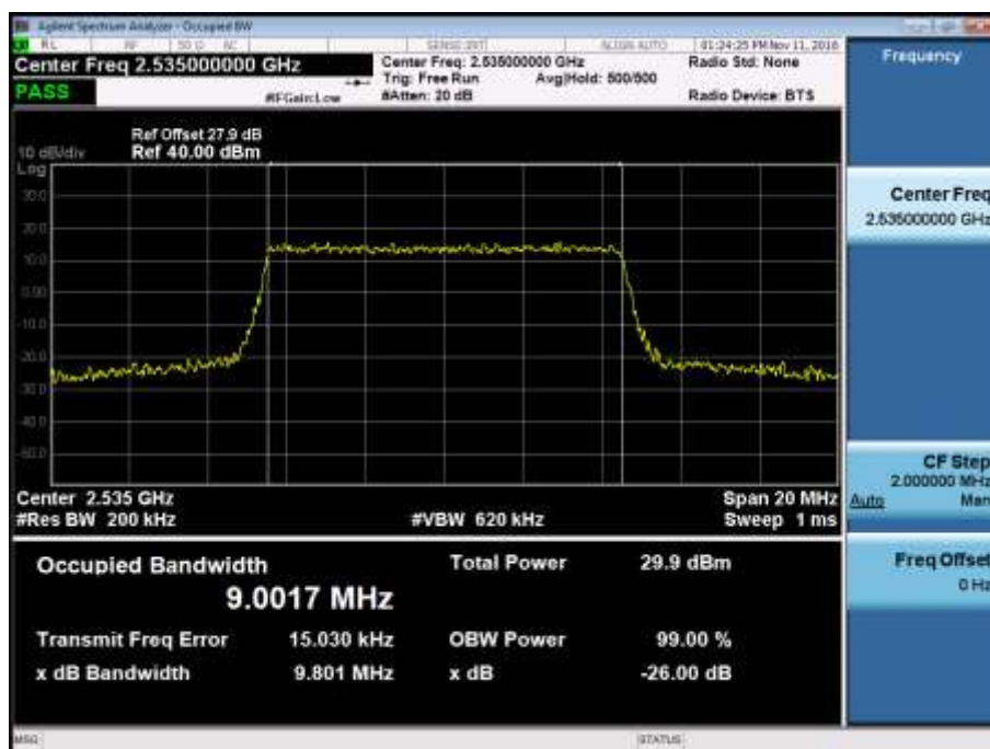
BAND7. Occupied Bandwidth Plot (10MHz Ch.21100 16-QAM RB 50)
