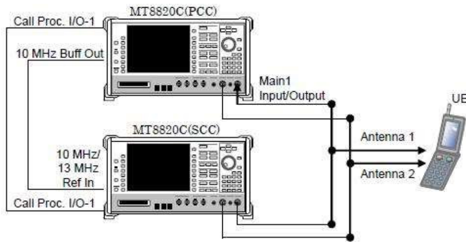
Power Measurement setup
