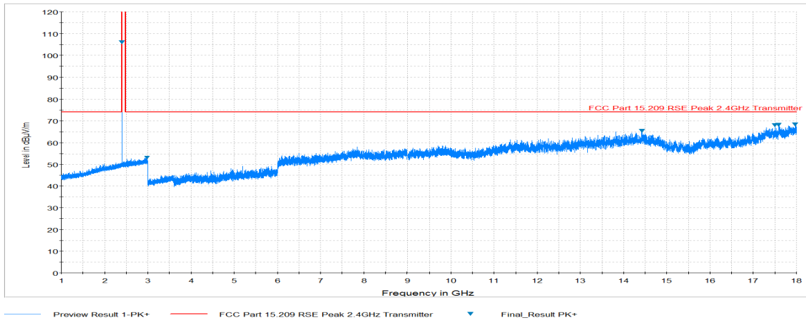
Plot 7-42. Radiated Spurious Plot above 1GHz (BT – Ch. 0, Ant. Pol. H)
