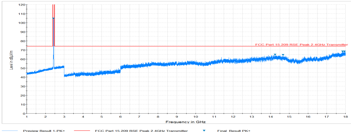
Plot 7-33. Radiated Spurious Plot above 1GHz (802.11b – Ch. 6, Ant. Pol. H)
