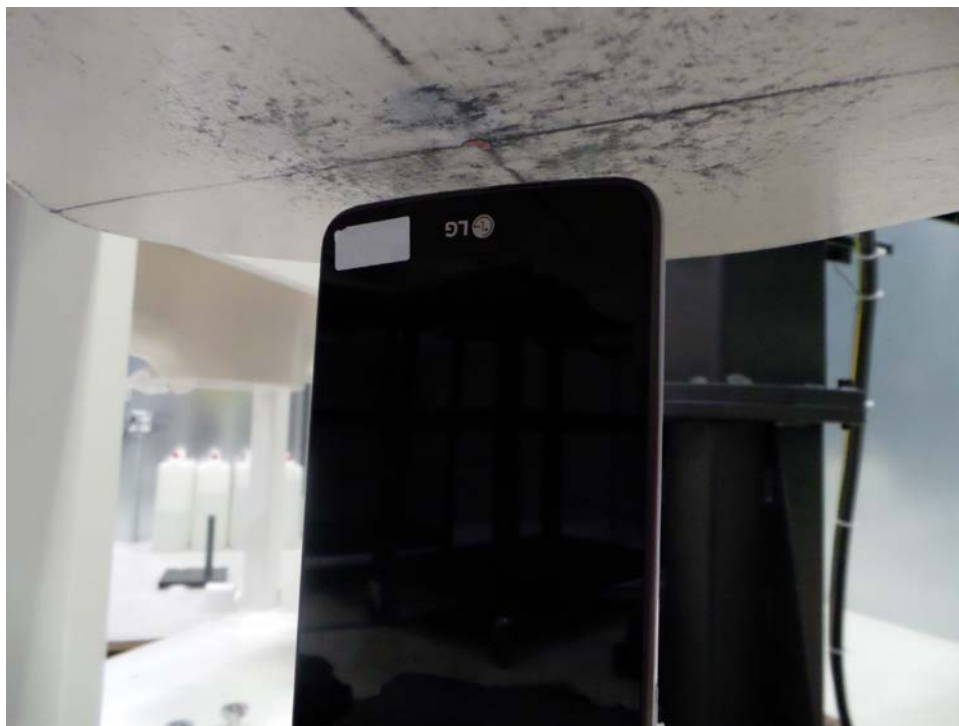
SAR Test Setup Photo 8: Bottom Edge at 1.0 cm
