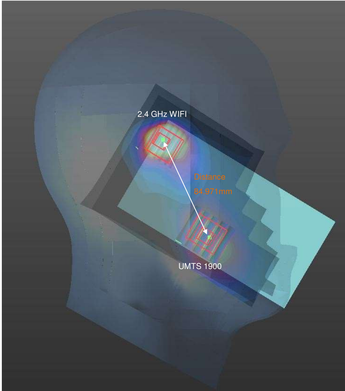
UMTS 1900&2.4GHz WiFi – Figure 1
