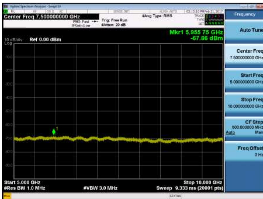
BAND 5. Conducted Spurious Plot _2 (20450ch_10MHz_QPSK_RB 1_0)
