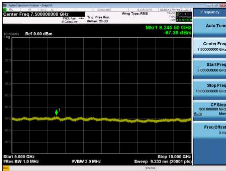
BAND 5. Conducted Spurious Plot _2 (20407ch_1.4MHz_QPSK_RB 1_0)
