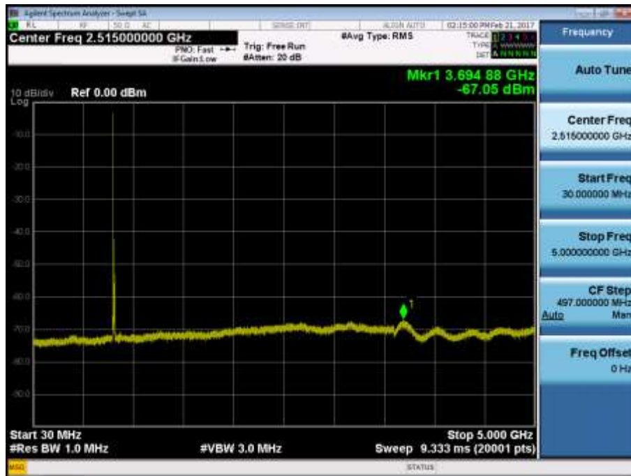
BAND 5. Conducted Spurious Plot _1 (20450ch_10MHz_QPSK_RB 1_0)
