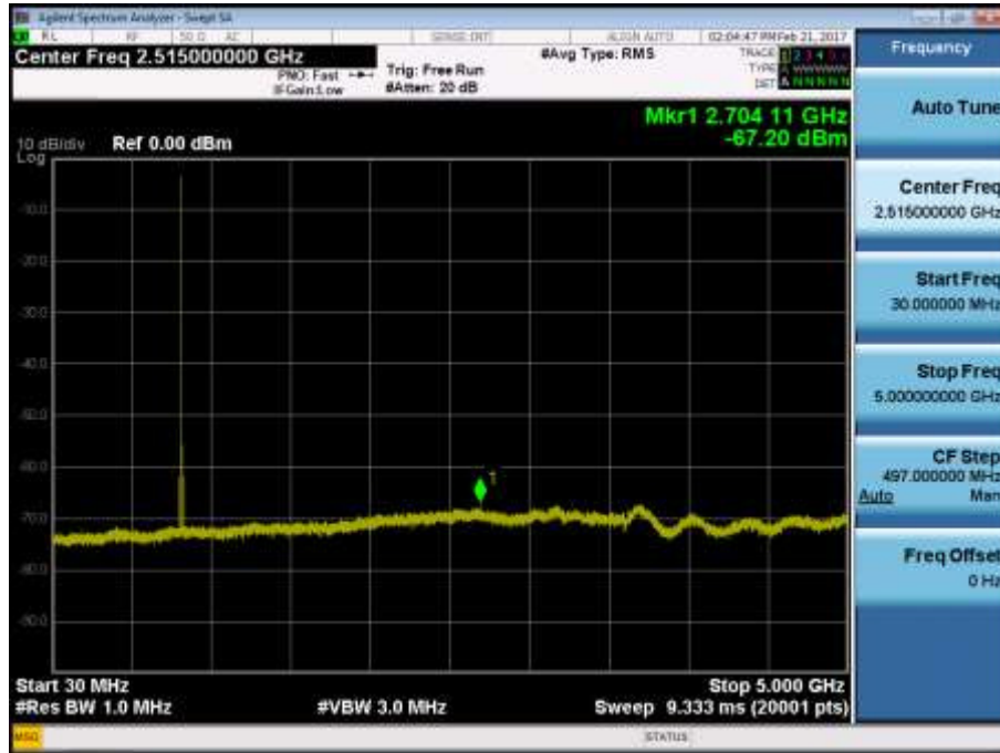
BAND 5. Conducted Spurious Plot _1 (20525ch_1.4MHz_QPSK_RB 1_0)
