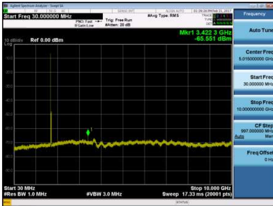
BAND 4. Conducted Spurious Plot_1 (20175ch_15MHz_QPSK_RB 1_0)
