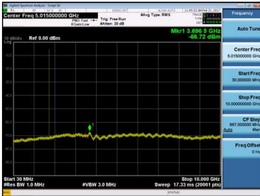
BAND 4. Conducted Spurious Plot_1 (20393ch_1.4MHz_QPSK_RB 1_0)
