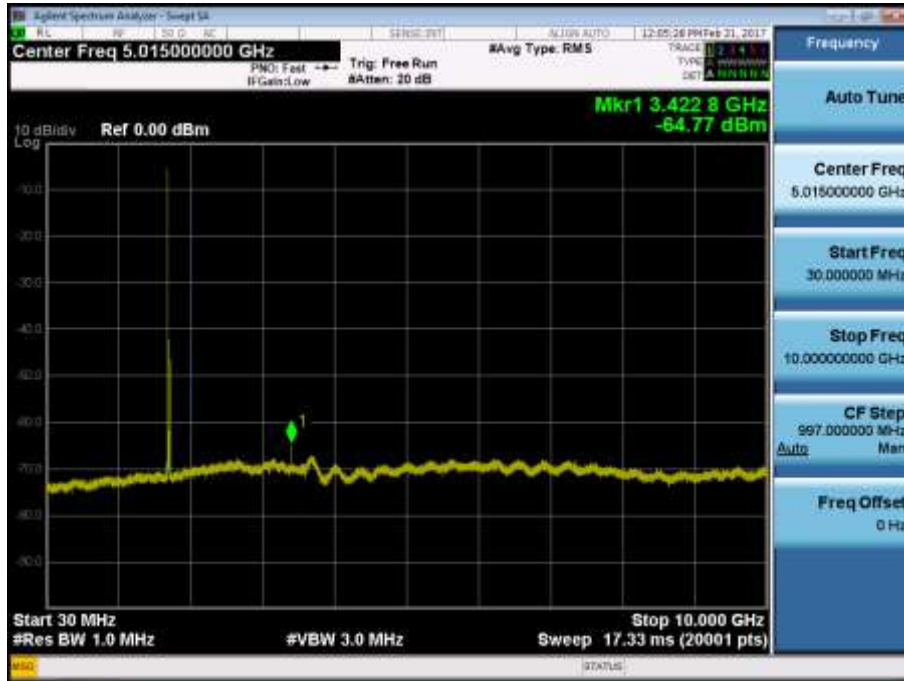
BAND 4. Conducted Spurious Plot_1 (20050ch_20MHz_QPSK_RB 1_0)
