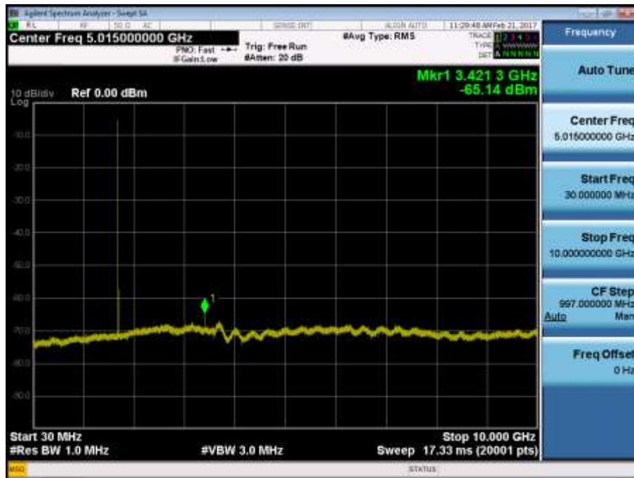
BAND 4. Conducted Spurious Plot_1 (19957ch_1.4MHz_QPSK_RB 1_0)
