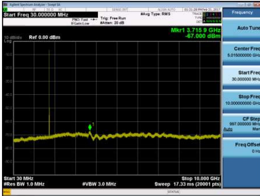
BAND 4. Conducted Spurious Plot_1 (20350ch_10MHz_QPSK_RB 1_0)
