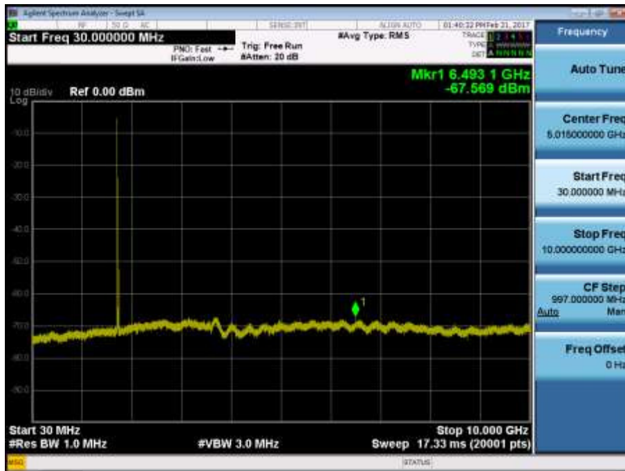
BAND 4. Conducted Spurious Plot_1 (20300ch_20MHz_QPSK_RB 1_0)
