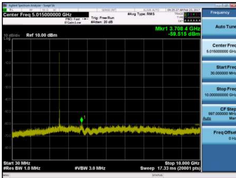
BAND7. Conducted Spurious Plot 1 (10MHz Ch.21100 QPSK RB 1, Offset 0)
