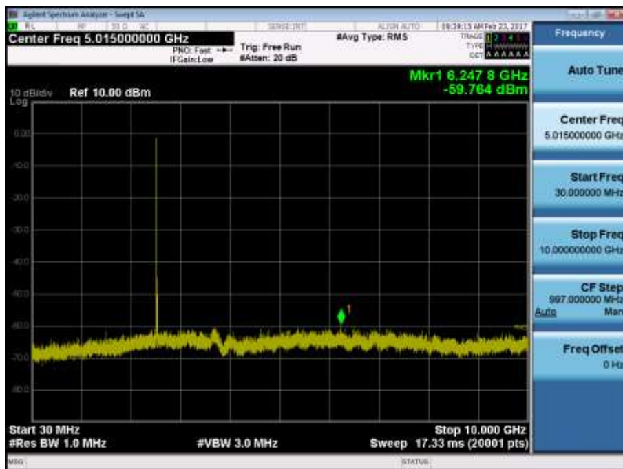
BAND7. Conducted Spurious Plot 1 (15MHz Ch.21100 QPSK RB 1, Offset 0)
