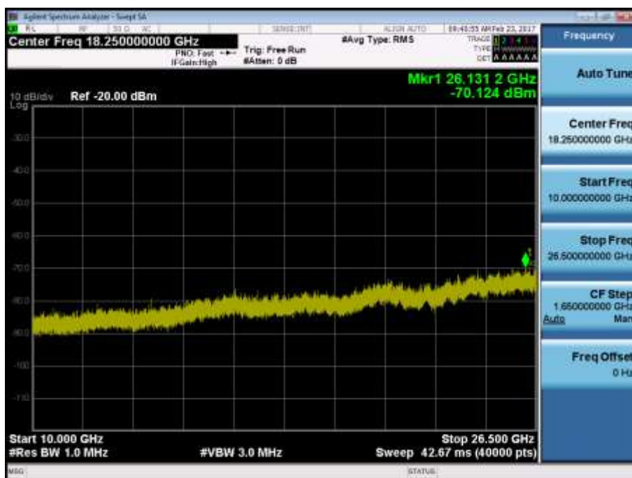
BAND7. Conducted Spurious Plot 2 (15MHz Ch.21375 QPSK RB 1, Offset 0)
