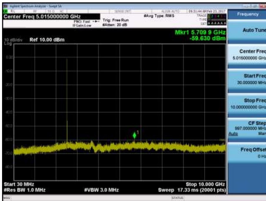
BAND7. Conducted Spurious Plot 1 (5MHz Ch.21100 QPSK RB 1, Offset 0)
