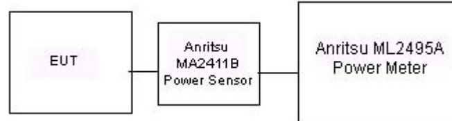
Figure 9-3 Power Measurement Setup
