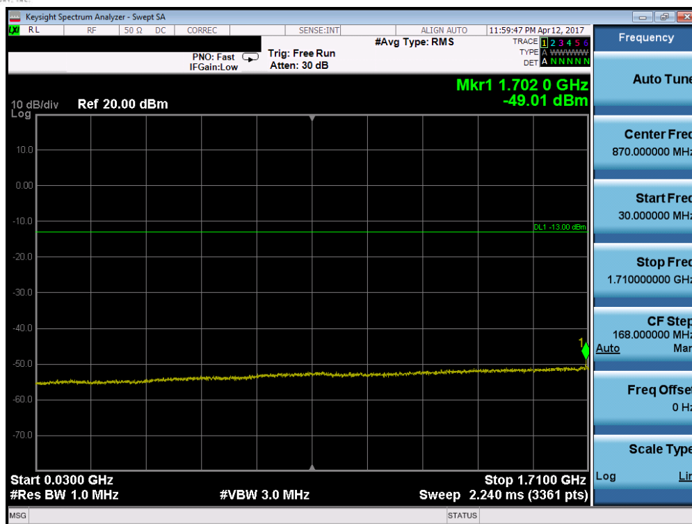
Plot 7-77. Conducted Spurious Plot (Band 4/66 – 20.0MHz QPSK – RB Size 1, RB Offset 0 – Mid Channel)
