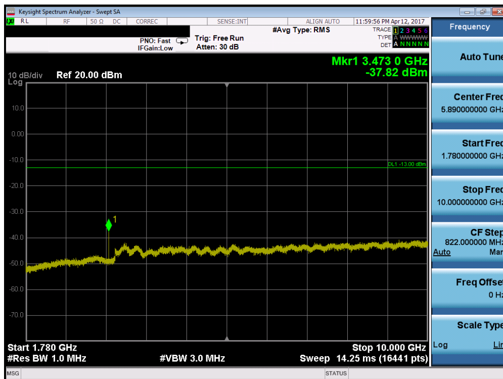
Plot 7-78. Conducted Spurious Plot (Band 4/66 – 20.0MHz QPSK – RB Size 1, RB Offset 0 – Mid Channel)
