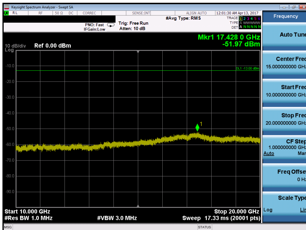
Plot 7-76. Conducted Spurious Plot (Band 4/66 – 20.0MHz QPSK – RB Size 1, RB Offset 0 – Low Channel)
