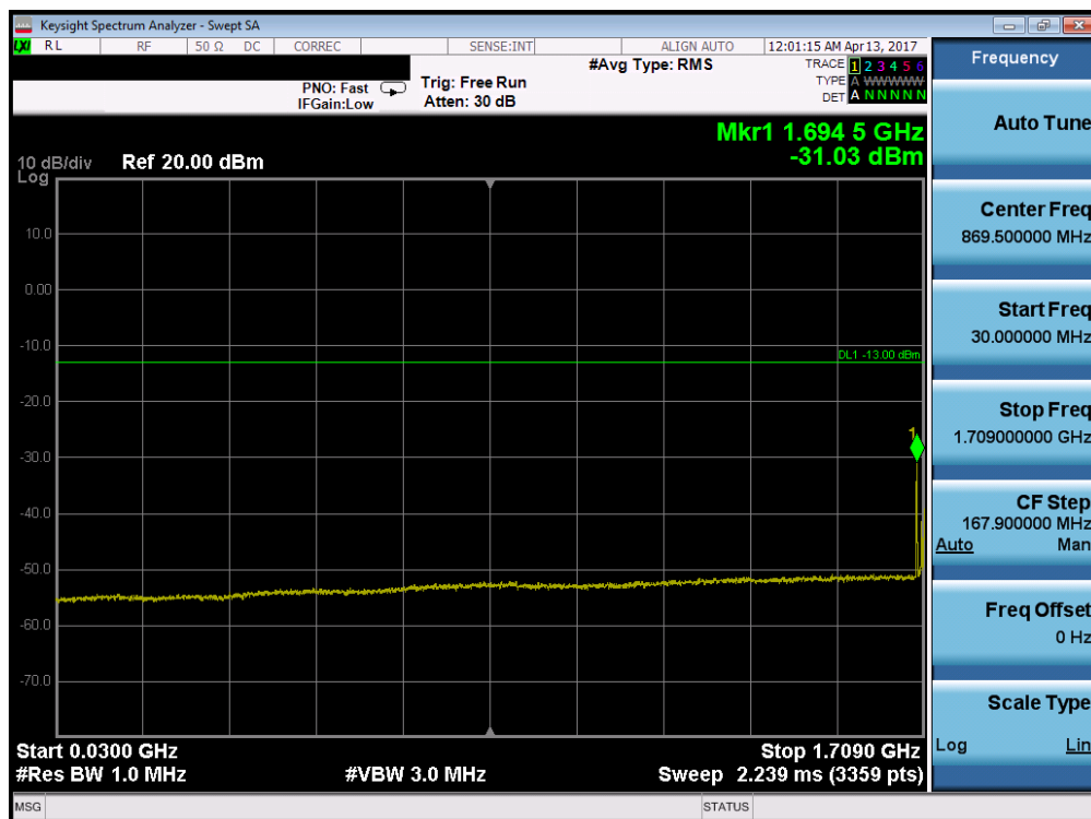
Plot 7-74. Conducted Spurious Plot (Band 4/66 – 20.0MHz QPSK – RB Size 1, RB Offset 0– Low Channel)
