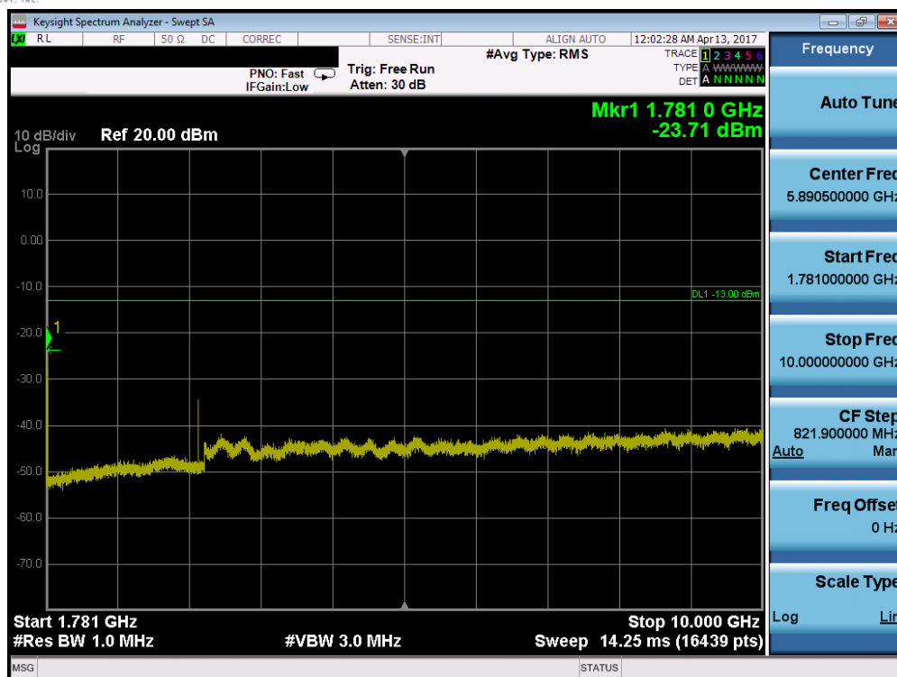
Plot 7-81. Conducted Spurious Plot (Band 4/66 – 20.0MHz QPSK – RB Size 1, RB Offset 0 – High Channel)
