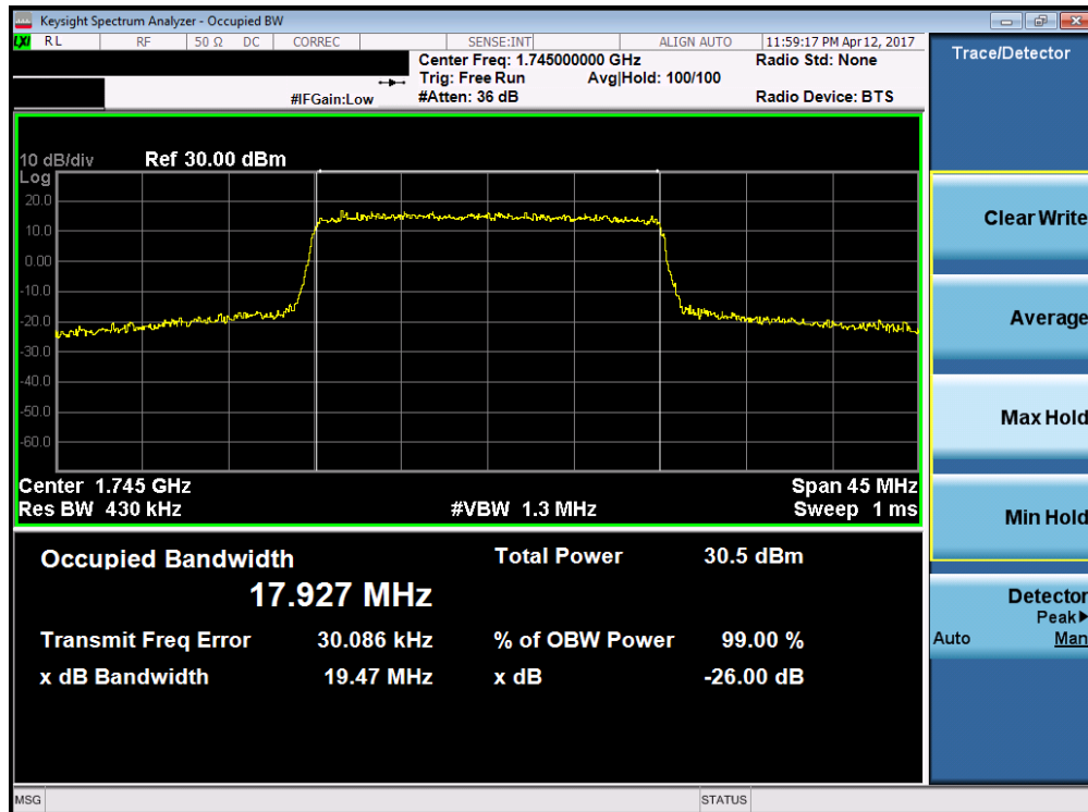
Plot 7-32. Occupied Bandwidth Plot (Band 4/66 – 20.0MHz 16-QAM – RB Size 100)
