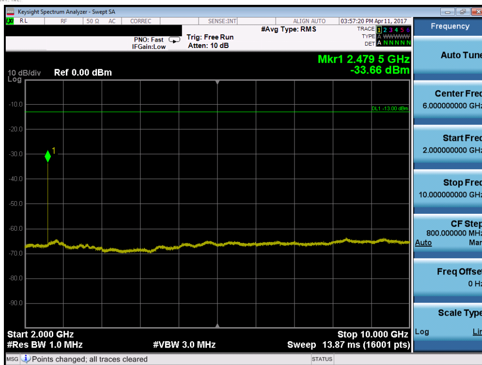
Plot 7-67. Conducted Spurious Plot (Band 5 – 5.0MHz QPSK – RB Size 1, RB Offset 0 – Low Channel)
