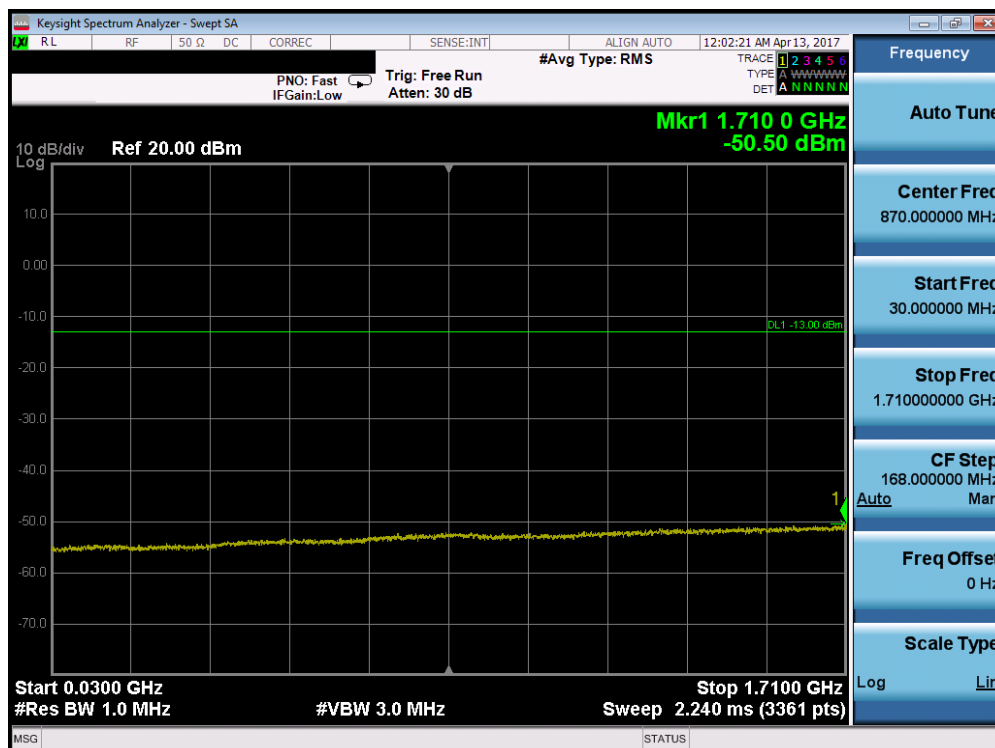
Plot 7-80. Conducted Spurious Plot (Band 4/66 – 20.0MHz QPSK – RB Size 1, RB Offset 0 – High Channel)
