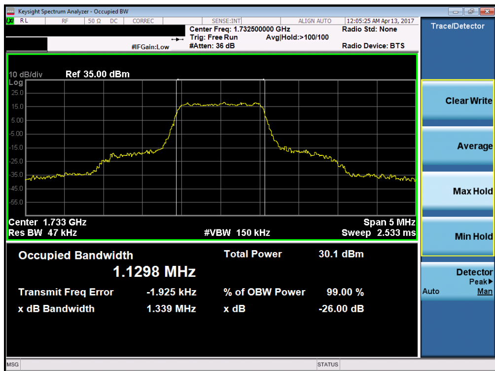
Plot 7-22. Occupied Bandwidth Plot (Band 4/66 – 1.4MHz 16-QAM – RB Size 6)
