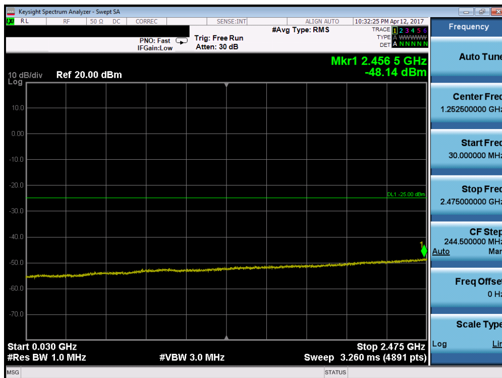
Plot 7-92. Conducted Spurious Plot (Band 7 – 20.0MHz QPSK – RB Size 1, RB Offset 0– Low Channel)
