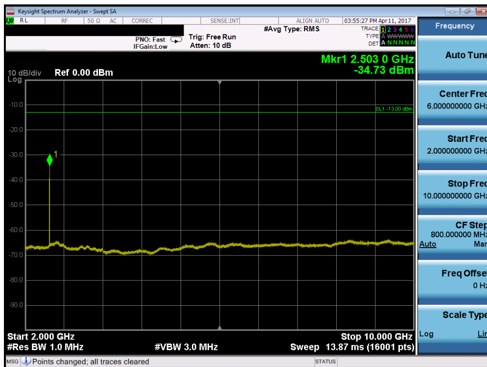
Plot 7-70. Conducted Spurious Plot (Band 5 – 5.0MHz QPSK – RB Size 1, RB Offset 0 – Mid Channel)
