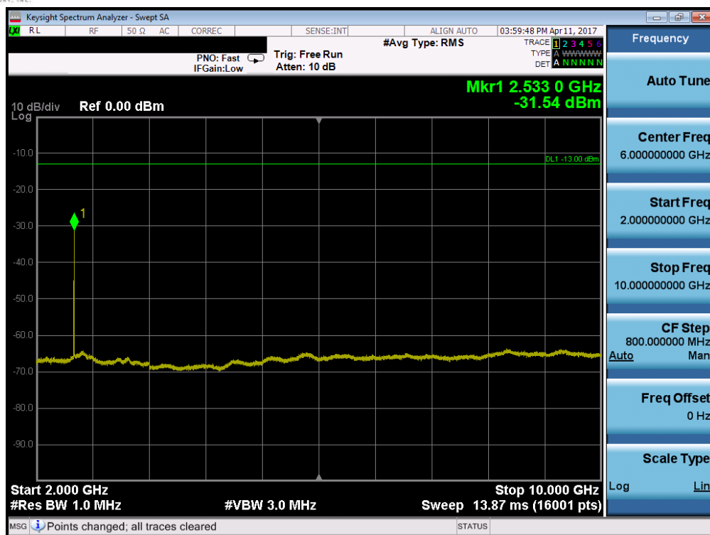
Plot 7-73. Conducted Spurious Plot (Band 5 – 5.0MHz QPSK – RB Size 1, RB Offset 0 – High Channel)
