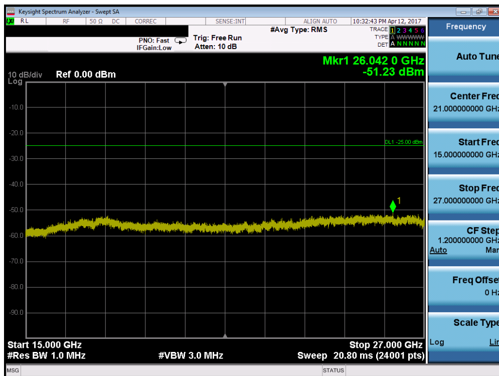
Plot 7-94. Conducted Spurious Plot (Band 7 – 20.0MHz QPSK – RB Size 1, RB Offset 0 – Low Channel)
