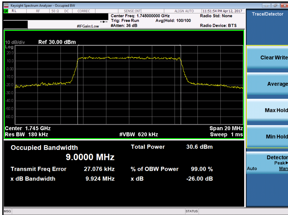
Plot 7-28. Occupied Bandwidth Plot (Band 4/66 – 10.0MHz 16-QAM – RB Size 50)
