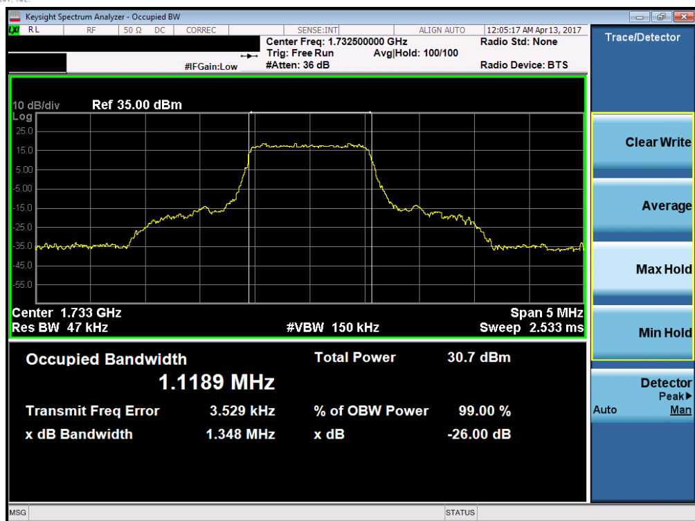
Plot 7-21. Occupied Bandwidth Plot (Band 4/66 – 1.4MHz QPSK – RB Size 6)
