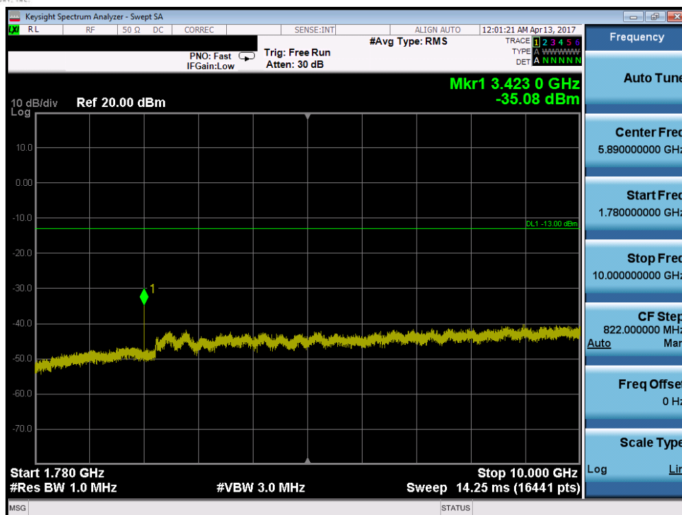
Plot 7-75. Conducted Spurious Plot (Band 4/66 – 20.0MHz QPSK – RB Size 1, RB Offset 0 – Low Channel)
