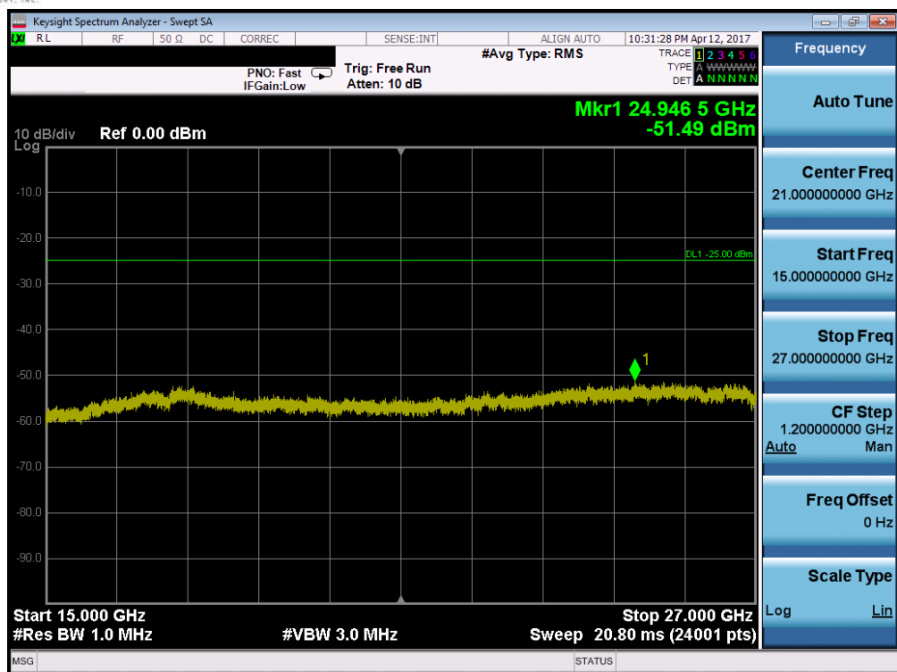
Plot 7-97. Conducted Spurious Plot (Band 7 – 20.0MHz QPSK – RB Size 1, RB Offset 0 – Mid Channel)
