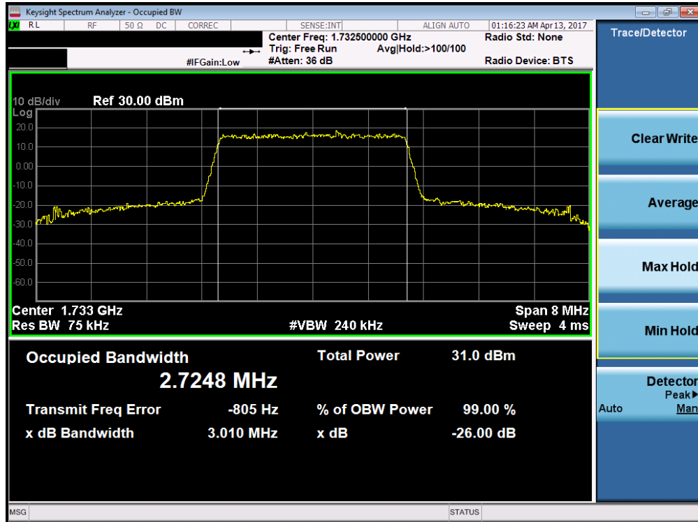
Plot 7-23. Occupied Bandwidth Plot (Band 4/66 – 3.0MHz QPSK – RB Size 15)
