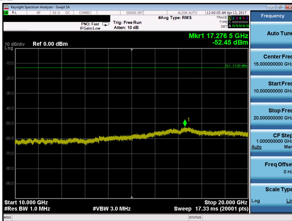
Plot 7-79. Conducted Spurious Plot (Band 4/66 – 20.0MHz QPSK – RB Size 1, RB Offset 0 – Mid Channel)
