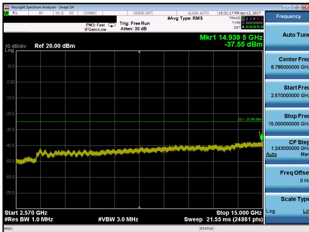
Plot 7-96. Conducted Spurious Plot (Band 7 – 20.0MHz QPSK – RB Size 1, RB Offset 0 – Mid Channel)
