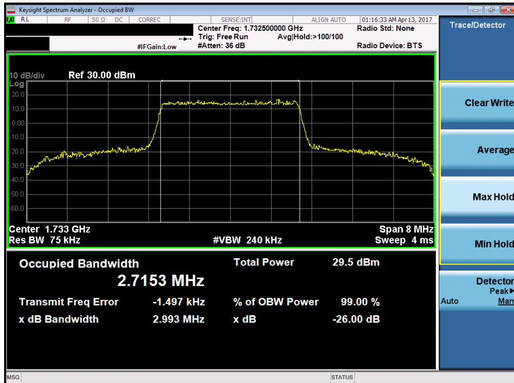
Plot 7-24. Occupied Bandwidth Plot (Band 4/66 – 3.0MHz 16-QAM – RB Size 15)
