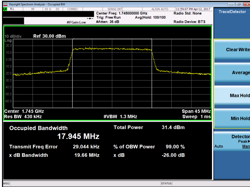
Plot 7-31. Occupied Bandwidth Plot (Band 4/66 – 20.0MHz QPSK – RB Size 100)
