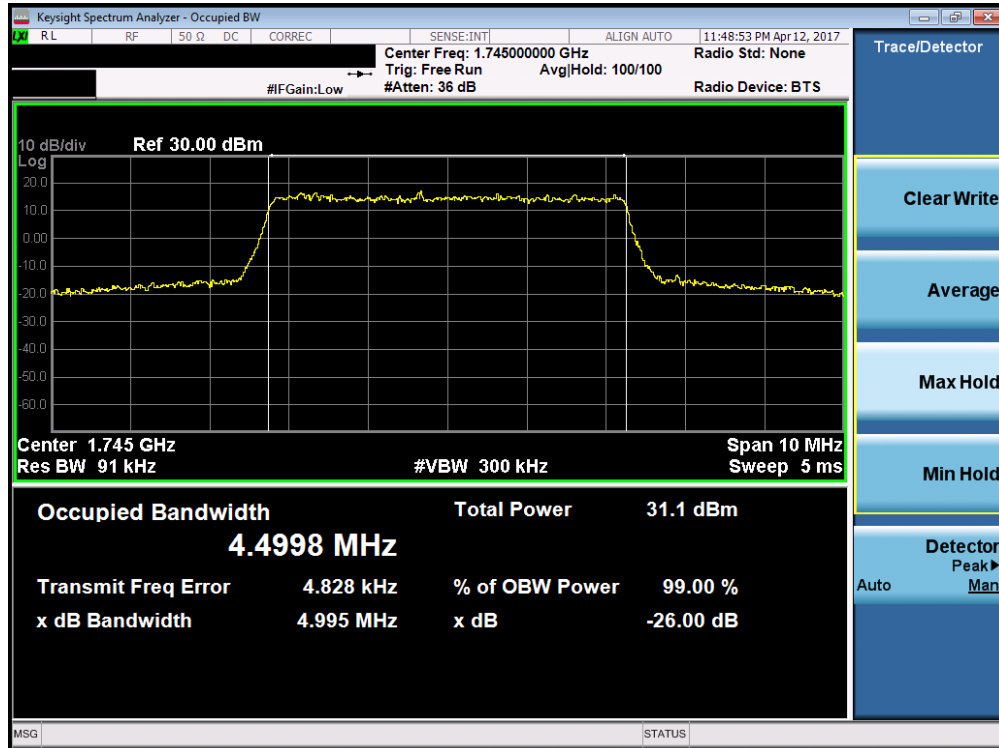
Plot 7-25. Occupied Bandwidth Plot (Band 4/66 – 5.0MHz QPSK – RB Size 25)
