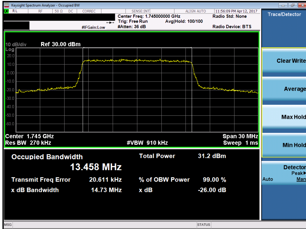
Plot 7-29. Occupied Bandwidth Plot (Band 4/66 – 15.0MHz QPSK – RB Size 75)
