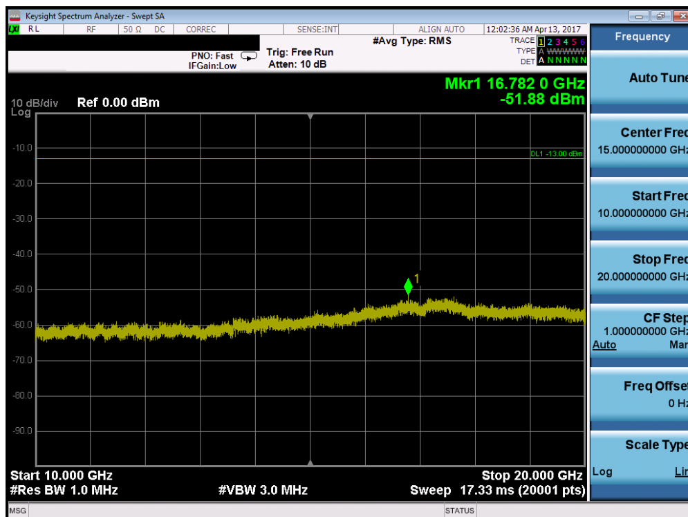
Plot 7-82. Conducted Spurious Plot (Band 4/66 – 20.0MHz QPSK – RB Size 1, RB Offset 0 – High Channel)
