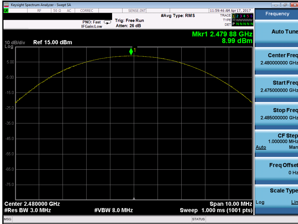
Plot 7-18. Peak Conducted Power (3Mbps – Ch. 78)
