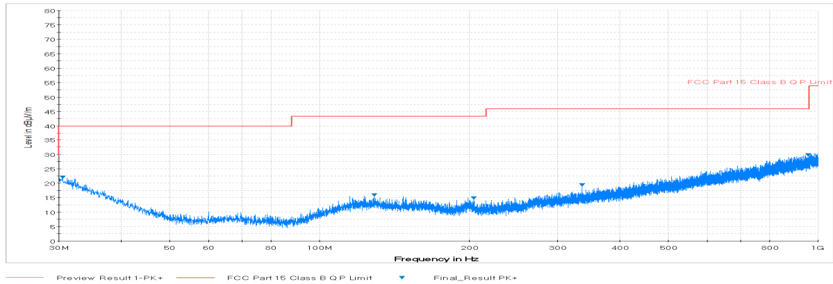
Plot 7-41. Radiated Spurious Plot below 1GHz (Pol. H)
