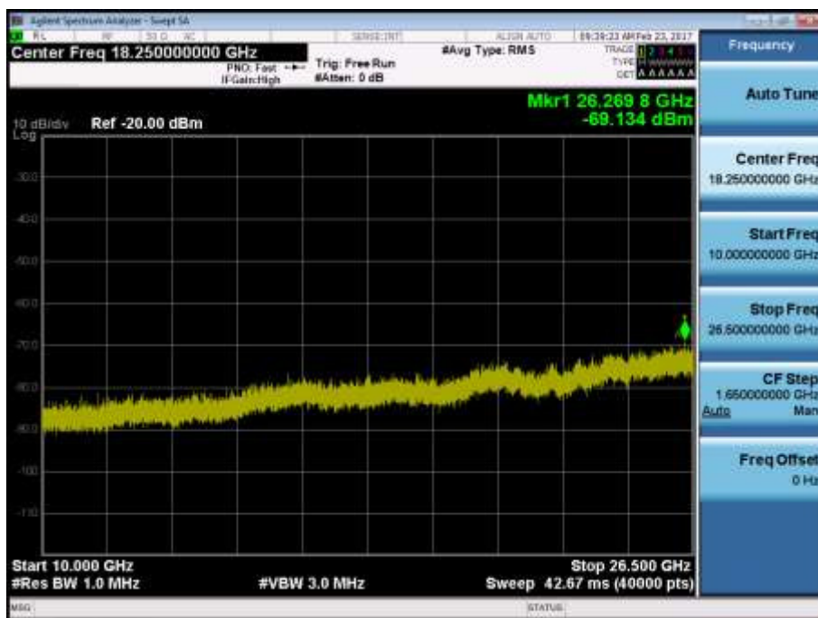
BAND7. Conducted Spurious Plot 2 (15MHz Ch.21100 QPSK RB 1, Offset 0)
