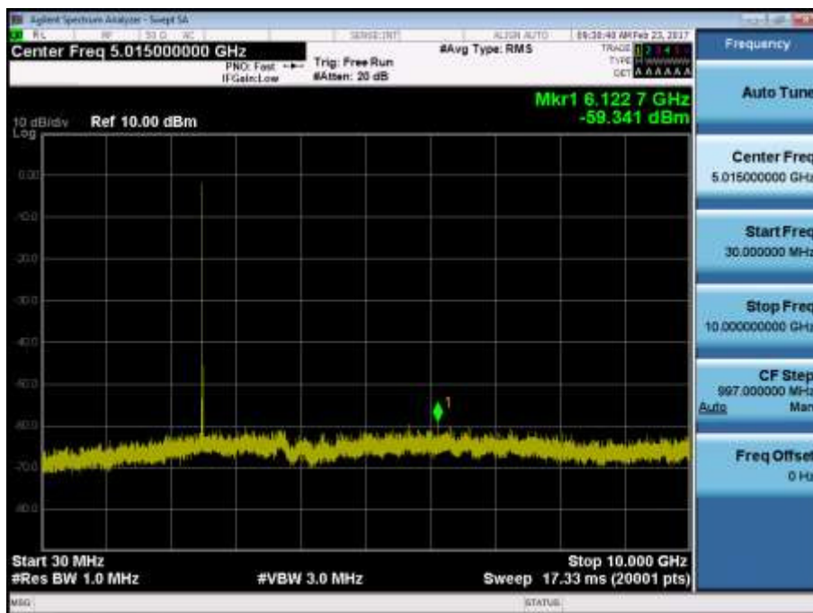
BAND7. Conducted Spurious Plot 1 (5MHz Ch.20775 QPSK RB 1, Offset 0)
