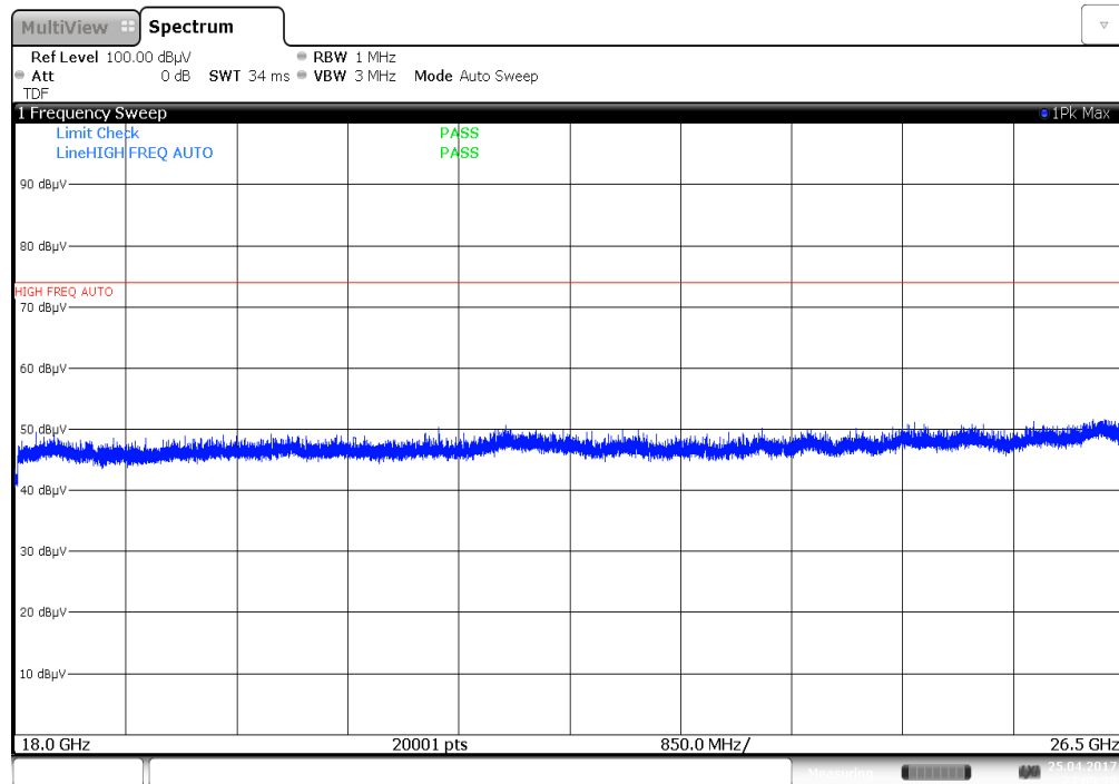
Plot 7-49. Radiated Spurious Plot above 18GHz (Pol. V)
