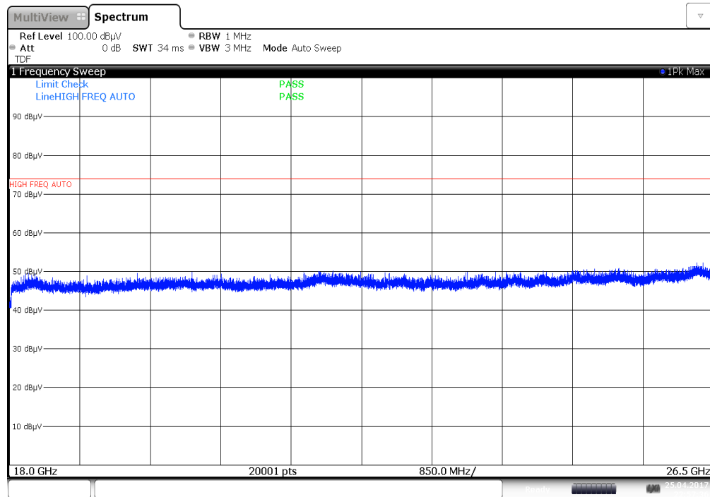
Plot 7-37. Radiated Spurious Plot above 18GHz (Pol. H)
