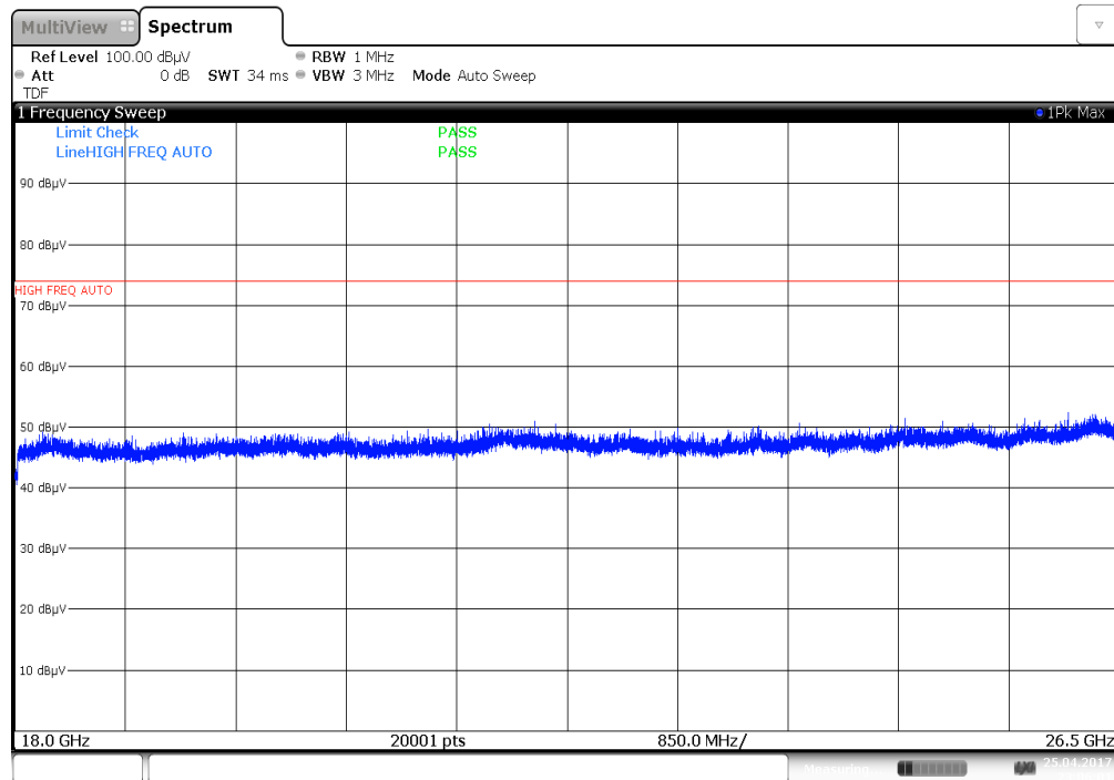
Plot 7-38. Radiated Spurious Plot above 18GHz (Pol. V)
