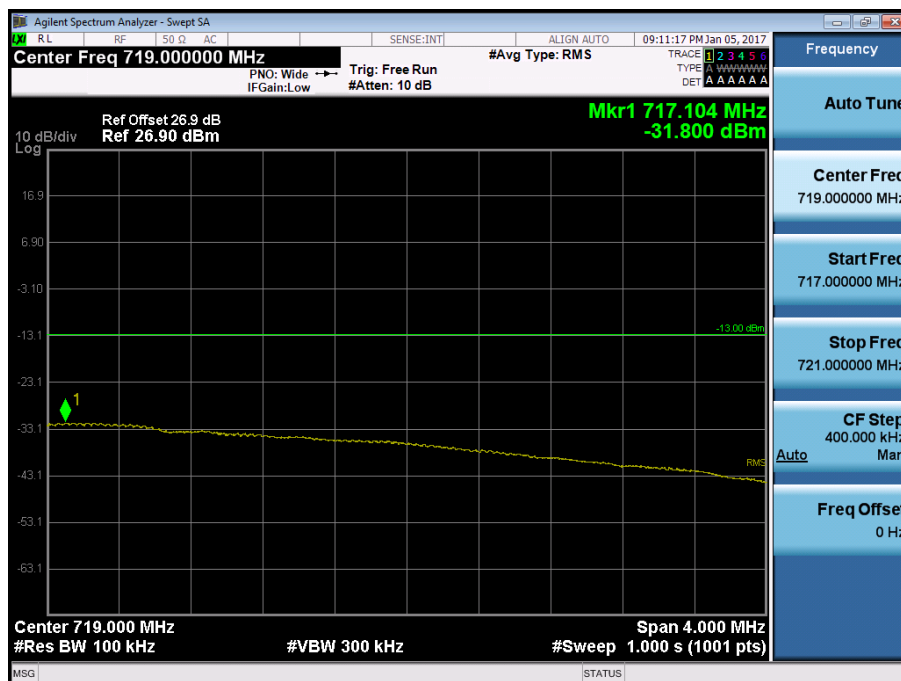
BAND 12 / 17. Upper Extended Band Edge Plot (10M BW Ch.23130 QPSK_RB50_0)
