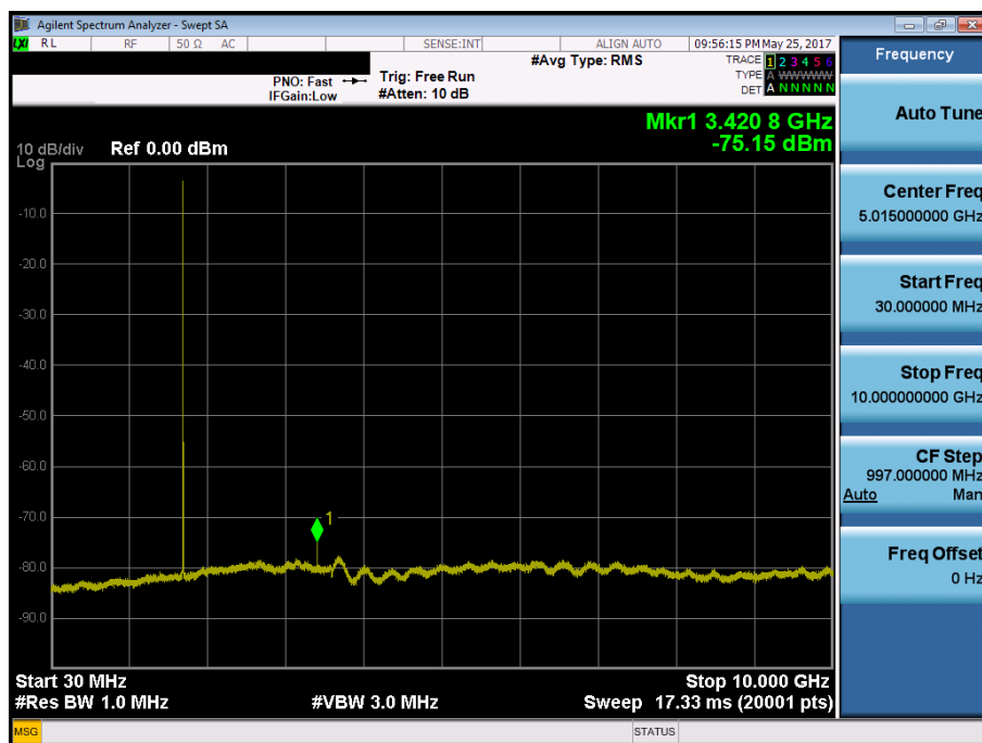
BAND 66. Conducted Spurious Plot_1 (131979ch_1.4MHz_QPSK_RB 1_0)
