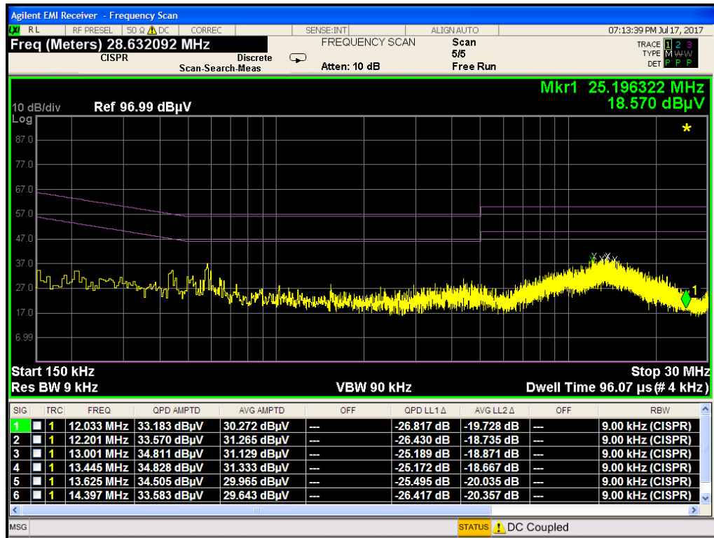
Plot 7-3. Line-Conducted Test Plot with NFC antenna terminated (L1)
