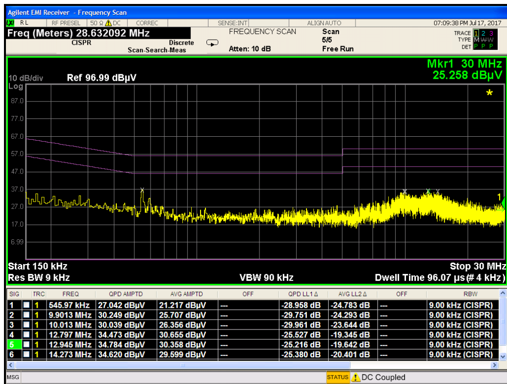
Plot 7-4. Line-Conducted Test Plot with NFC antenna terminated (N)
