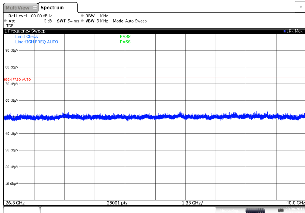
Plot 7-86. Radiated Spurious Plot above 26.5GHz - 40GHz (802.11a – Ant. Pol. V)
