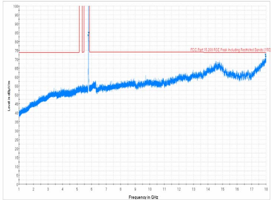
Plot 7-81. Radiated Spurious Plot above 1GHz (802.11a – U3 Ch. 157, Ant. Pol. H)
