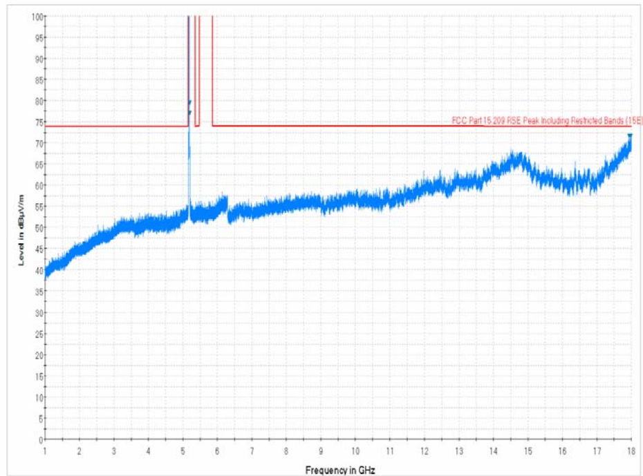
Plot 7-76. Radiated Spurious Plot above 1GHz (802.11a – U1 Ch. 40, Ant. Pol. V)
