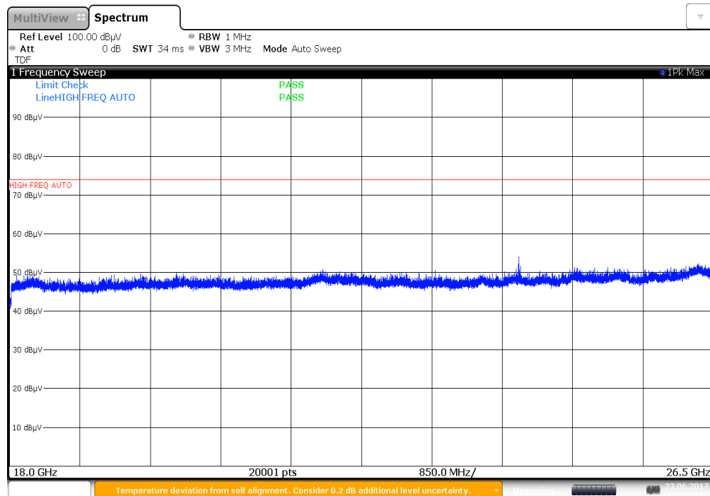
Plot 7-84. Radiated Spurious Plot above 18GHz - 26.5GHz (802.11a – Ant. Pol. V)
