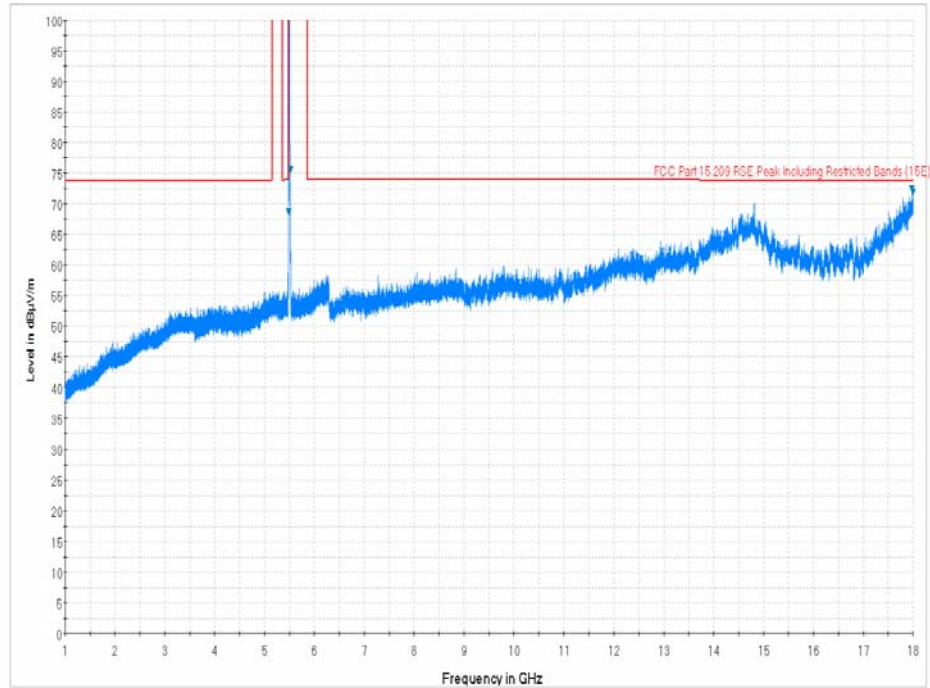
Plot 7-79. Radiated Spurious Plot above 1GHz (802.11a – U2C Ch. 116, Ant. Pol. H)
