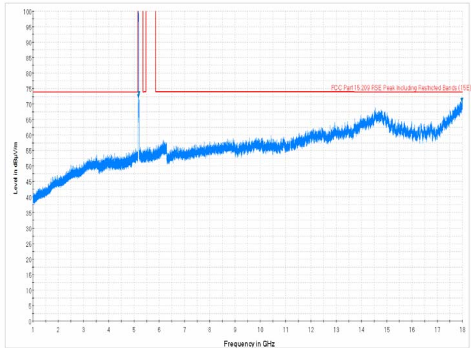
Plot 7-75. Radiated Spurious Plot above 1GHz (802.11a – U1 Ch. 40, Ant. Pol. H)
