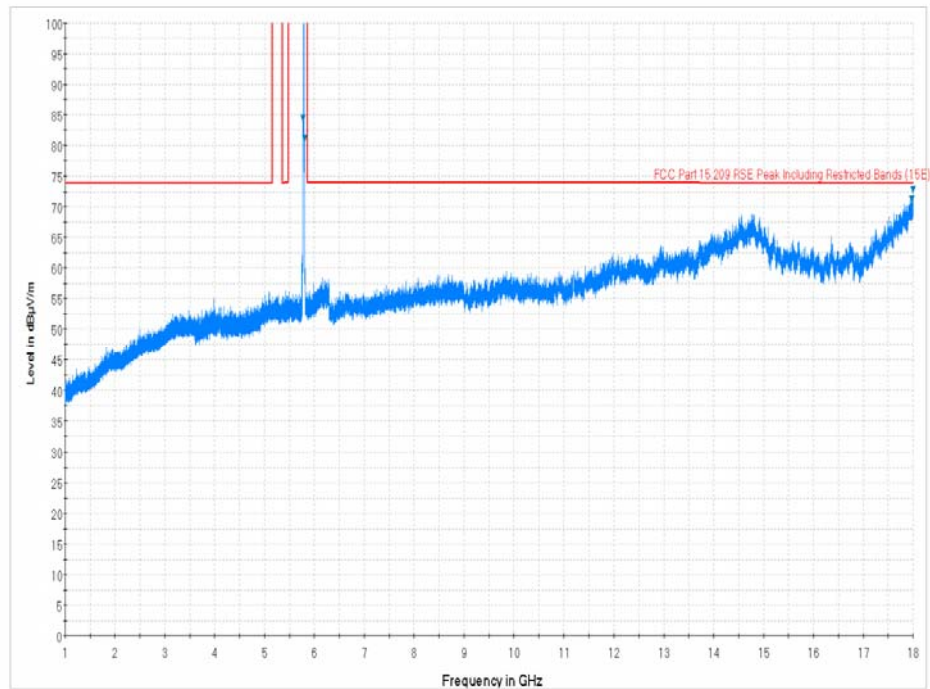
Plot 7-82. Radiated Spurious Plot above 1GHz (802.11a – U3 Ch. 157, Ant. Pol. V)
