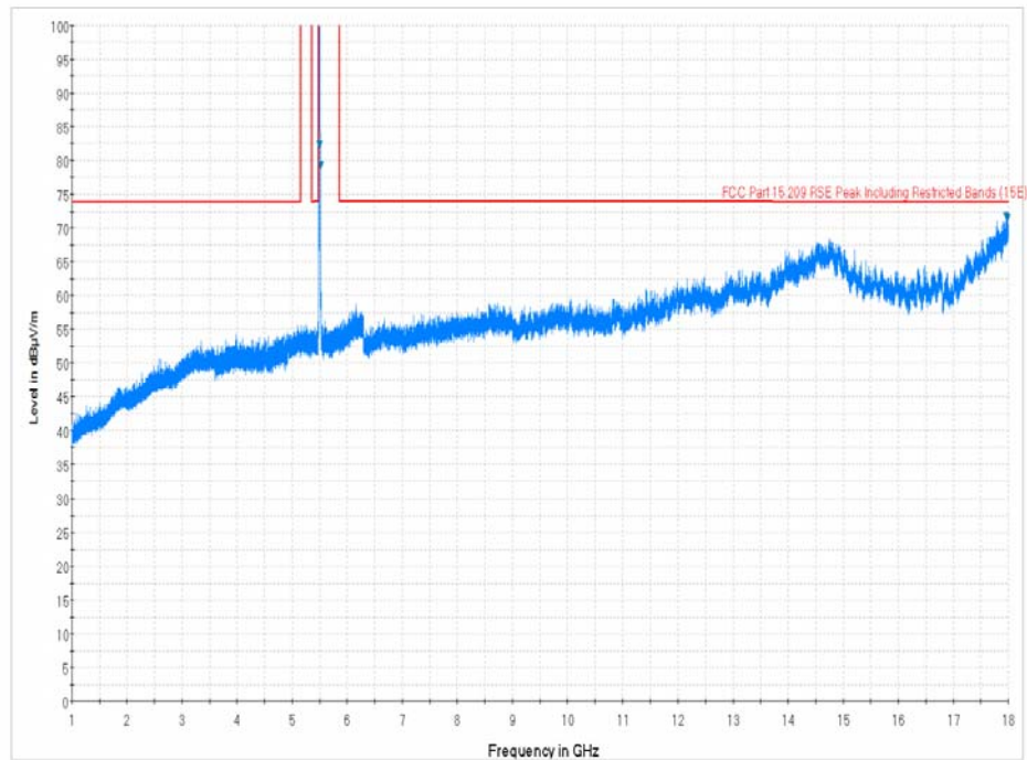
Plot 7-80. Radiated Spurious Plot above 1GHz (802.11a – U2C Ch. 116, Ant. Pol. V)
