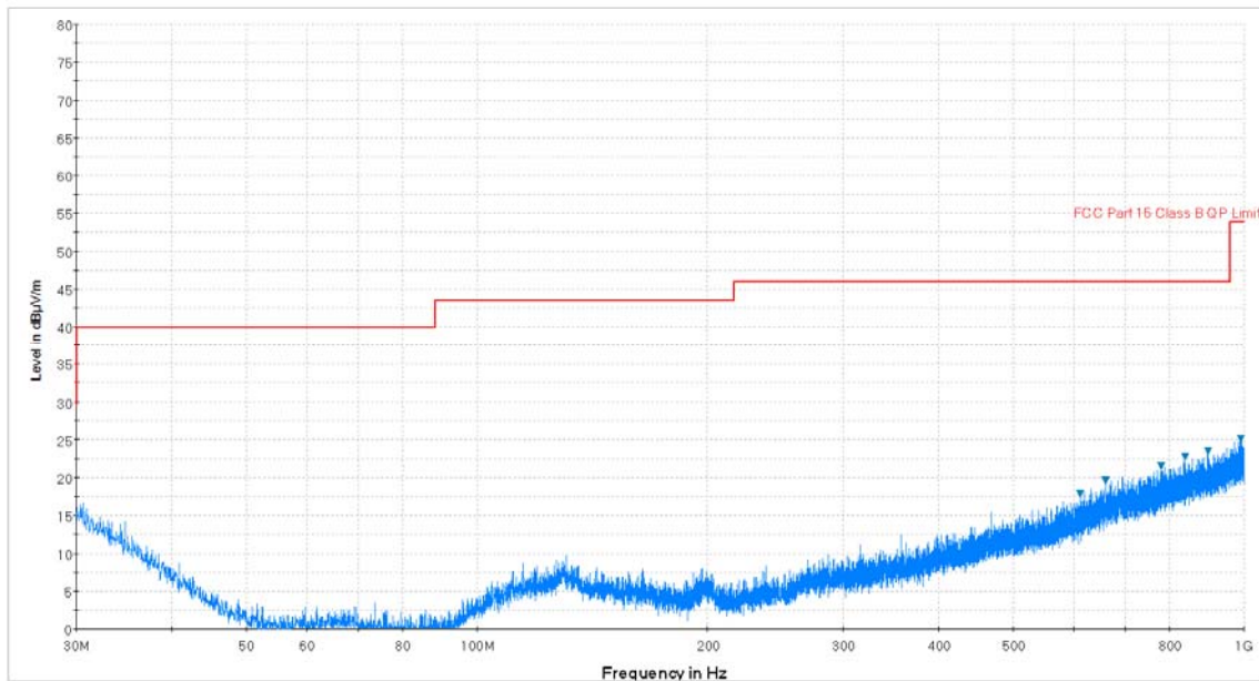
Plot 7-105. Radiated Spurious Plot below 1GHz (802.11a – U3 Ch. 157, Ant. Pol. V)
