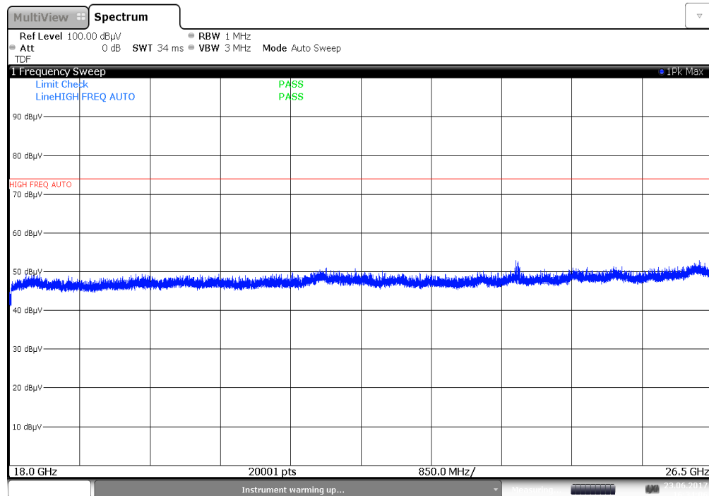
Plot 7-83. Radiated Spurious Plot 18GHz - 26.5GHz (802.11a – Ant. Pol. H)
