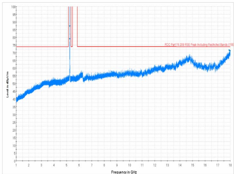
Plot 7-78. Radiated Spurious Plot above 1GHz (802.11a – U2A Ch. 56, Ant. Pol. V)
