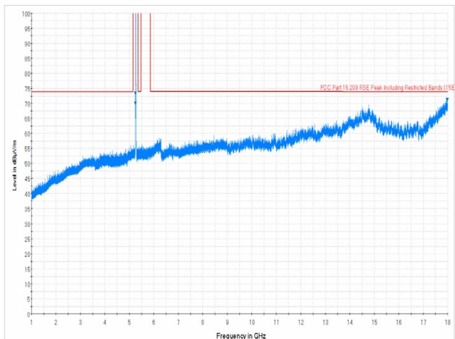
Plot 7-77. Radiated Spurious Plot above 1GHz (802.11a – U2A Ch. 56, Ant. Pol. H)
