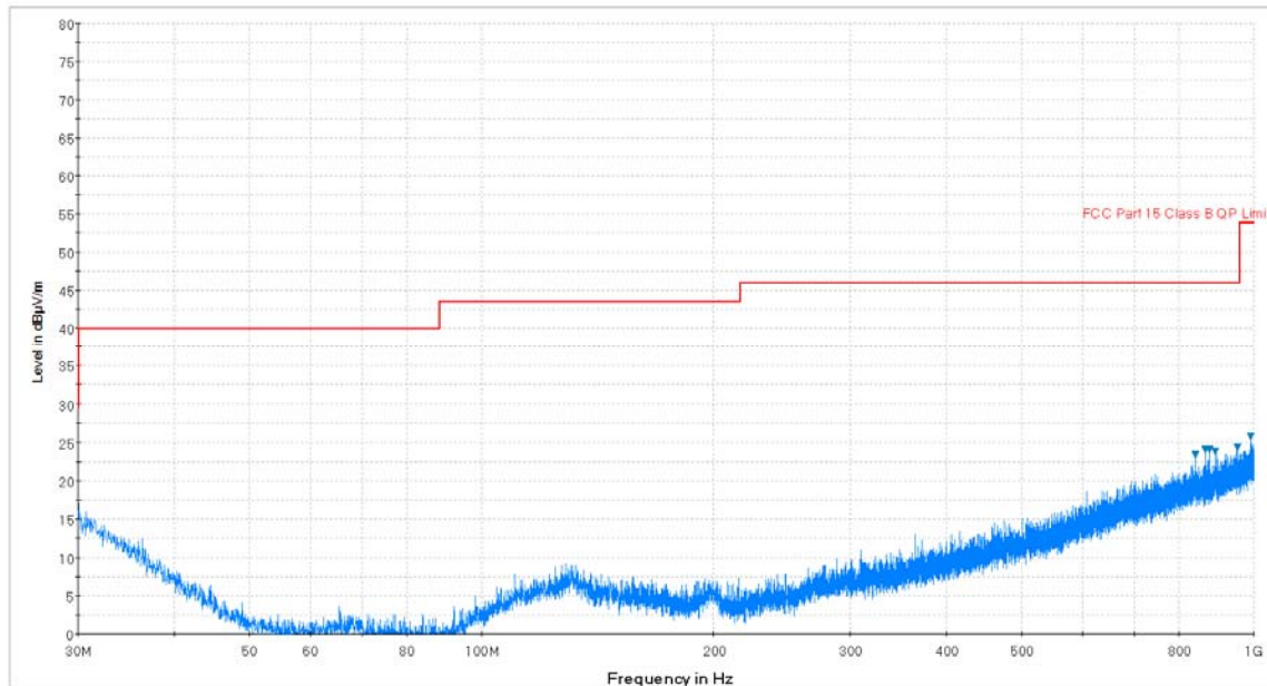
Plot 7-104. Radiated Spurious Plot below 1GHz (802.11a – U3 Ch. 157, Ant. Pol. H)
